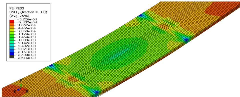
Figure 5.40 Crushing of concrete (Bridge 100-262-1- CR-SS)
