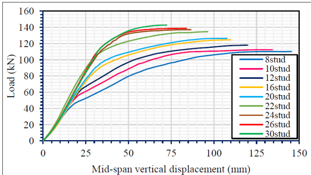
Figure 5.15 Partial interaction effect on the load-deflection relationship of the curved composite beam, redrawn from (A.Jaaffer & L.Kareem, 2020)
