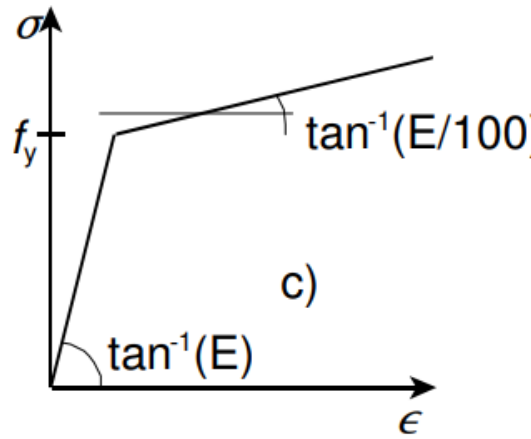
Figure 5.4: Stress-strain relation with strain hardening (EN 1993-1-5, 2005)
