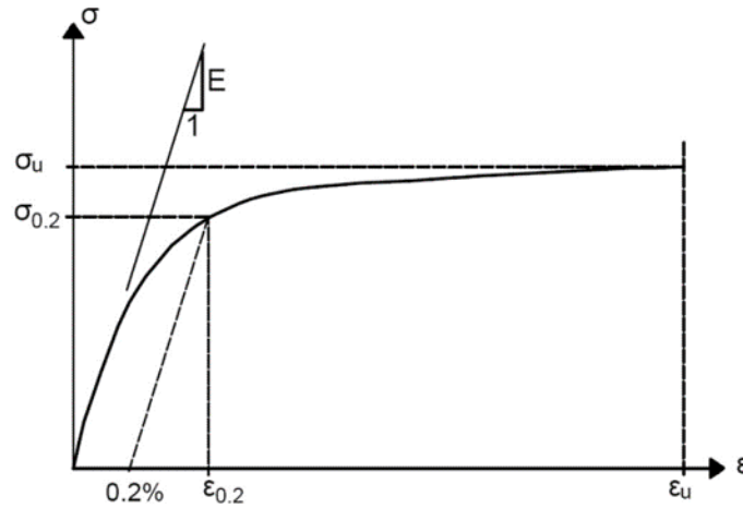
Figure 4.4 Stress-strain relation for stainless steel, from (Shammas & Cashell, 2019)
