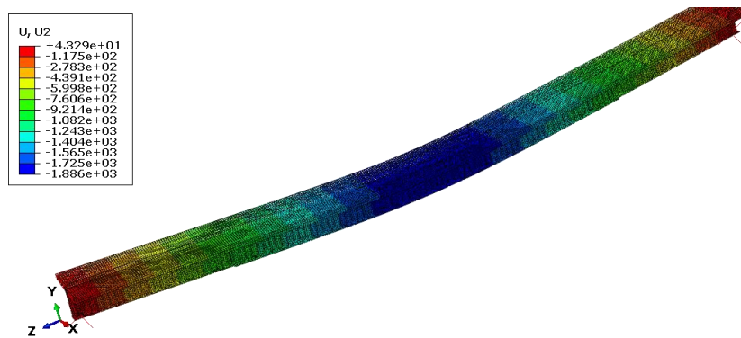
Figure 5.38 Vertical displacement (Bridge 100-262-1- CR-SS)
