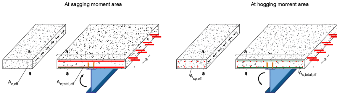
Figure 3.12 Design shear flow at section a-a, redrawn from ( Vayas & Iliopoulos, 2014)
