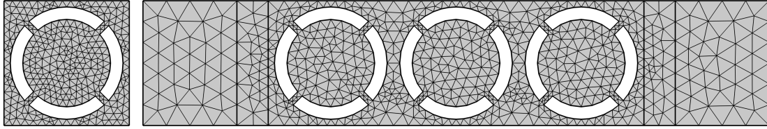
Figure 3.1: Discretized samples for both the unit cell (left) and complete sample (right) with meshing from COMSOL.
