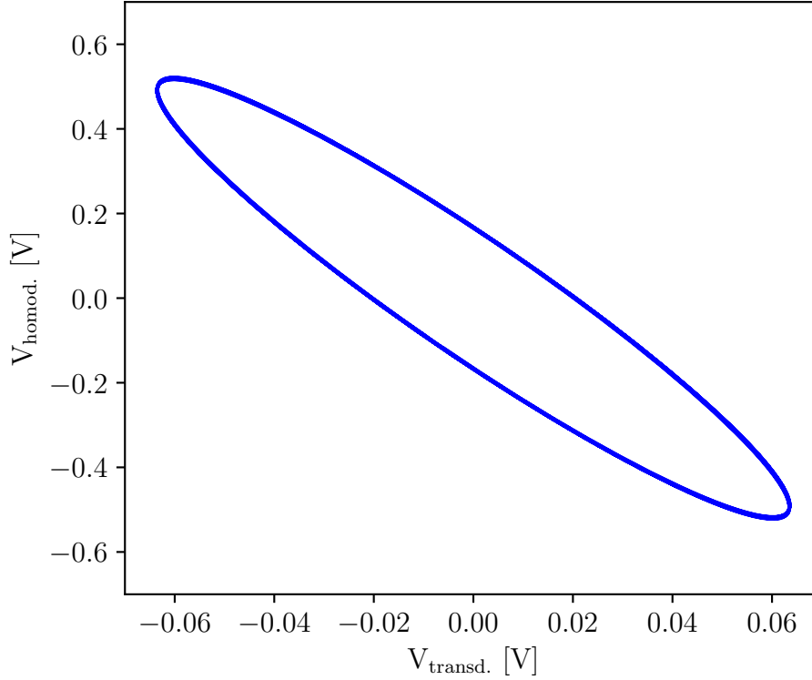
Figure 3.6: Example of a linear calibration measurement where the output voltage of the homodyne is plotted against the input voltage to the transducer. The resulting shape is an ellipse from which the amplitude ratio between the signals can be extracted.
