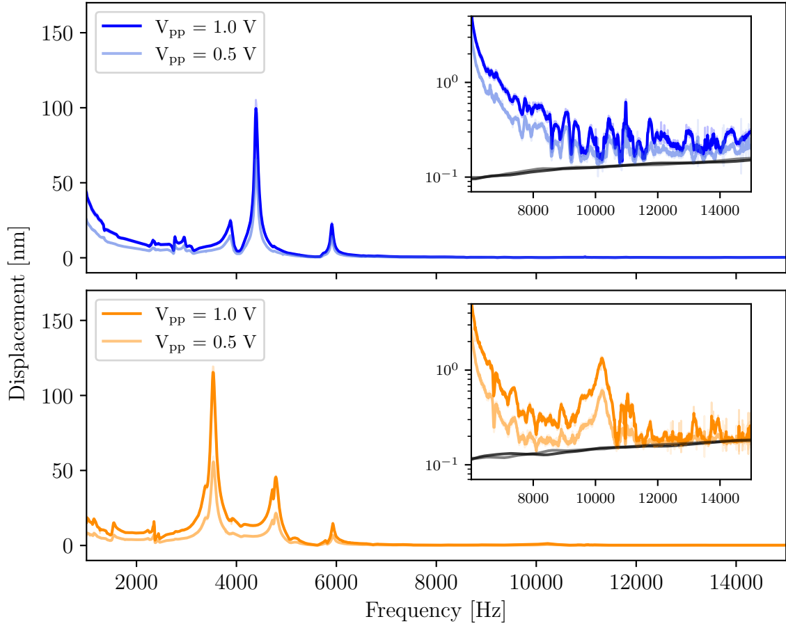
Figure 4.19: Displacements of mirror and bulk sample at frequencies of 1.0–15.0 kHz at input voltages of 0.5 and 1.0 volts. The insets (top right) for each sample shows the log-scaled displacement at higher frequencies.
