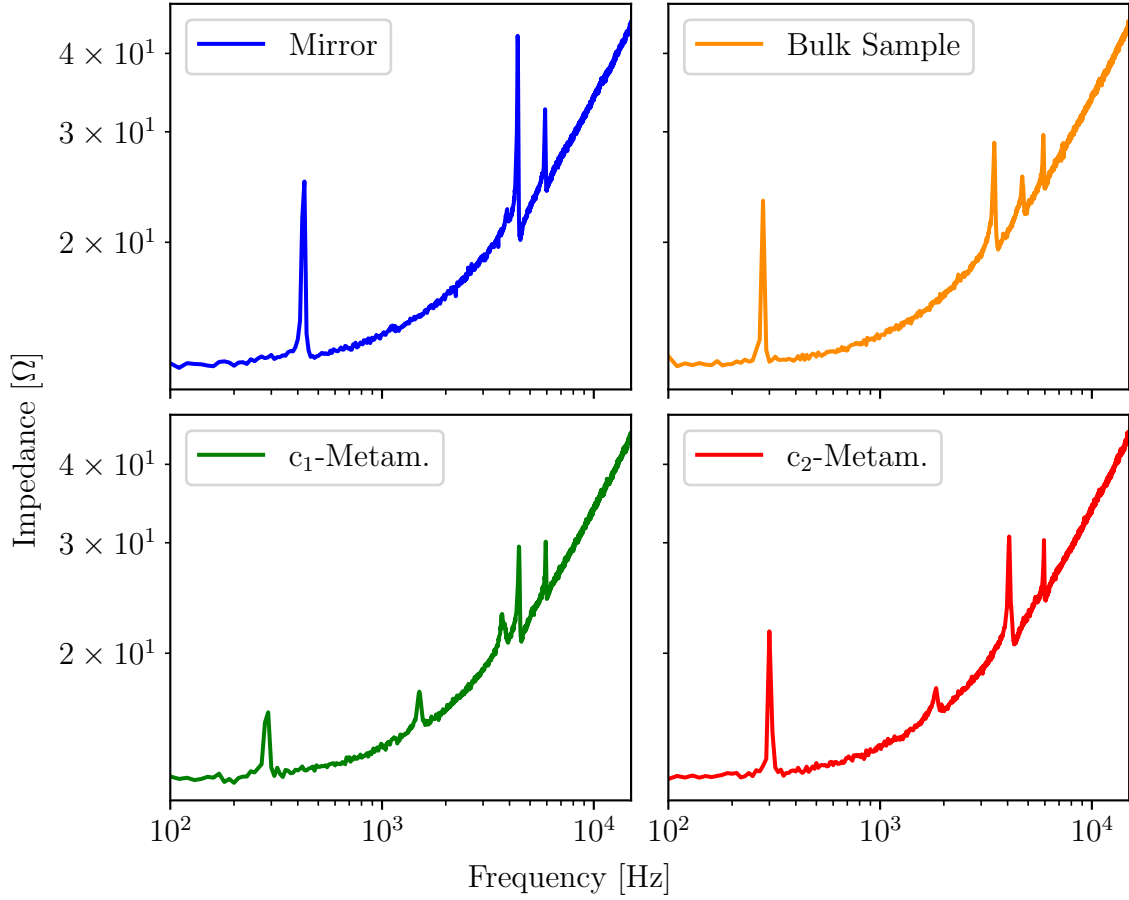
Figure 4.15: Transducer impedance as a function of frequency for each of the four studied samples, with the mirror (top left), bulk sample (top right), c_1 - (bottom left) and c_2 -metamaterials (bottom right). Multiple peaks can be observed corresponding to resonance frequencies of the transducer for each respective load.
