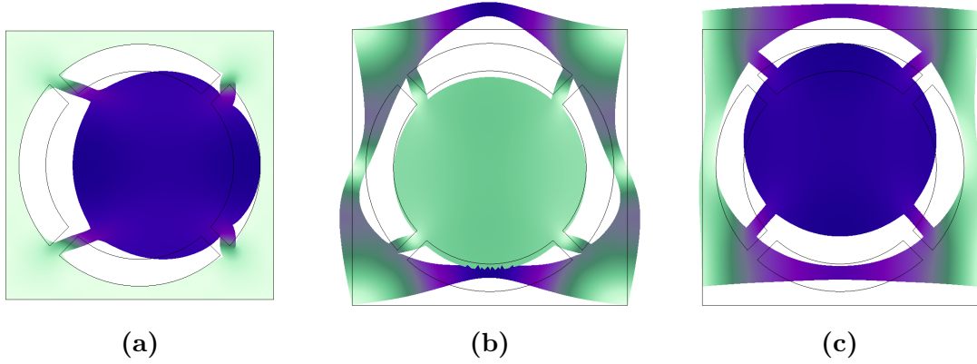
Figure 4.8: Vibrational modes of the unit cell for the c_2 -metamaterial, with dark blue indicating a larger motion and green indicating little to zero motion. These modes are taken from three different points in the dispersion relation, with (a) and (b) corresponding to the upper and lower bands of the directional band gap, respectively, at X. In (c) a mode at halfway between \Gamma and X is shown for the first acoustic band.
