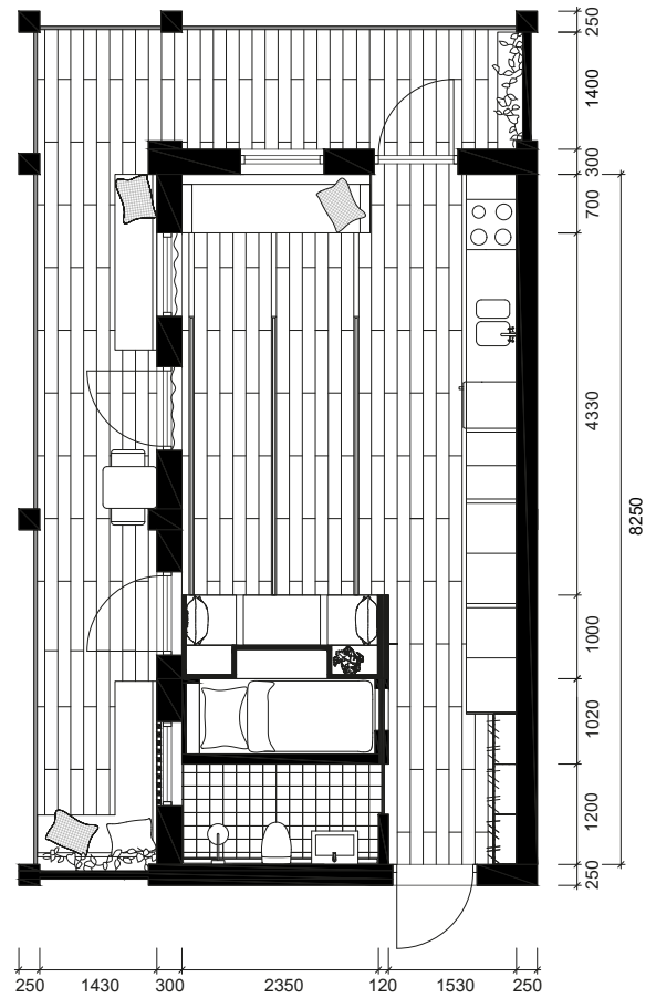
One person household, maximum free space
