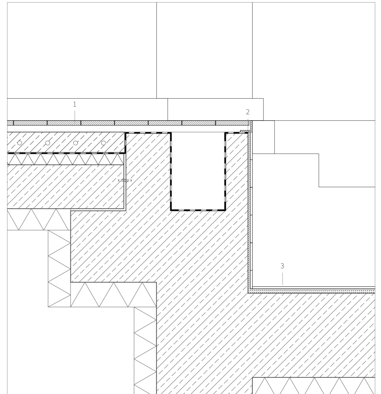
Pool Detail 1:10
