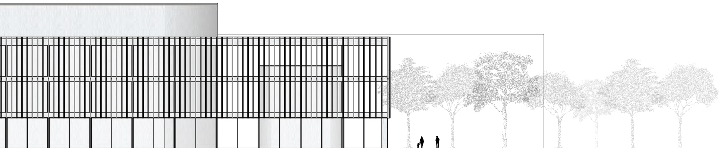
South Elevation 1:400
