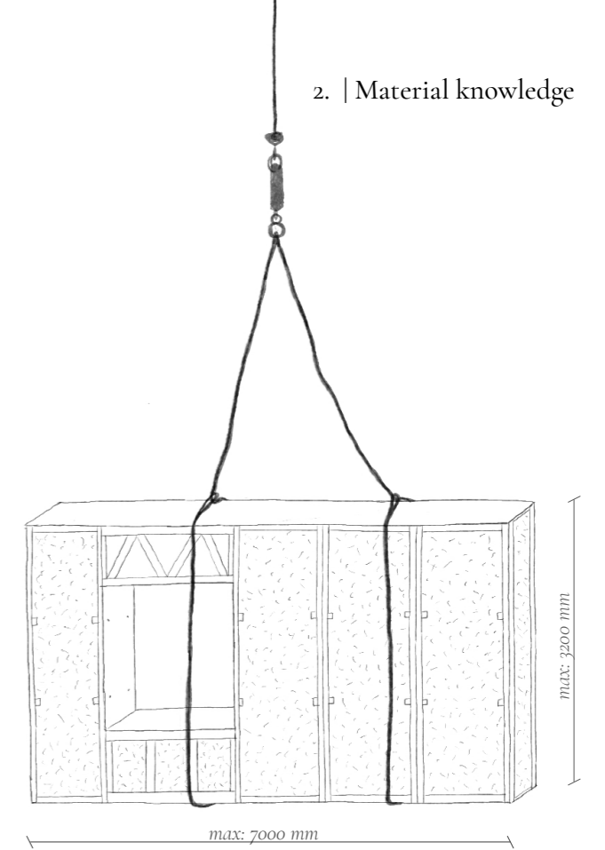
Illustration: Pre-assembled wall element
