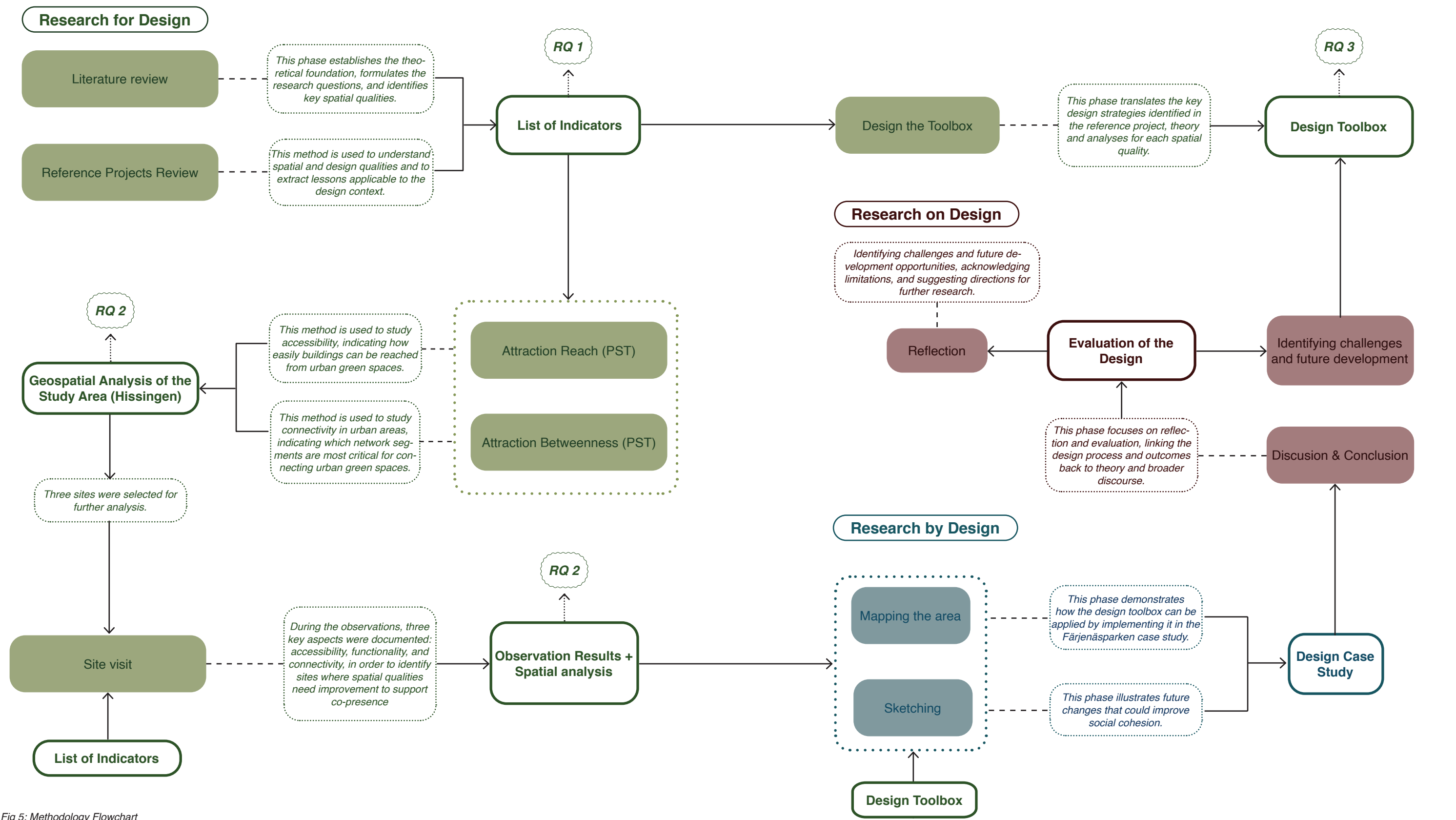
Fig 5: Methodology Flowchart
