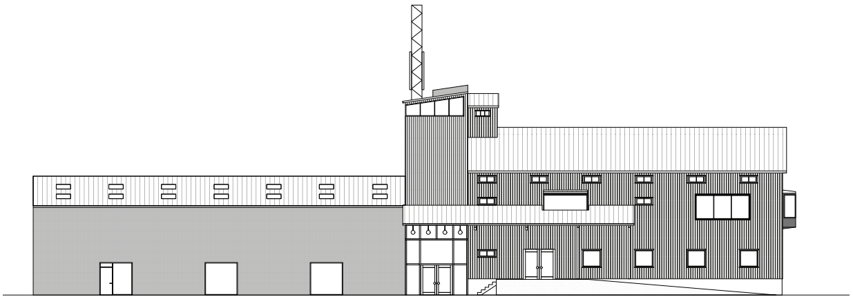
Elevation North-West
