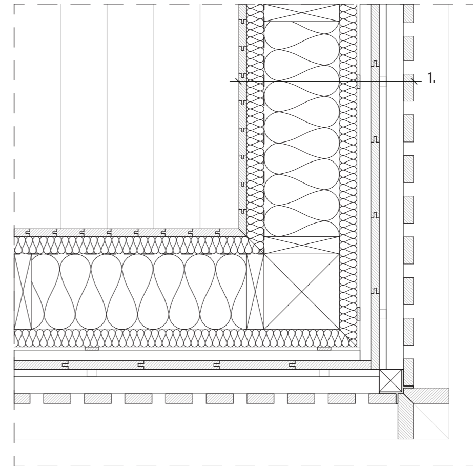
Corner detail Scale 1:10
