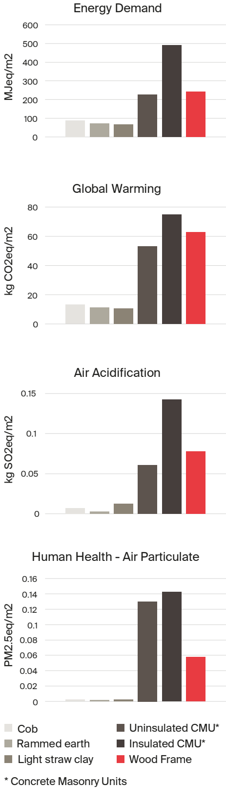
Figure 3. Environmental embodied impacts comparison among different wall systems (adapted from Ben-Alon et al., 2019).
