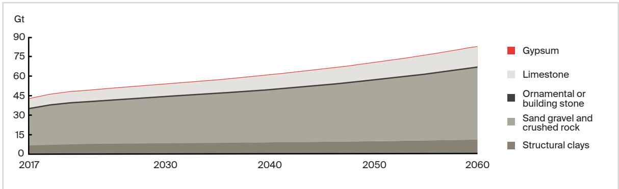
Figure 2. Materials' use for materials directly entering construction in Gt (adapted from OECD, 2019).
