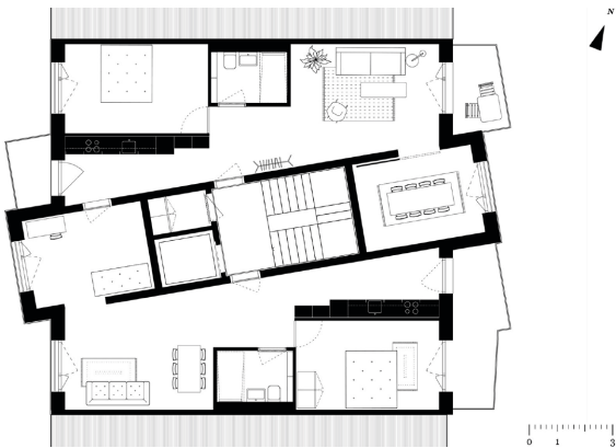
Figure 26. Typical floor plan. Image courtesy of NEUME.
