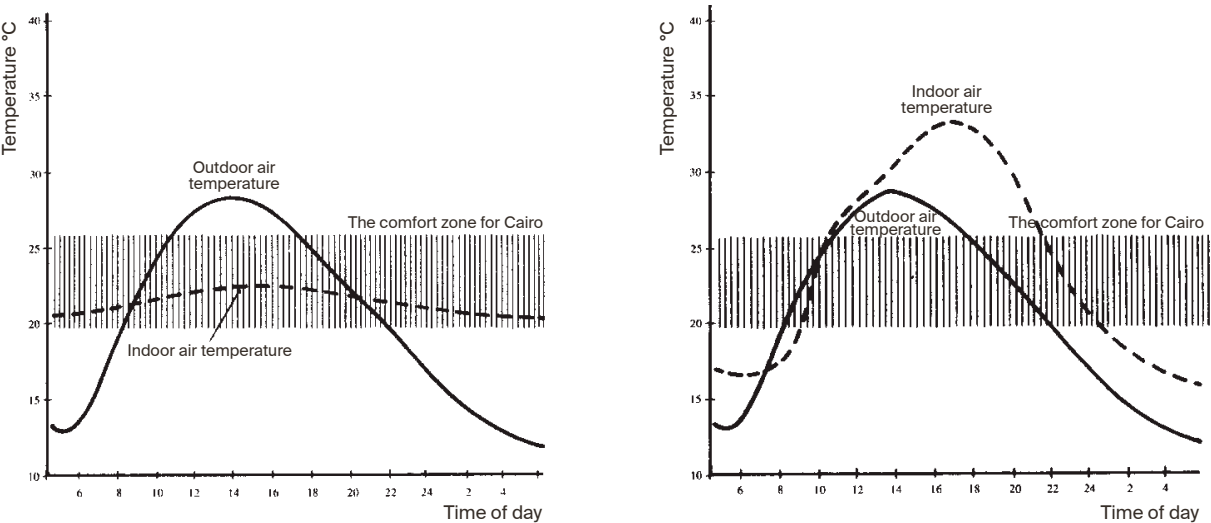
Figure 15. Diurnal variation of indoor and outdoor temperatures in two buildings of equal volume in Egypt: one with 50 cm-thick earth walls and mud brick vaults (left), the other with 10 cm-thick pre-cast concrete elements and a flat roof (right) (originally from Fathy (1986), as reproduced in Minke (2012, p. 30).
