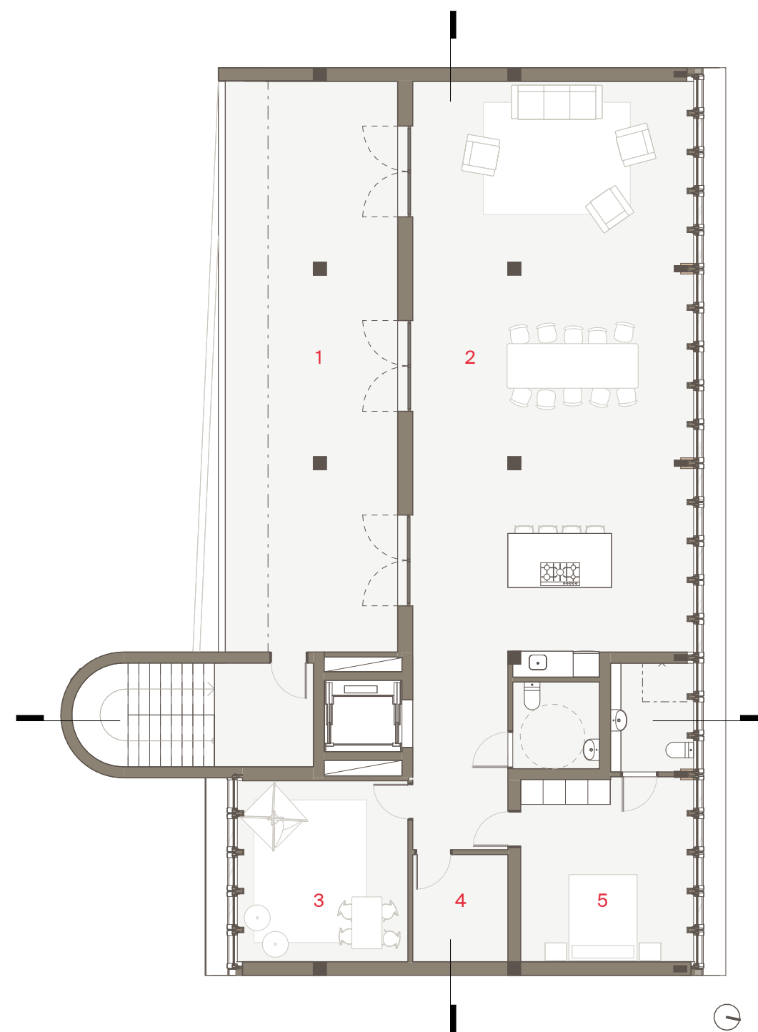
Fourth floor 1:125
