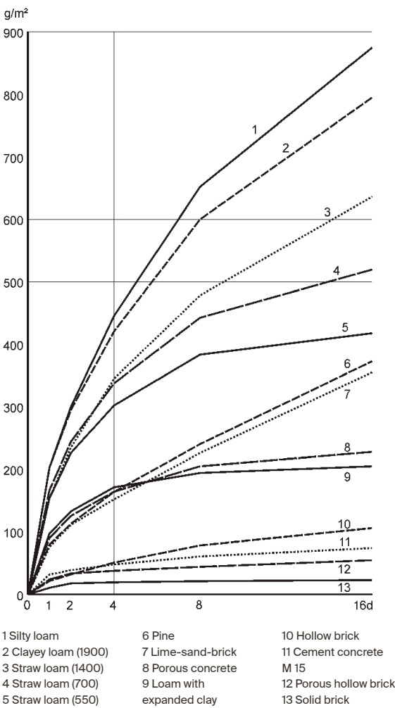
Figure 14. Absorption curves of 11.5 cm-thick interior walls with both sides exposed at 21°C after an abrupt rise in humidity from 50 to 80% (Minke, 2012)
