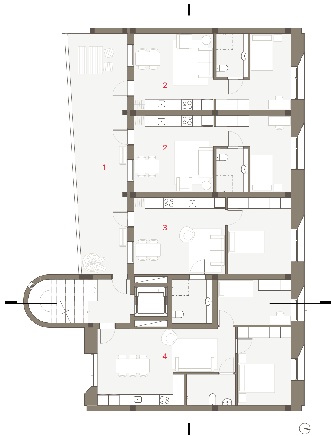
First floor 1:125
