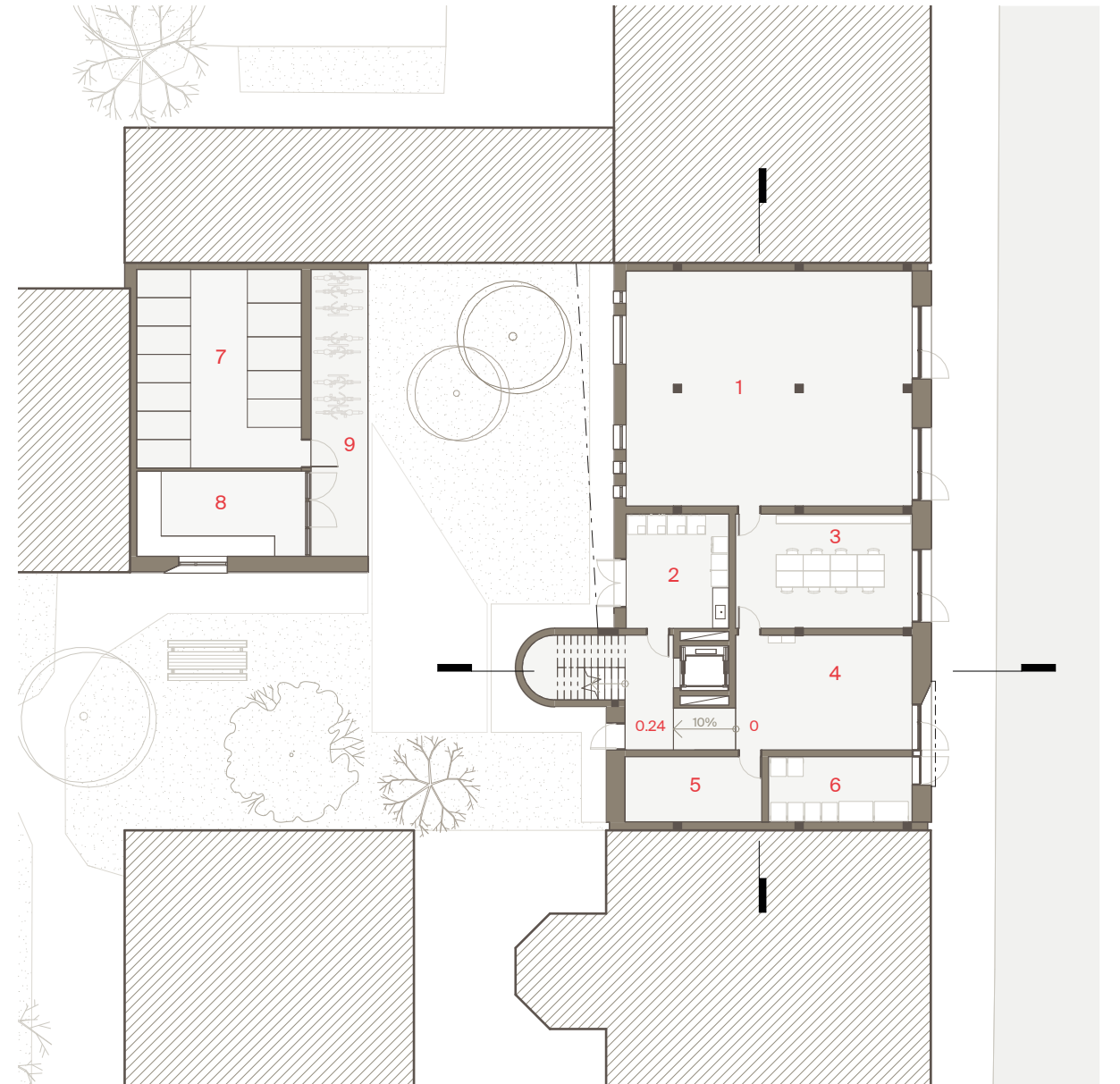
Groundfloor plan 1:250
