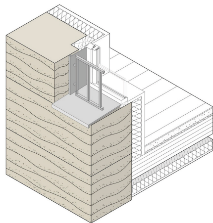
Figure 29. Detail axonometry of prefabricated rammed earth wall. Image courtesy of Déchelette Architecture.
