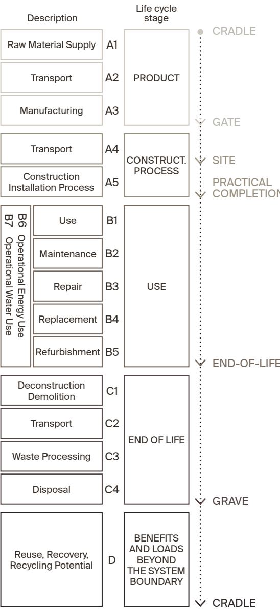
Figure 20. Building's LCA stages according to EN 15978, elaborated by the author.
