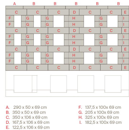
Figure 41. Diagram for the different types of prefabricated rammed earth panels with respective dimensions - street facade elevation
