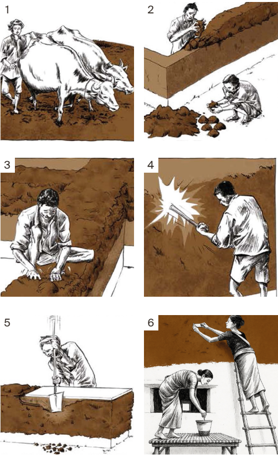
(1) The earth mixture is kneaded into a plastic state (2) It is shaped into small balls by hand (3) The balls are stacked in 50–60 cm layers and pressed together (4) Each layer is tamped to close cracks formed during drying (5) Excess material is trimmed with a shovel and guide board (6) The wall is ready for plastering.
