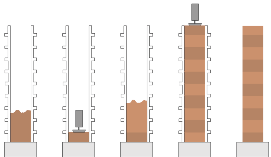
Figure 8. Construction sequence of a rammed earth wall, from layer preparation to formwork removal (adapted from Anysz & Narloch, 2019).
