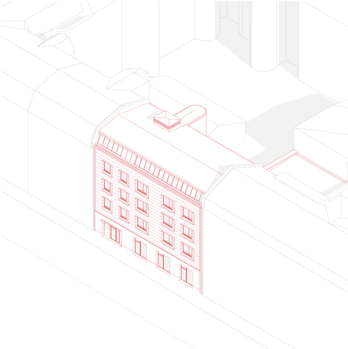
Axonometric view from the street side of the new building
