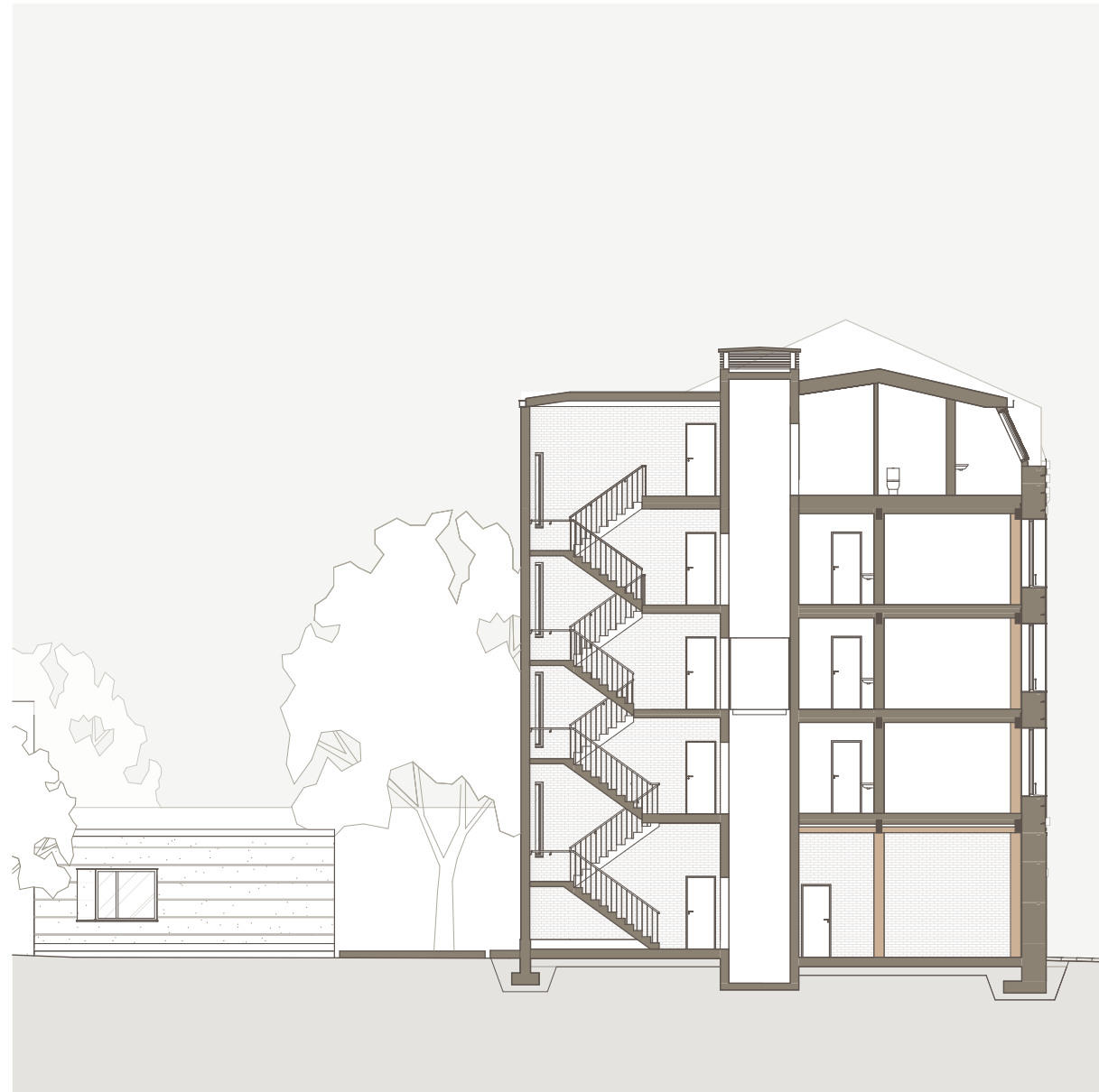
Cross section 1:200
