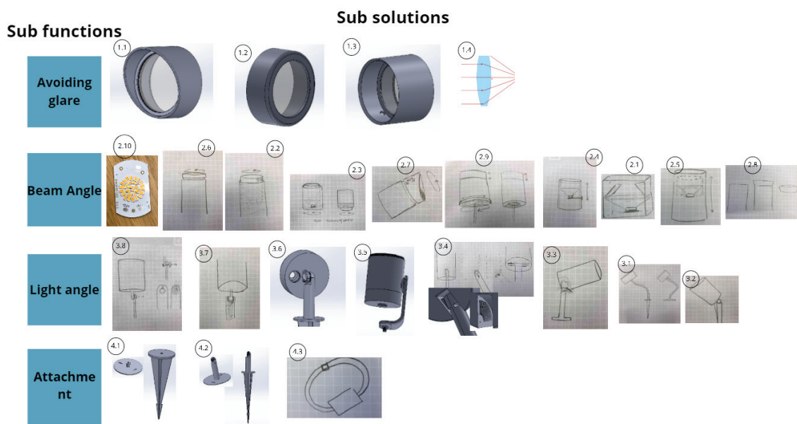
Figure 5.3: Morphological matrix
