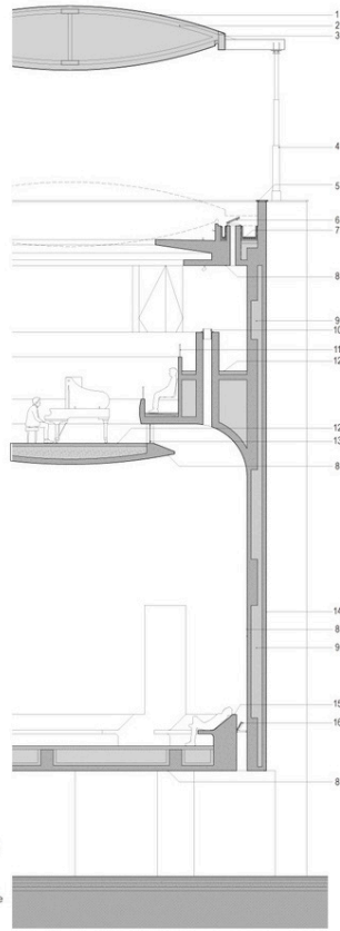
Fig 5. Acoustic detail. Chapel of Music, Vector Architects, 2023
