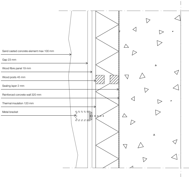
Dark concert hall, wall element Highlighted detail, scale 1:10
