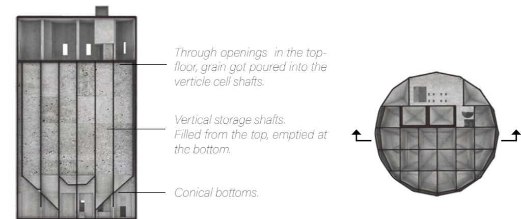
Section of the Quay 240 Grain Silo.
