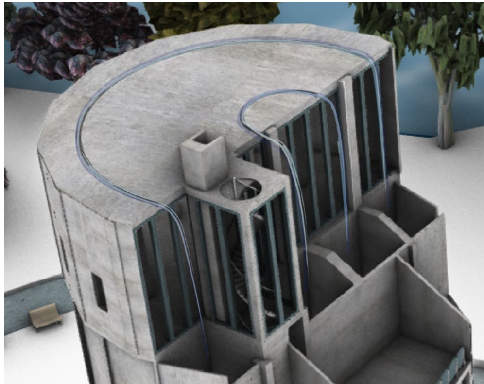
Grooves in the roof collect rainwater and lead it over the edge into open cell shafts.
