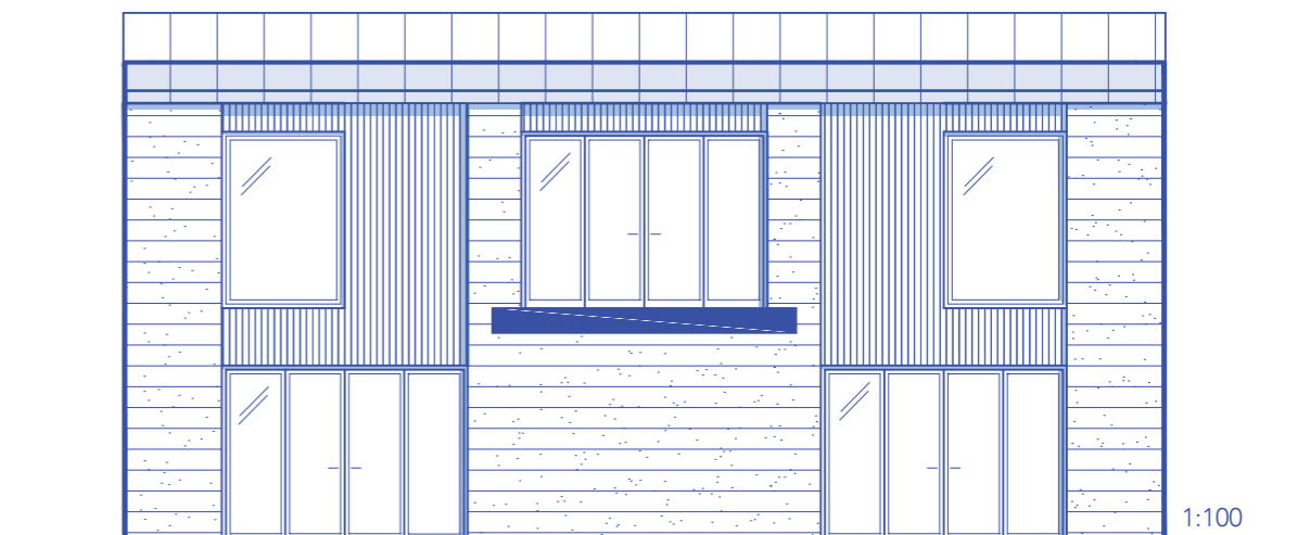
Figure 43. Facade elevation towards the greenhouse, showing the partition of wood and rammed earth sections
