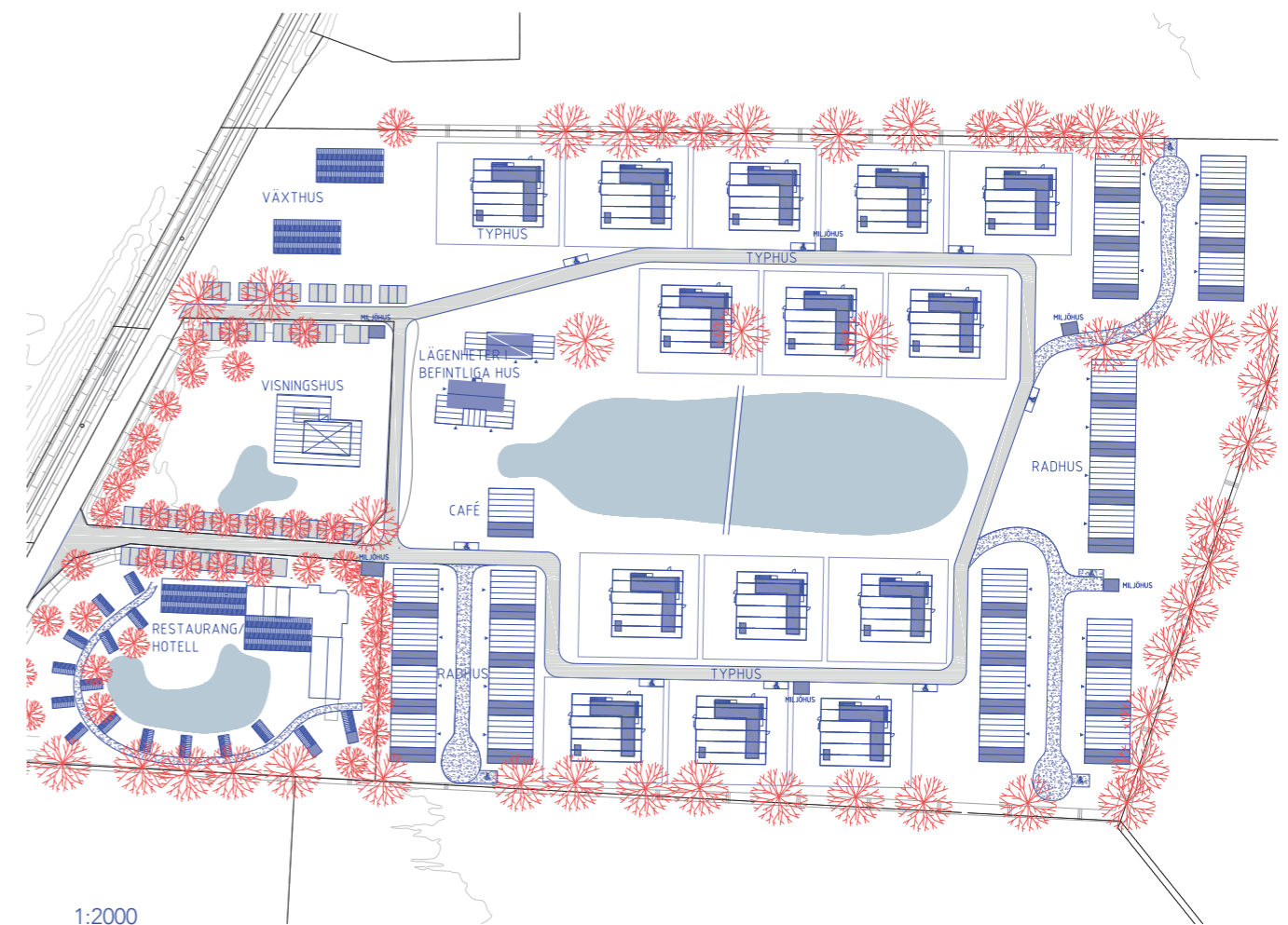
Figure 39. Viadal eco-village site plan, showing rowhouses and villas in combination with greenhouses.
