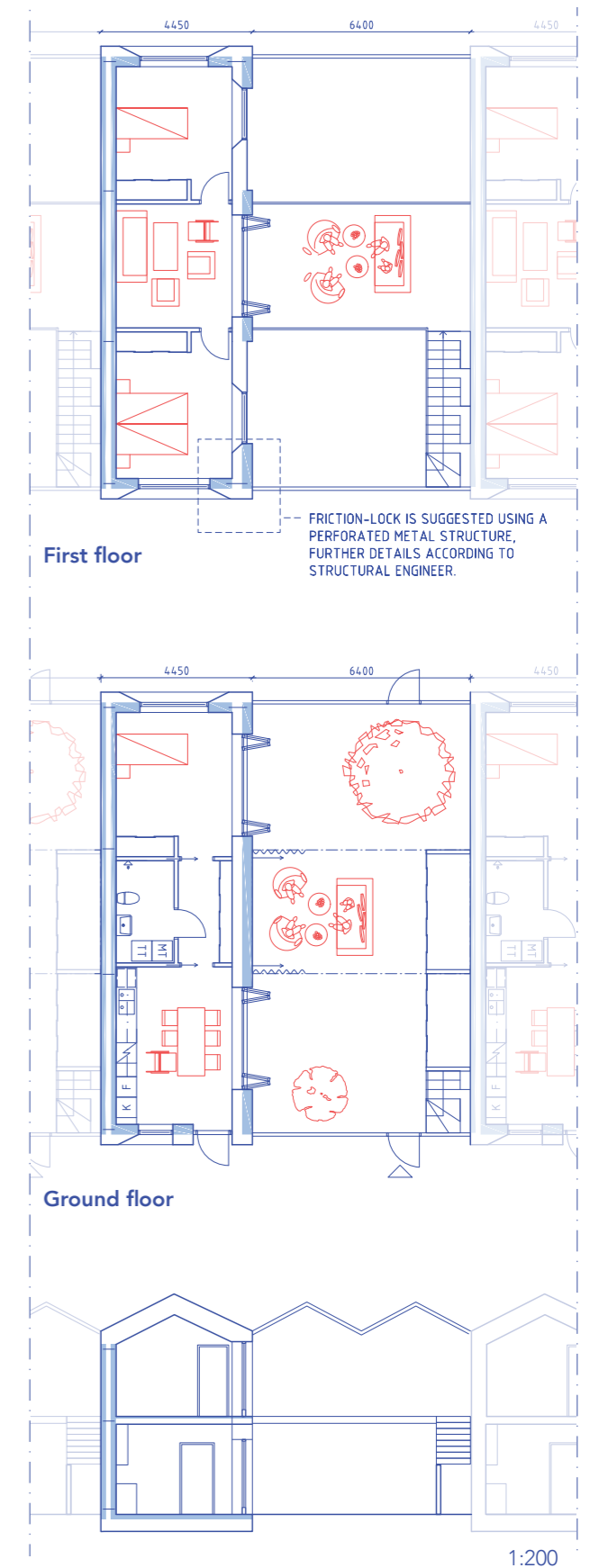
Figure 42. Adapted layout of the rowhouse. Light blue shading shows the placement of the rammed earth.
