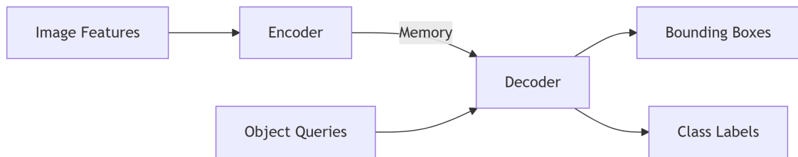
Figure 2.3: Schematic simplified view of DETR
