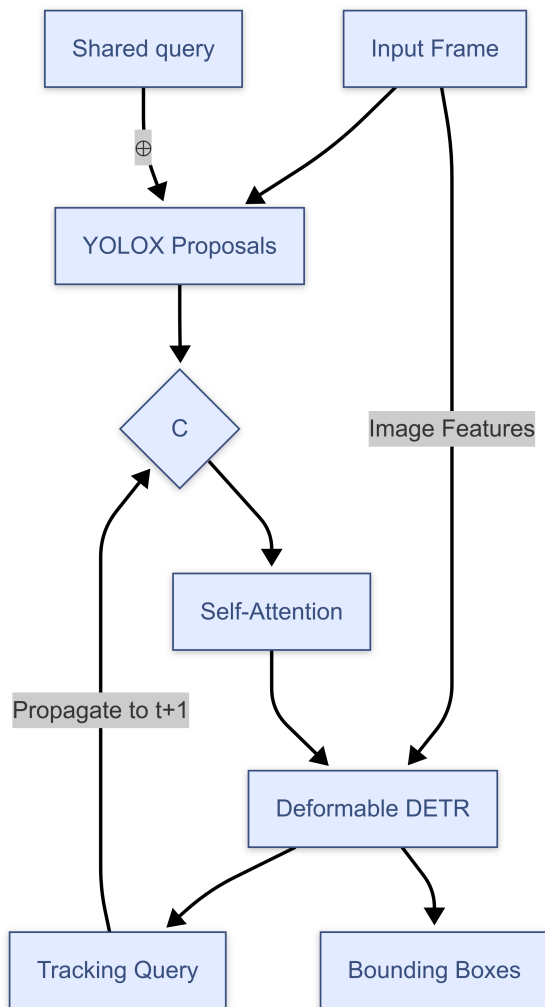
Figure 2.4: Simplified illustration of the MOTRv2 architecture, adapted from original source [2]. Symbols: \oplus denotes addition; C denotes concatenation.
