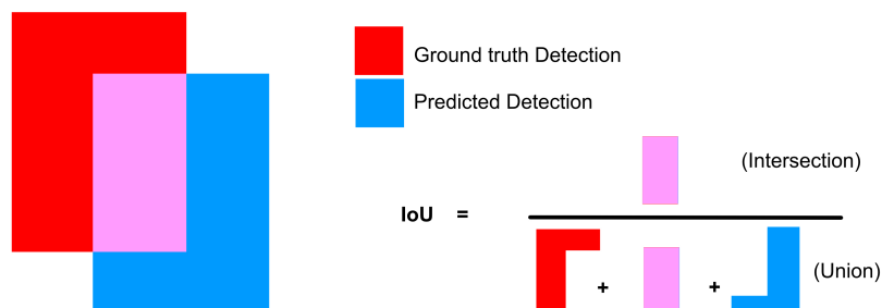
Figure 2.8: Illustration of Intersection over Union (IoU). The blue box is the prediction, the red box is the ground truth, and the shaded pink region represents their intersection.
