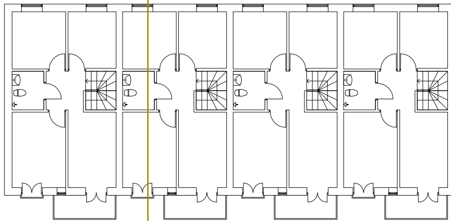
Plans existing house 1:200 (A4).
