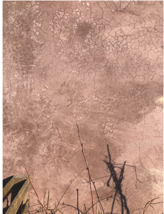
Illustration 6. Image showing cracks in clay plaster facade. Photo: Klara Moene-Omholt.
