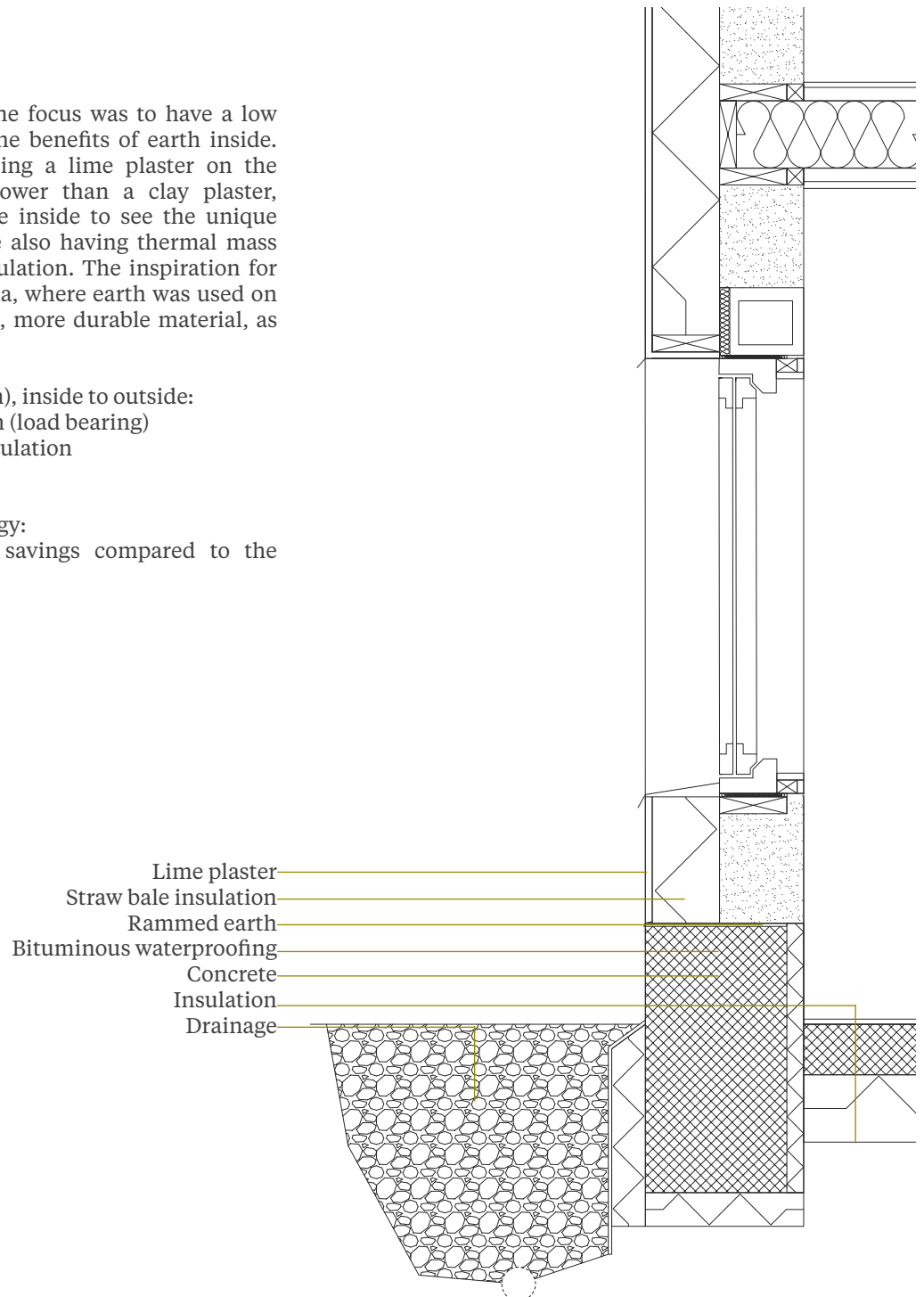
Illustration 41. Detail section 1:20 (A4).
