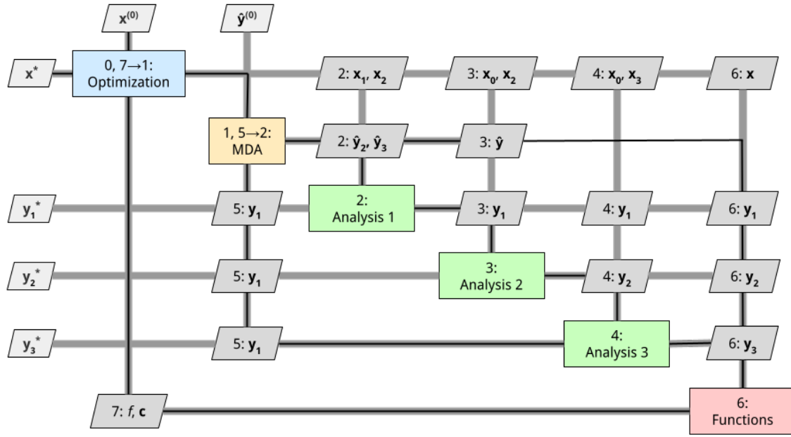
Figure 2.13: Gauss-Seidel multidisciplinary analysis for the MDF architecture [53].
