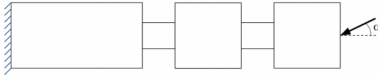
Figure 4.4: Side view of Development Geometry under crash load case P1 . Impact is at an angle \alpha . Boundary conditions are set as fixed in all translations and rotations, the same as for the modal analysis.
