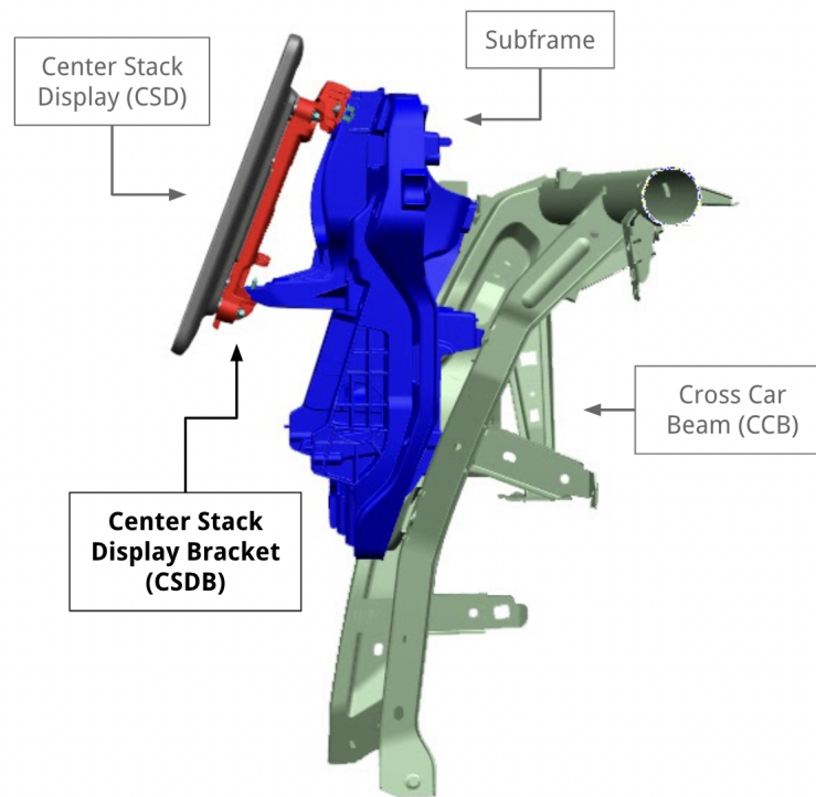
Figure 1.3: Side view of a CSDB and its associated components from a recent VCC model. Note that this is not the exact geometry used in this work.
