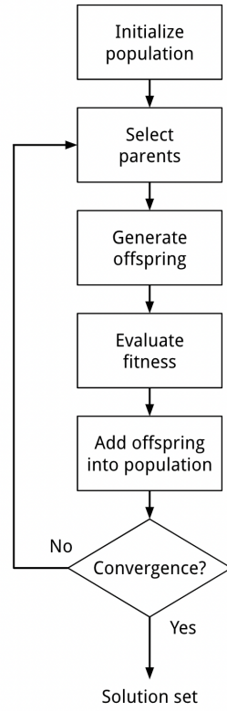
Figure 2.3: A general genetic algorithm process [26].
