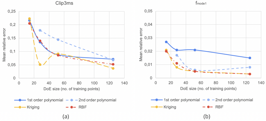
Figure 4.11: Mean relative error as a function of DoE size in clip3ms and f_{model1} for the Development Geometry. 1st and 2nd order polynomial regression, Kriging, and RBF are compared for 3n , 5n , 10n , and 25n with n = 5 and 15-20% validation sets for each respective DoE (excluded in DoE size on x-axis).
