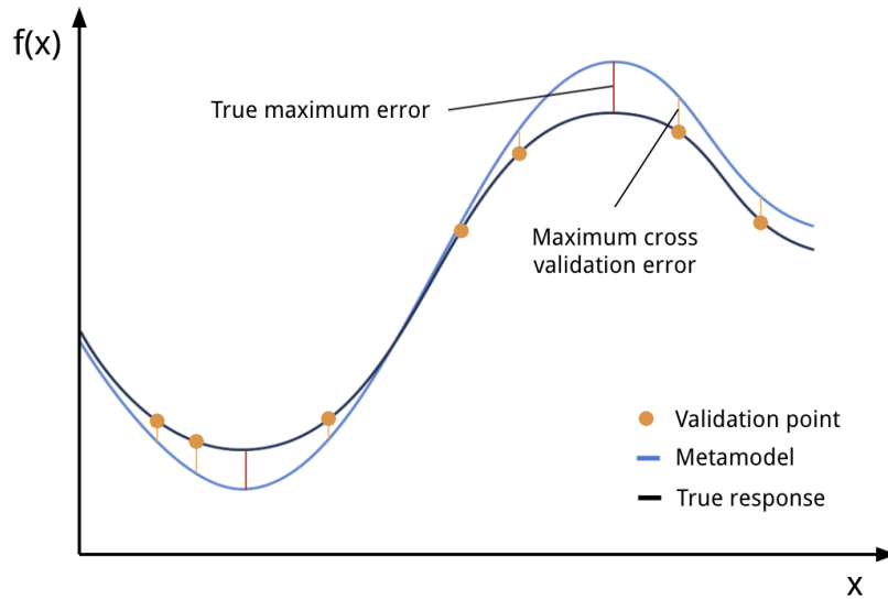
Figure 4.12: Schematic illustration of true maximum metamodel error as compared with maximum simple cross validation error.
