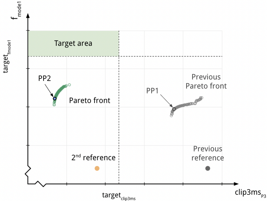
Figure 5.3: Second Pareto front as compared to the previous, see Figure 5.2, after changing DV bounds and fixing a complication with an associated component. Values on axes have been removed for confidentiality.
