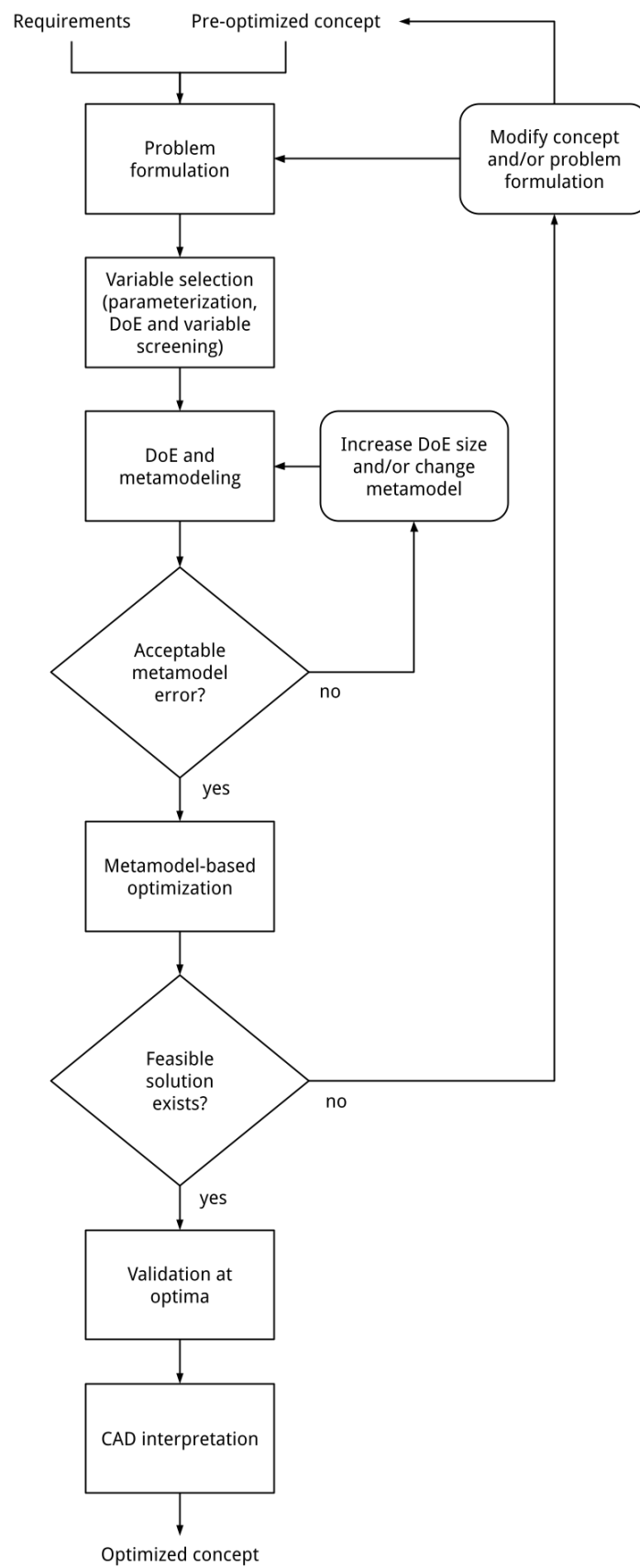
Figure 4.5: Flowchart of the MDO process.
