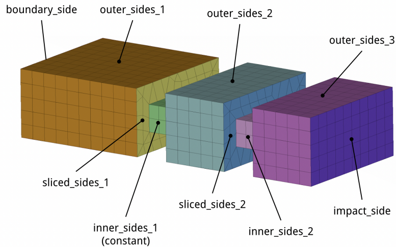
Figure 4.9: Second parameterization of DG, n = 8 . Note that boundary_side, sliced_sides_1, and sliced_sides_2 are completely or partially obscured.
