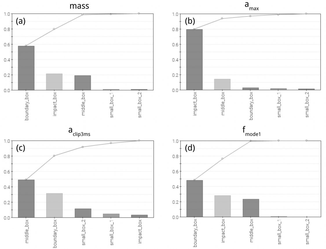
Figure 4.8: Effect bar charts for the first parameterization with four responses: (a) mass, (b) maximum acceleration a_{max} , (c) clip3ms acceleration a_{clip3ms} , and (d) eigenfrequency of the first mode f_{mode1} .
