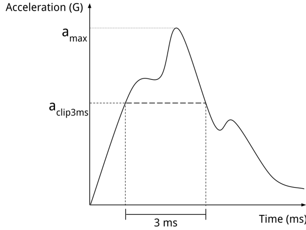
Figure 2.1: Schematic representation of acceleration curve under head impact. Maximum acceleration a_{max} and maximum acceleration under a 3 milliseconds time interval a_{clip3ms} are denoted.
