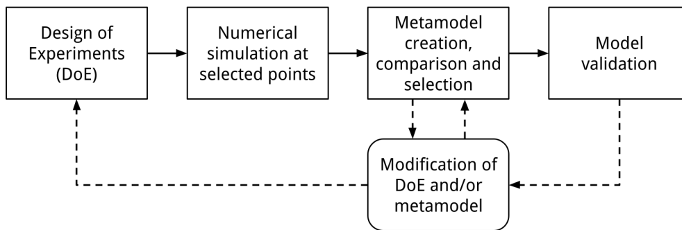
Figure 2.8: Key stages of the metamodeling process, adapted from [42]. Dashed lines indicate steps that may be required if a subprocess arrives at an unsatisfactory result.
