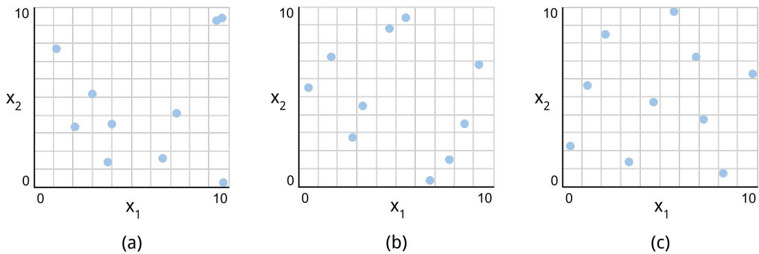
Figure 2.7: Point distribution in a bidimensional space with various sampling algorithms: (a) Simple Monte Carlo sampling; (b) non-space-filling or random Latin Hypercube; (c) space-filling Uniform Latin Hypercube.
