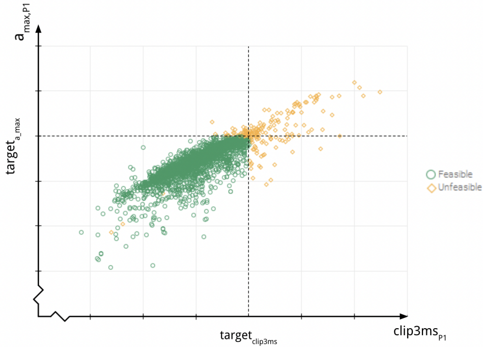
Figure 5.4: MOGA-II crash performance results for second MOO at P1 . Values on axes have been removed for confidentiality.
