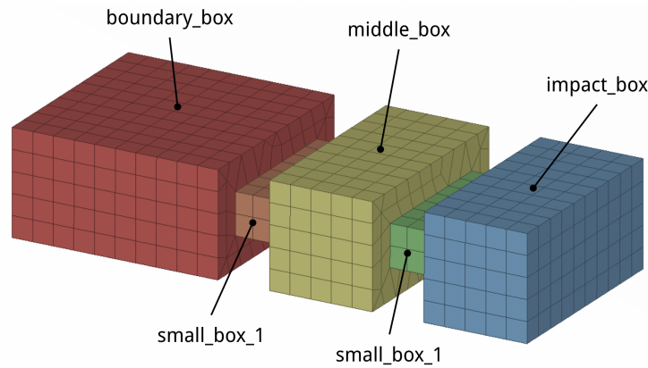
Figure 4.7: First parameterization of DG, n = 5 .
