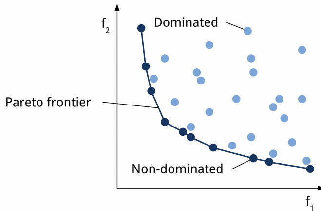
Figure 2.2: Pareto optimality in a min-min problem, i.e., a problem where both objectives are minimized. Points represent evaluations in the design space with the objective functions f_1 and f_2 .
