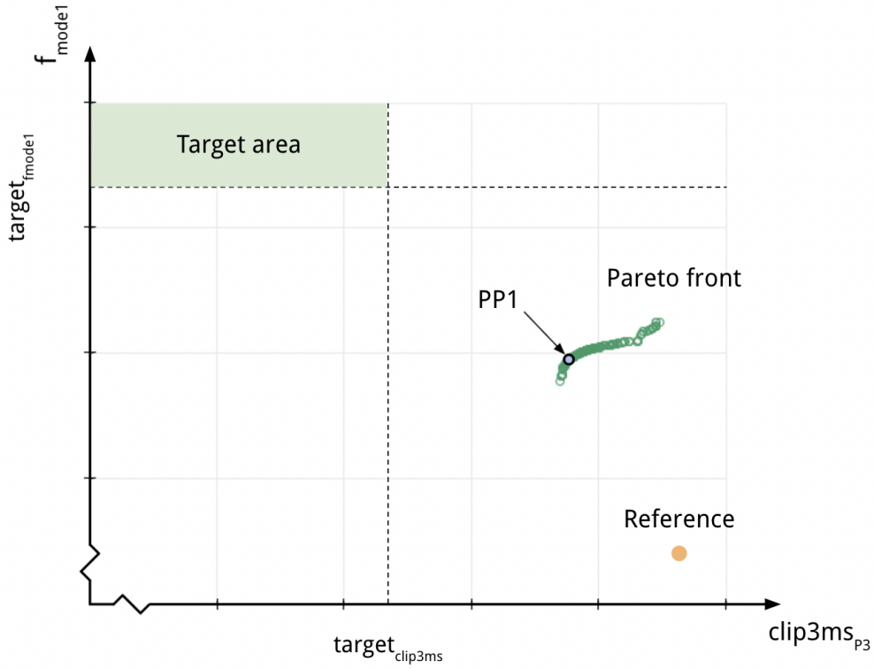
Figure 5.2: Pareto front from metamodels in relation to the reference and the targets on max-min MOO formulation ( f_{model1} is maximized and clip3ms_{P3} is minimized) illustrating the trade-off between clip3ms and modal performance. Values on axes have been removed for confidentiality.
