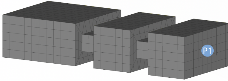
Figure 4.3: Shell mesh of Development Geometry annotated with head impact point P1 .
