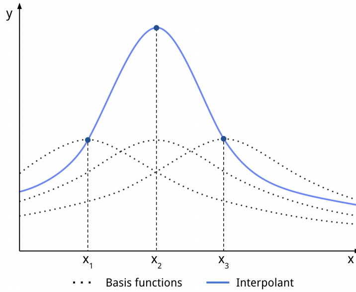
Figure 2.9: RBF interpolation with n = 3 using inverse multiquadrics, adapted from [45].
