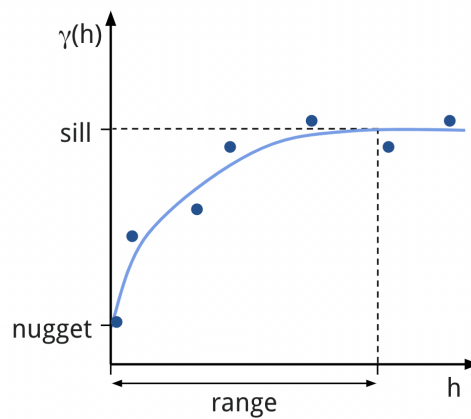
Figure 2.10: Theoretical variogram fitting with spherical model to an experimental variogram with associated notation. Adapted from [51].
