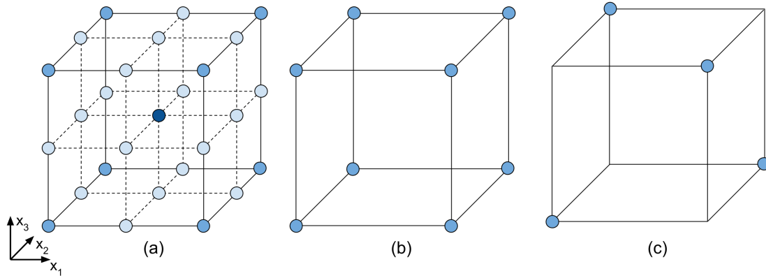
Figure 2.6: Representation of design points in the experimental domain: (a) 3-level, 3-factor full factorial design with 3^3 points; (b) 2-level, 3-factor full factorial design with 2^3 points; (c) 2-level, 3-factor 1/2 fractional factorial design with 2^{3-1} points.
