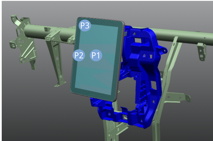
Figure 5.1: Points of head impact on the CSD for load cases P1 , P2 , and P3 .
