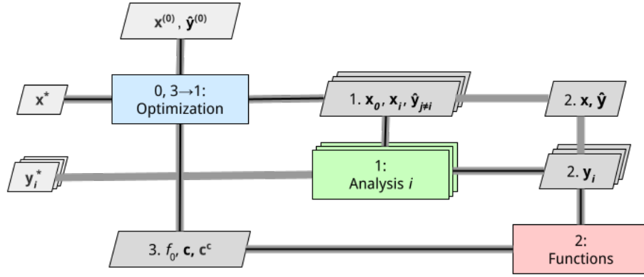
Figure 2.14: Process flow and data dependencies of the IDF architecture [53].
