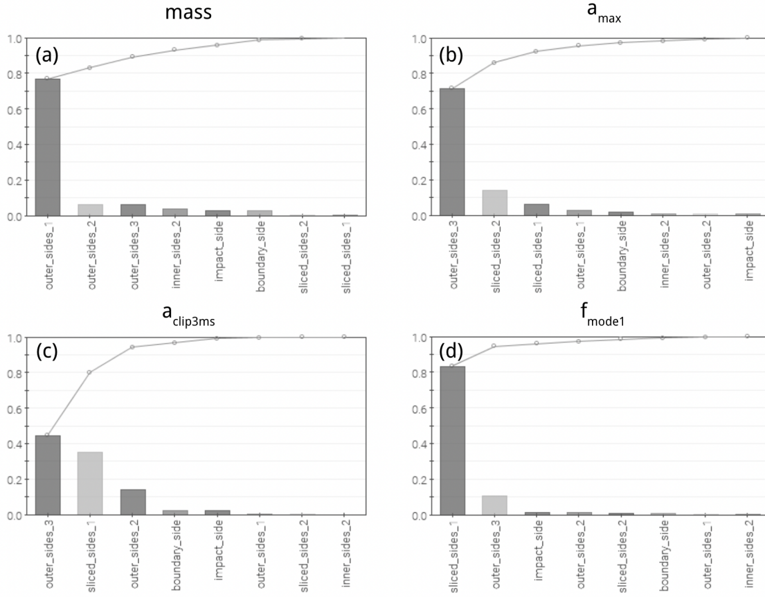
Figure 4.10: Effect bar charts for the second parameterization with four responses: (a) mass, (b) maximum acceleration a_{max} , (c) clip3ms acceleration a_{clip3ms} , and (d) eigenfrequency of the first mode f_{mode1} .
