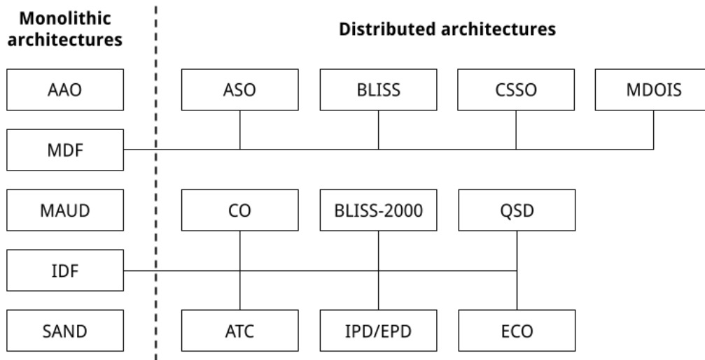
Figure 2.11: A selection of MDO architectures and their categorization.
