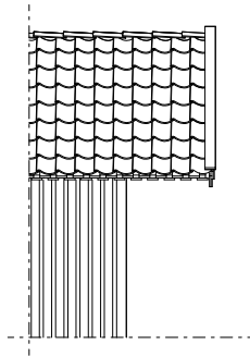
Extended gable | protection
