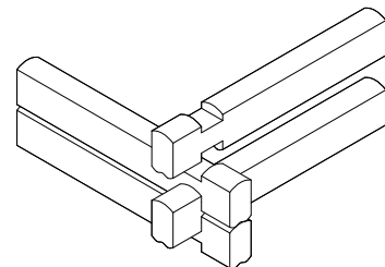
Straight double-notch knot
