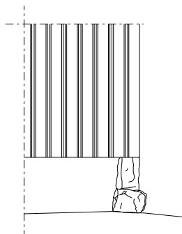
Stone foundation | Meeting with the ground
