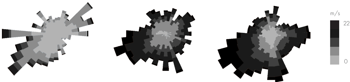
Windroses showing direction and intensity based on data from Svarteberg (left), Måseskär fyr (middle) and Väderöarna (right).
