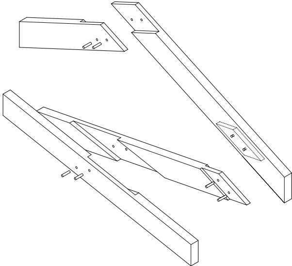
1. Roof truss
