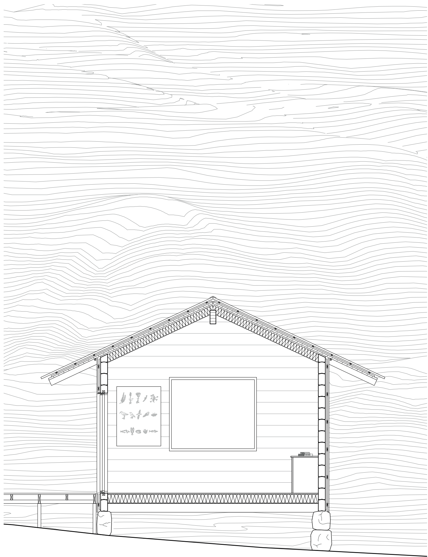
Section C-C
