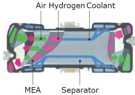
Figure 3.28: Honda clarity PEM fuel cell stack 1
