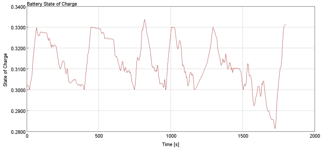
Figure 4.13: Case 2: The initial SOC value is 30.2%, WLTC driving cycle.
