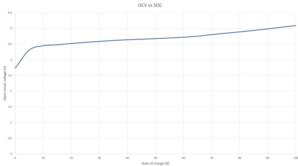
Figure 3.46: HEV battery cell U-I curve
