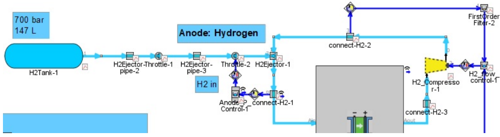
Figure 3.32: Anode reactants supplying system model in GT-Suite
