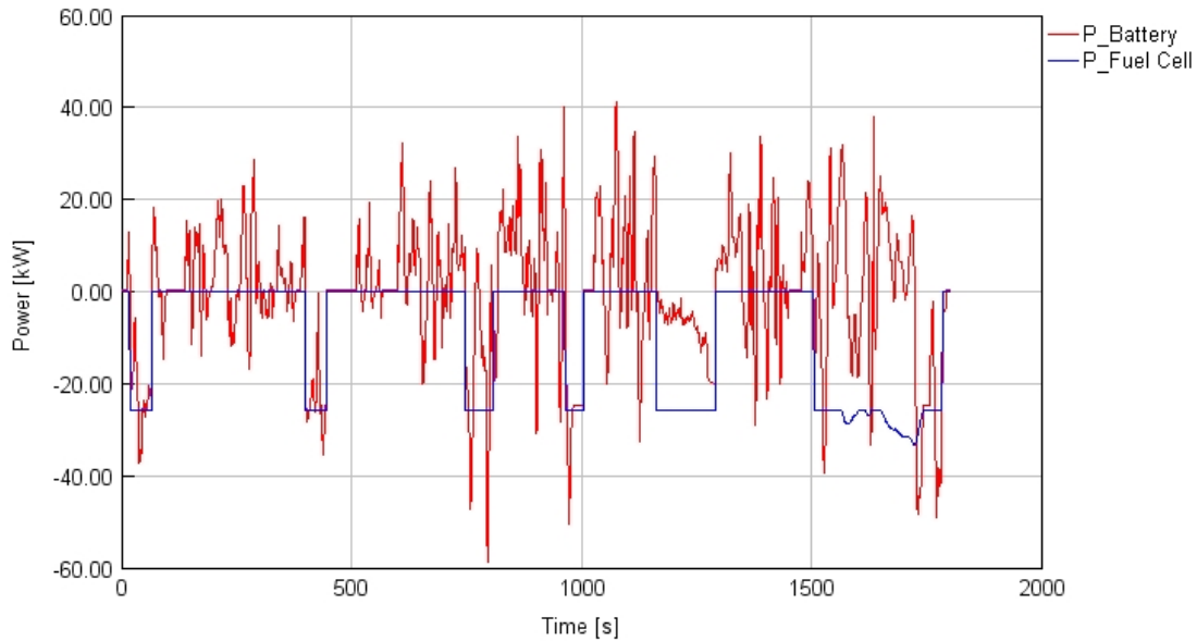
Figure 4.19: Battery power and fuel cell stack power for the Fuel Cell-PHEV.
