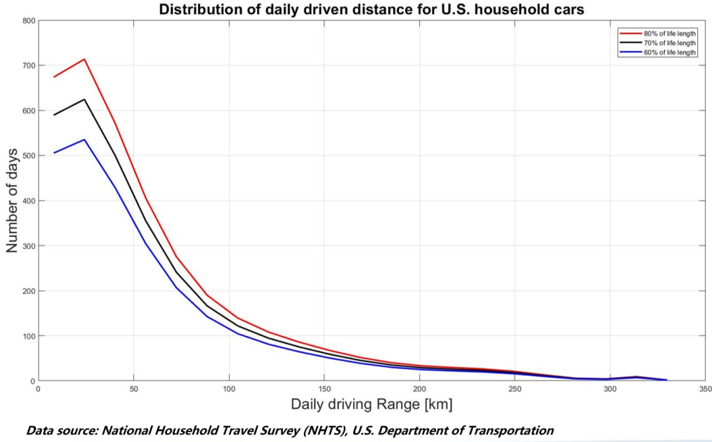
Figure 3.57: Distribution of the daily driven distance for U.S.household cars in number of days
