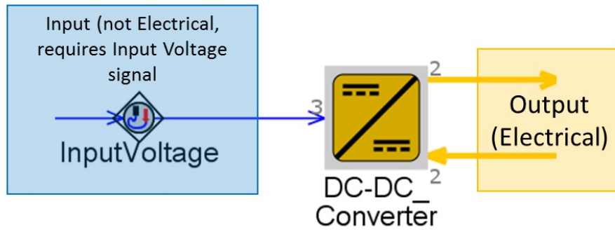
Figure 3.40: DC-DC converter required connection in GT-Suite
