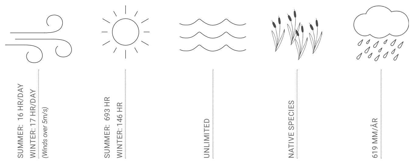
Data from Måseskär weather station (SMHI)
