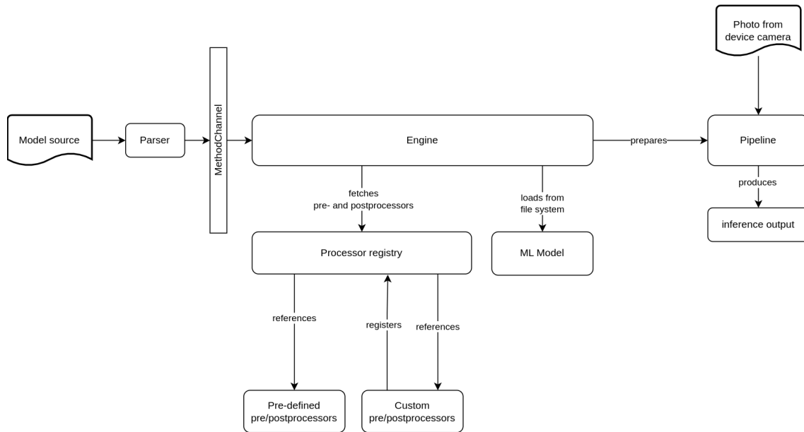
Figure 4.3: Illustration of how the model engine prepares an ML serving pipeline from a DSL instance.
