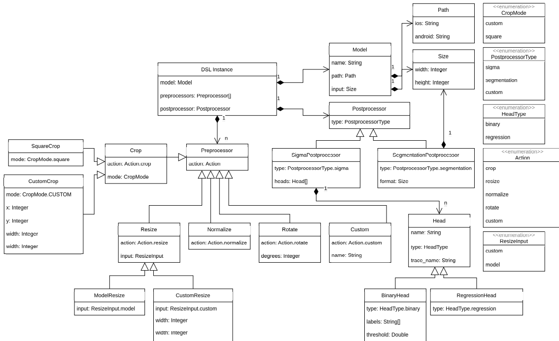
Figure 4.2: Abstract syntax of the DSL.
