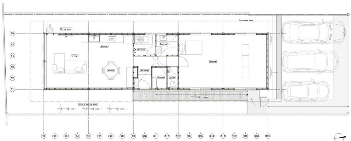
Floorplan [Drawing], by Tomoaki Uno Architects, 2018, Arch Daily
