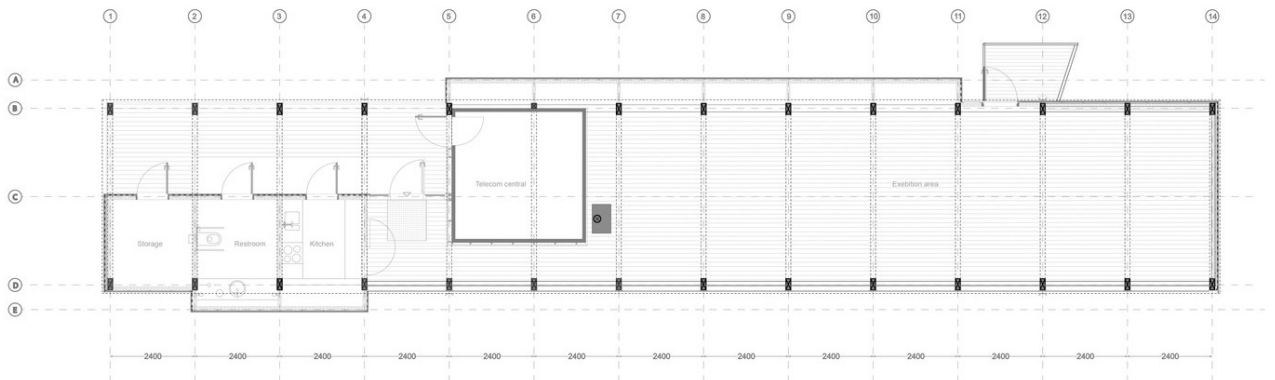
Floorplan [Drawing], by Marchesi, Hellum & Stikbakke, 2013, Arch Daily
