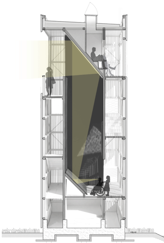
Perspective Section of Periscope Tower [Drawing], by OOPEAA, (n.d), OOPEAA
