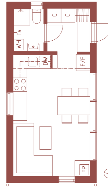
Figure 49. Entrance floor - Scale 1:200
