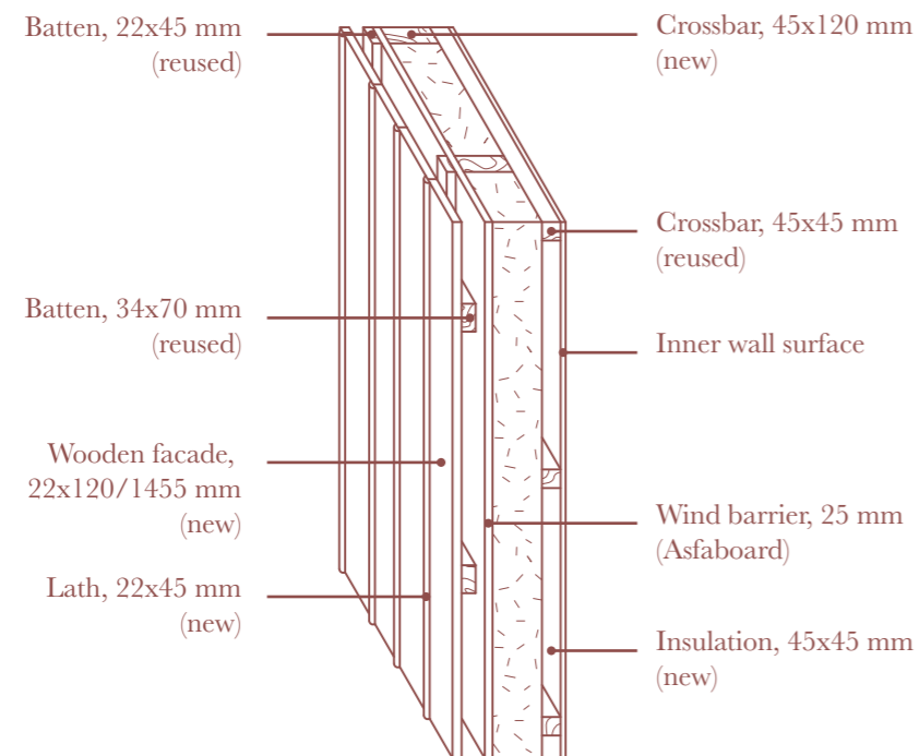
Figure 48. Detail of wall - Scale 1:20
