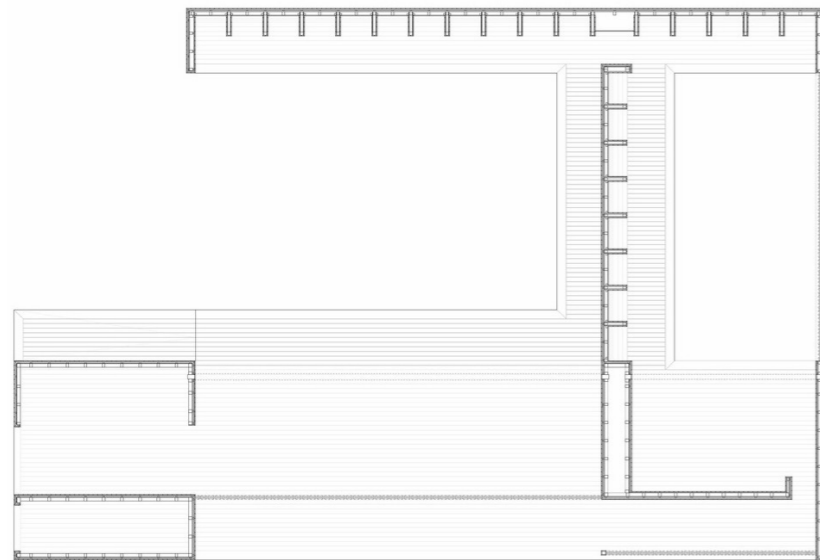
Fig. 9 Community centre Spinelli, plan Atelier U20. (2016)
