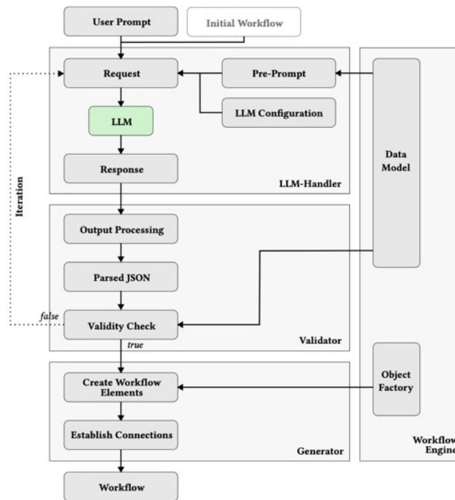
Figure 4.7: The proposed workflow with an integrated LLM, and LLM-handler (Reitenbach et al., 2024).
