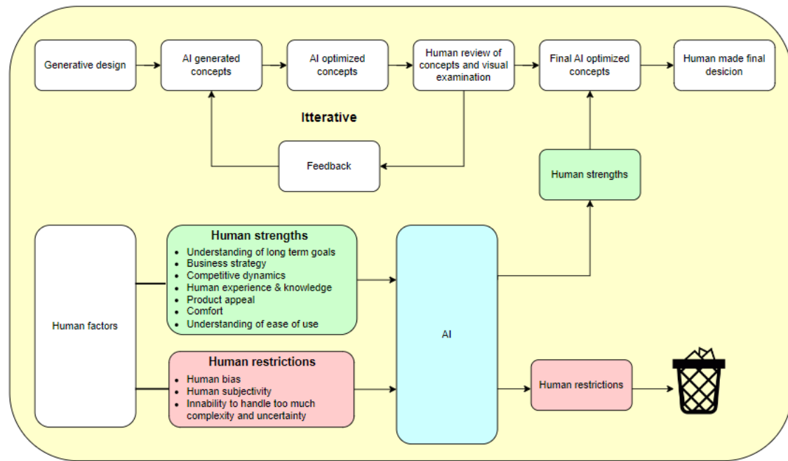
Figure 5.2: Visualization of how AI could support concept evaluation
