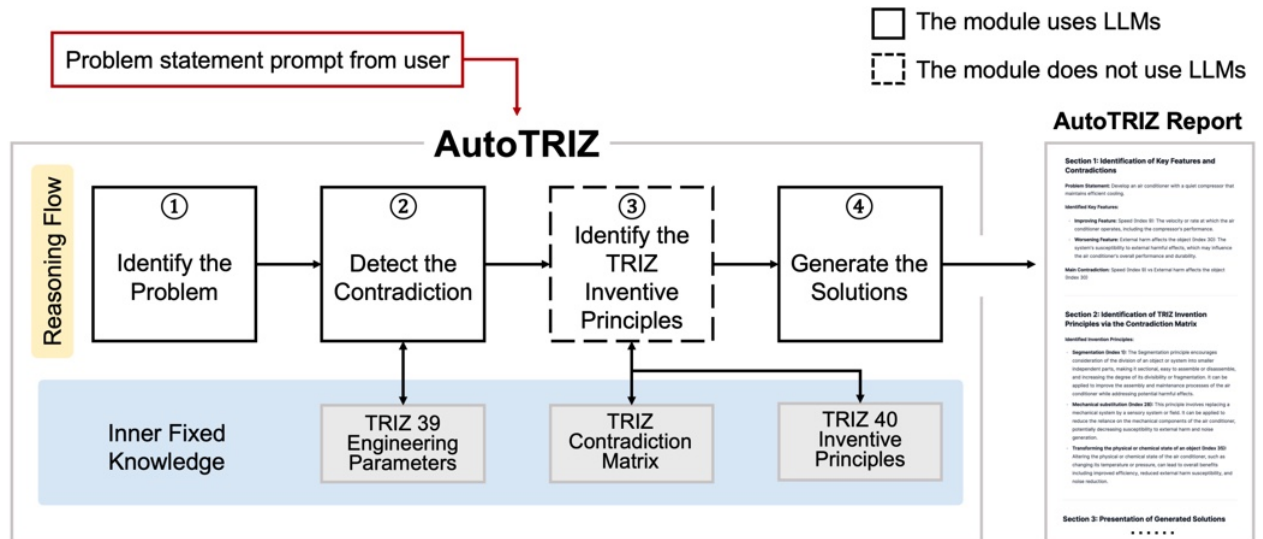
Figure 4.3: The process flow in AutoTRIZ (S. Jiang & Luo, 2024).
