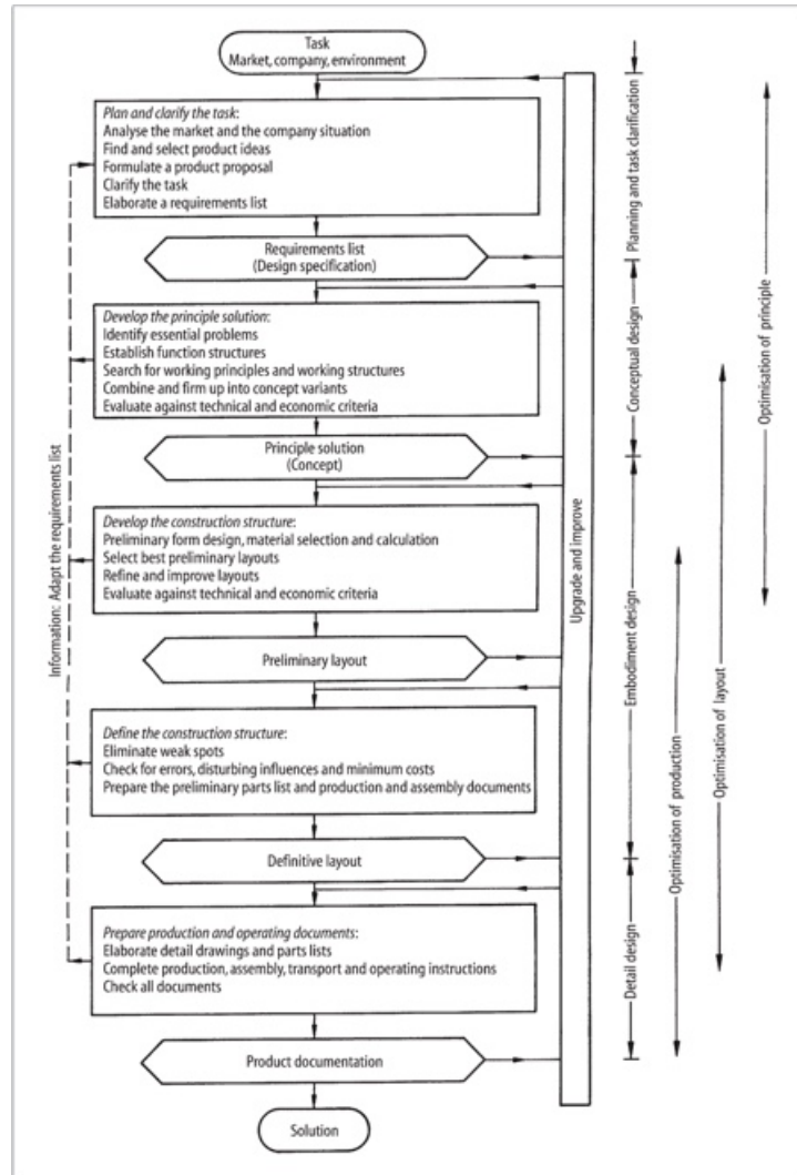
Figure 2.1: The ED process according to (Beitz et al., 1996)
