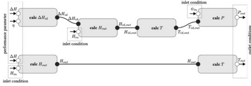
Figure 4.5: The workflow the LLM is asked to perform correct inquiries in (Reitenbach et al., 2024).
