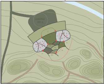
Cross firing clusters (front zone), overhead distribution grid (seated zone), and line array positions (middle and back zones)
