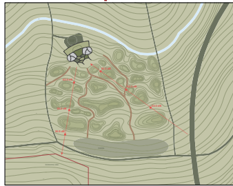
Broadband SPL sample points along noise path (unweighted, with noise mitigation measures)
