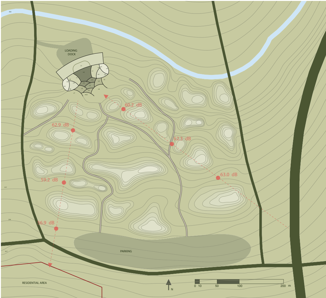
Broadband SPL sample points along noise path (unweighted, with noise mitigation measures)
