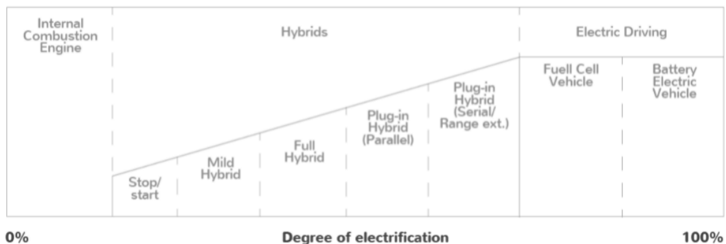
Figure 2-4 Different degrees of electrification (Anders, 2020)
