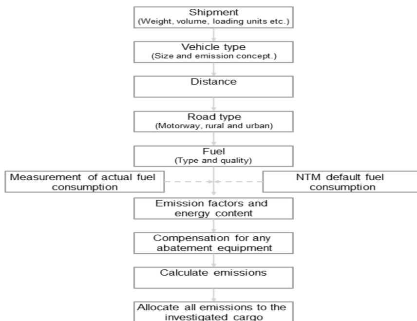
Figure 3-2 General calculation process of road cargo transport in NTM (NTM, 2021)
