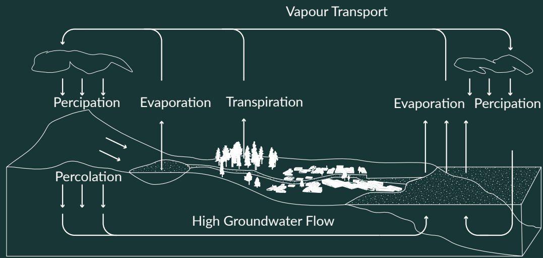
Figure 1: The changing water cycle
