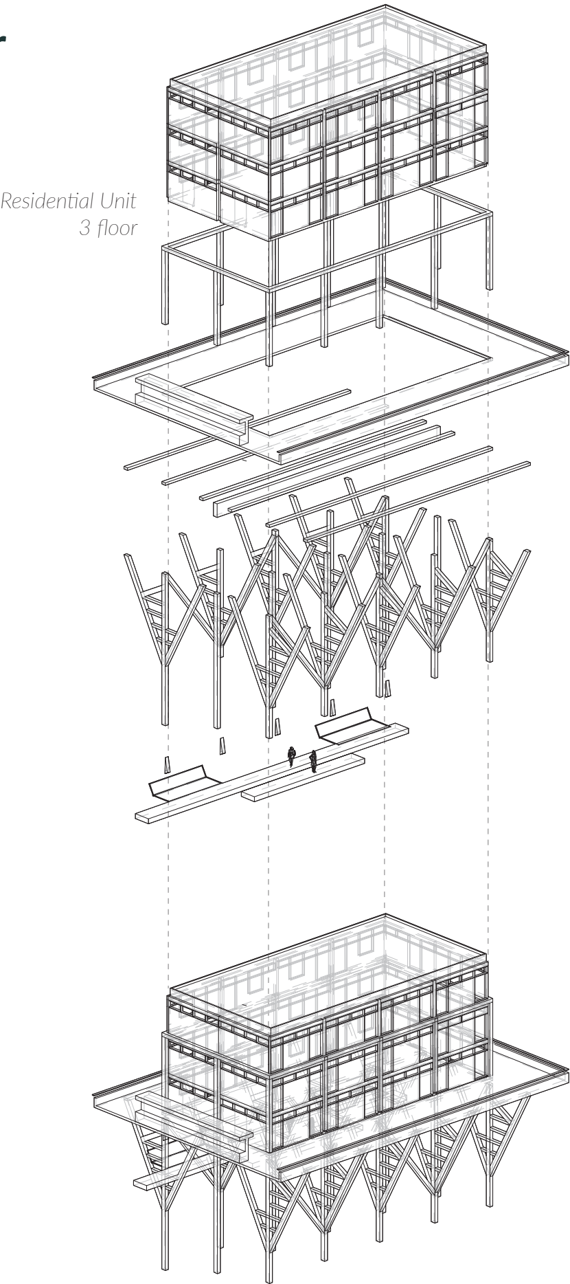
Figure 38: Axonometric - Shell Structure of the Elder Mollusc with submerged habitats and recreational gantries
