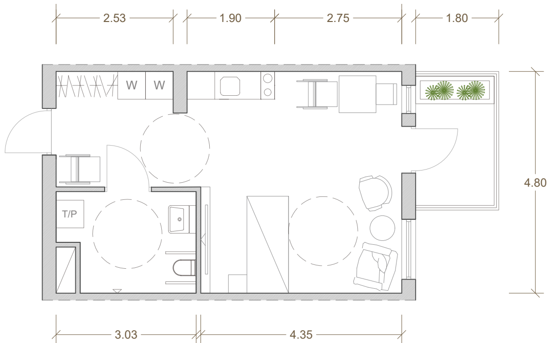
Apartment Plan, S = 1:80 (A4) (Unit: Meter)
