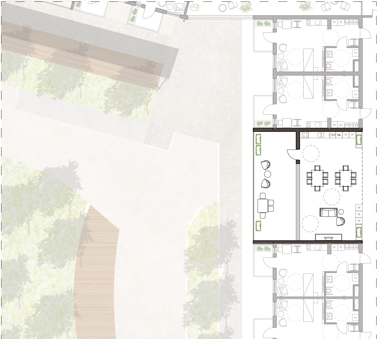
First Floor Plan, S = 1:200 (A4)
