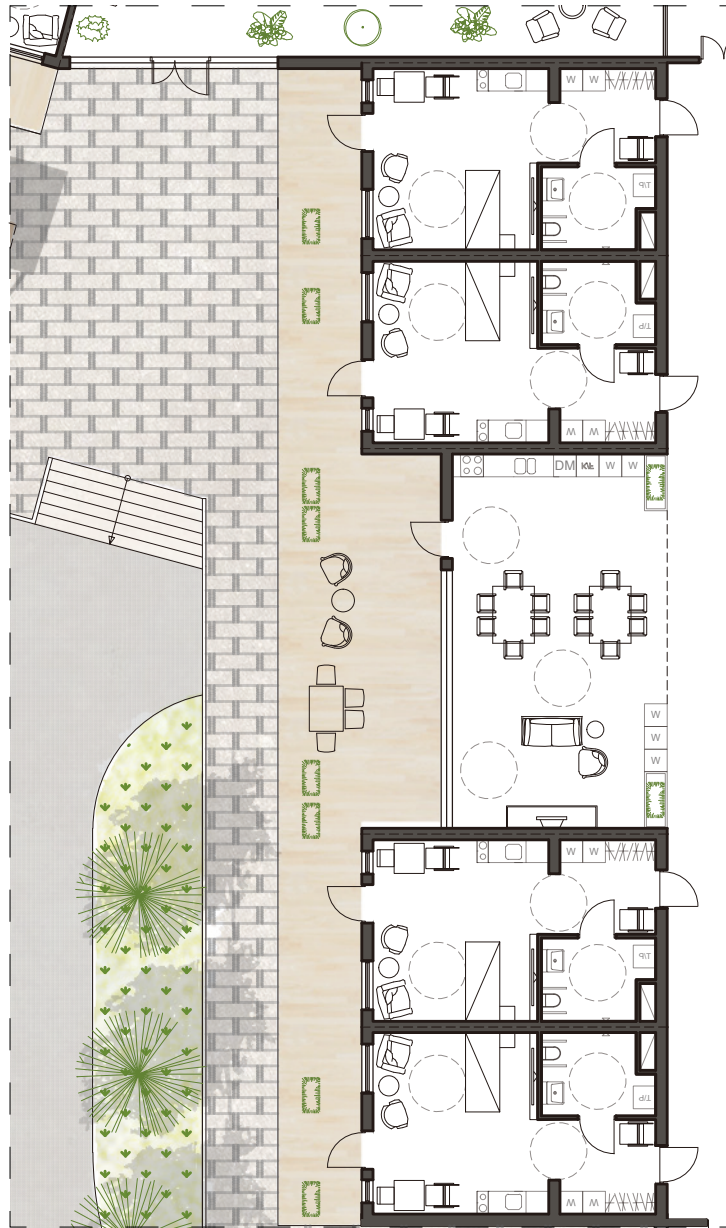
Ground Floor Plan, S = 1:200 (A4)
