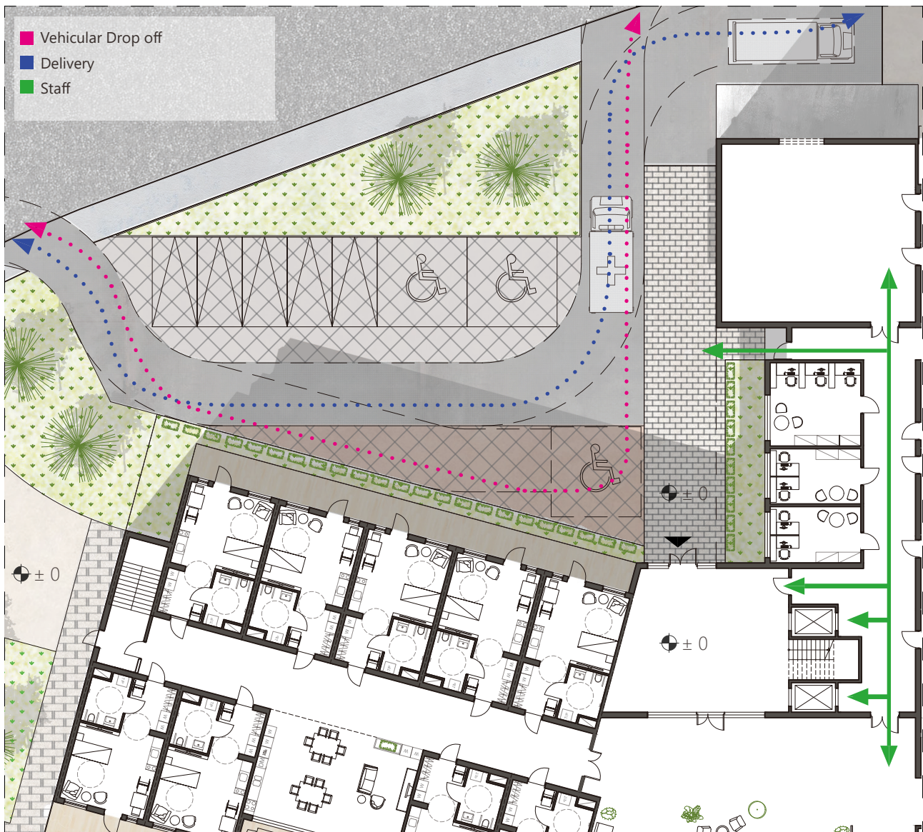
Ground Floor Plan, S = 1:300 (A4)
