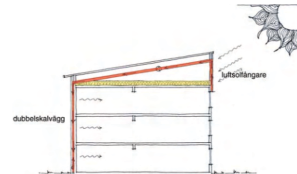
Figure 18: Heating system with solar air collectors and double walls
