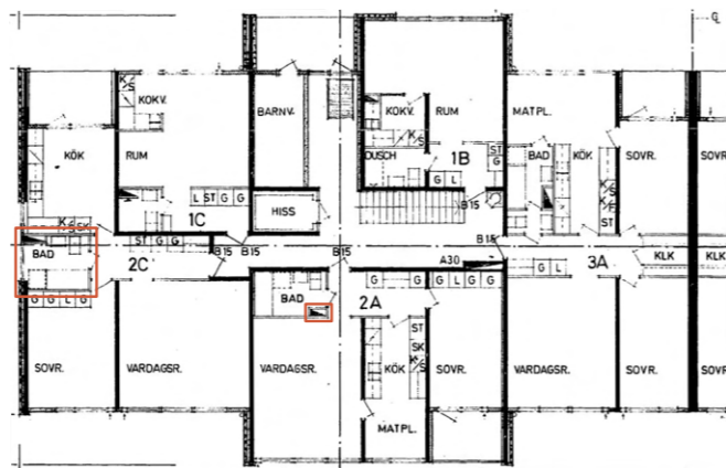
Investigated building with bathroom in apartment 2C and pishaft in apartment 2A marked
