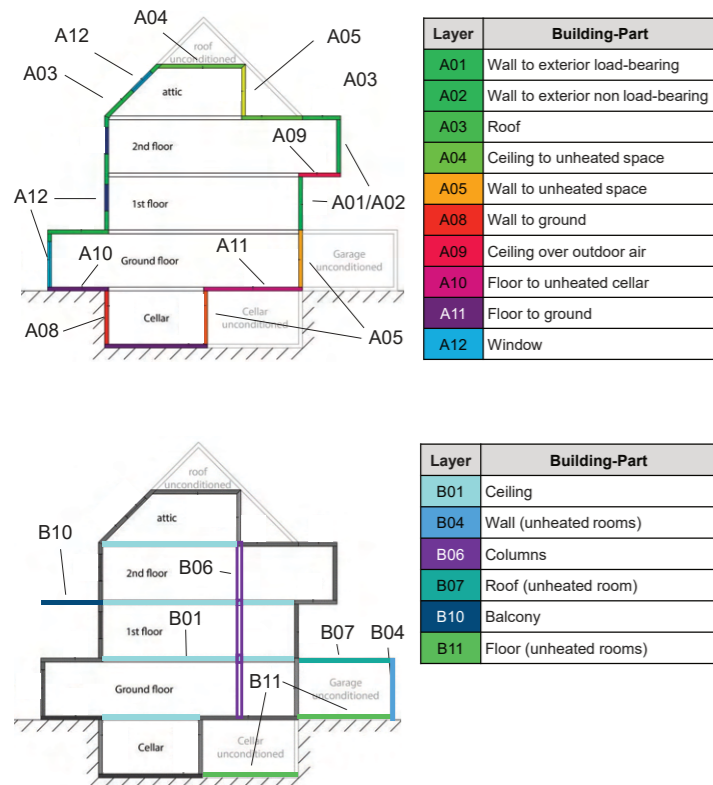
Figure 11 & 12: CAALA layers for the preliminary planning phase
