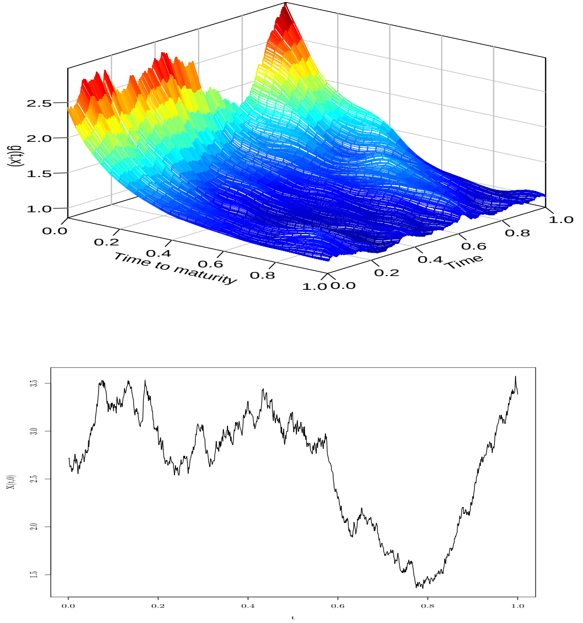
Figure 2: Future simulation and spot curve for \alpha = 0.2 and \kappa = 10 with Brownian drift.
