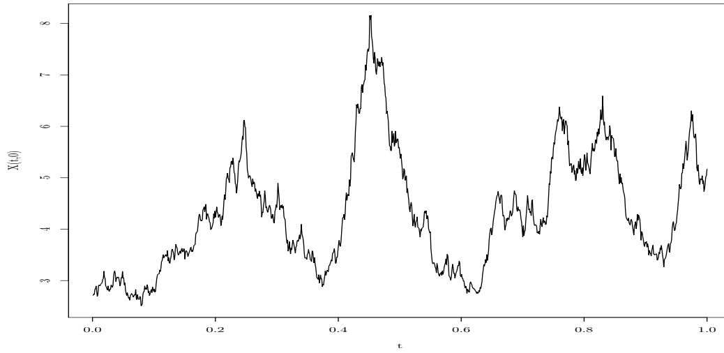
Figure 7: Future simulation and spot curve for \alpha = 4 and \kappa = 2 with NIG drift.
