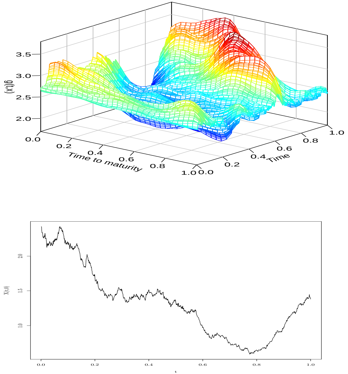
Figure 4: Future simulation and spot curve for \alpha = 4 and \kappa = 10 with Brownian drift.
