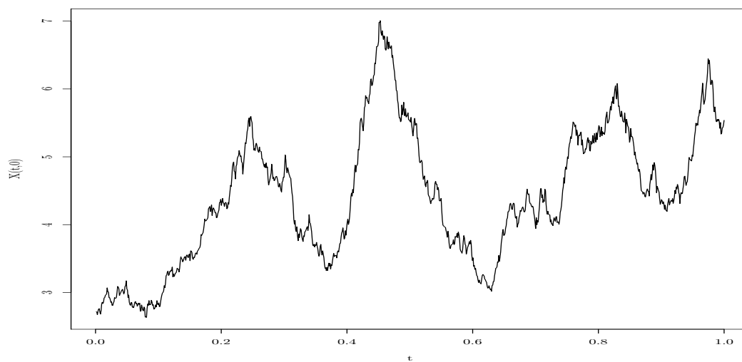
Figure 6: Future simulation and spot curve for \alpha = 0.2 and \kappa = 10 with NIG drift.
