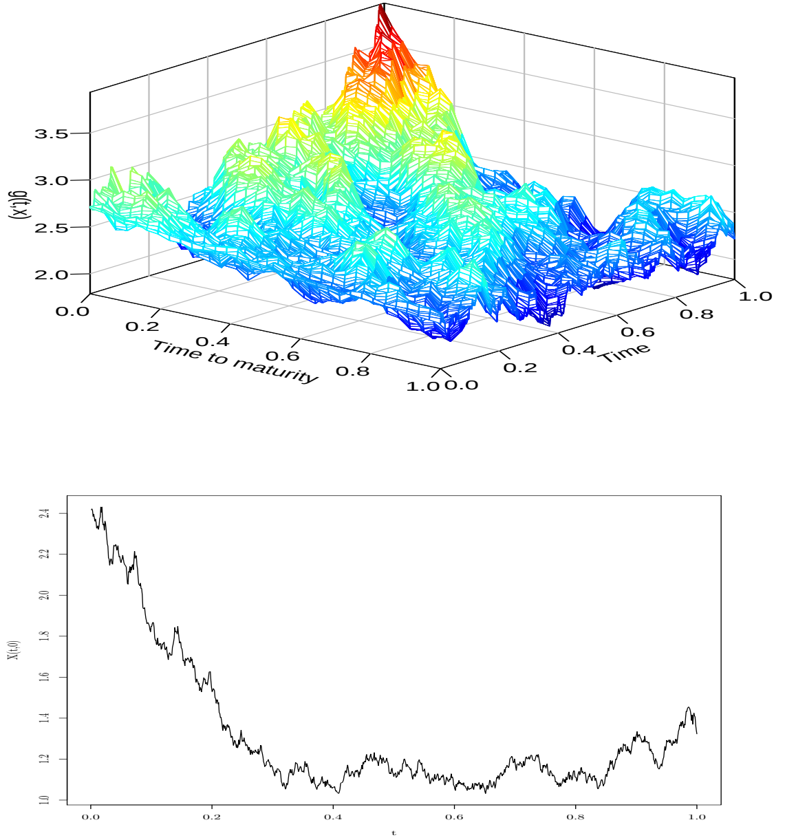
Figure 8: Future simulation and spot curve for \alpha = 4 and \kappa = 10 with NIG drift.
