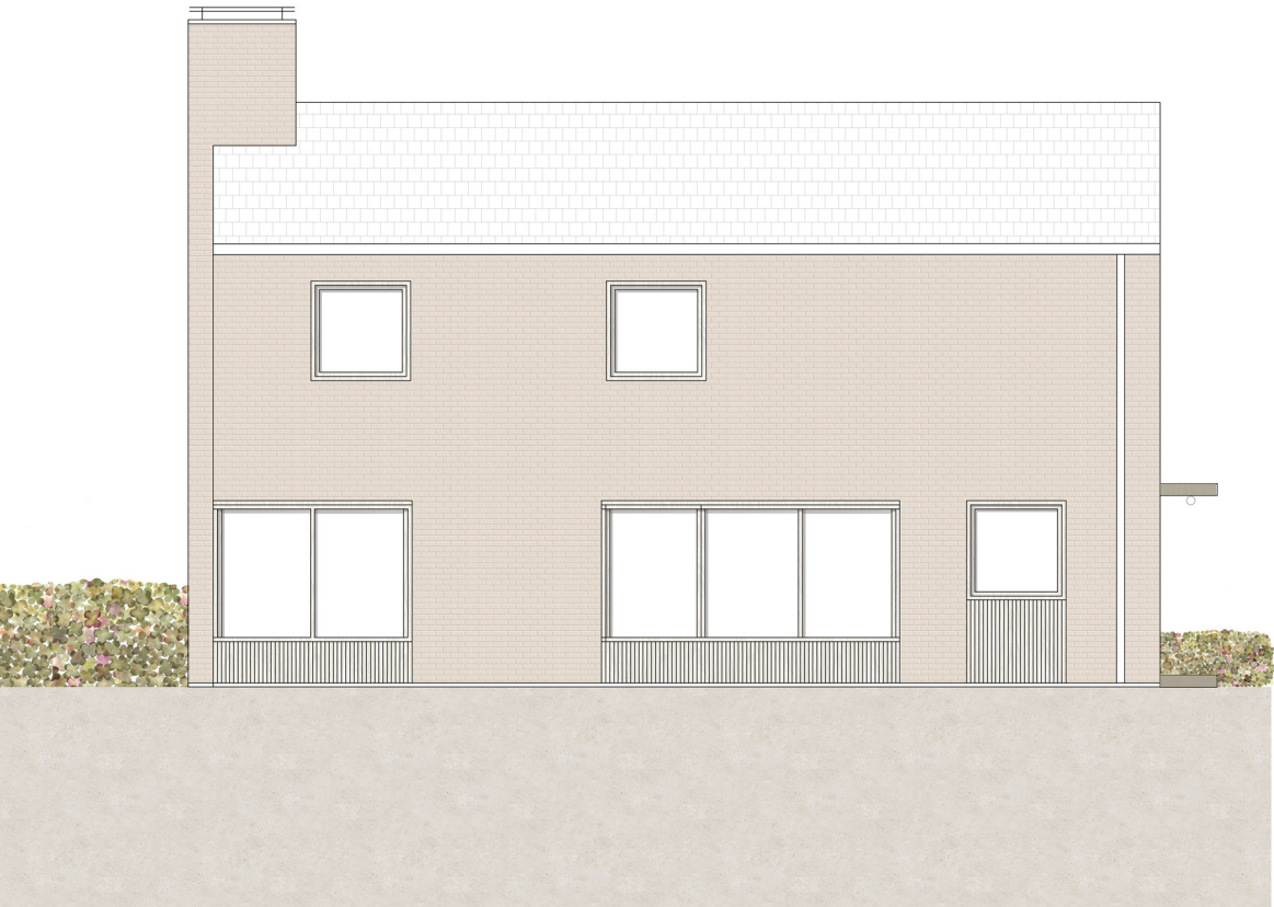
FIGURE 191: Right facade wood. Scale 1:100 FIGURE 192: Right facade brick. Scale 1:100
