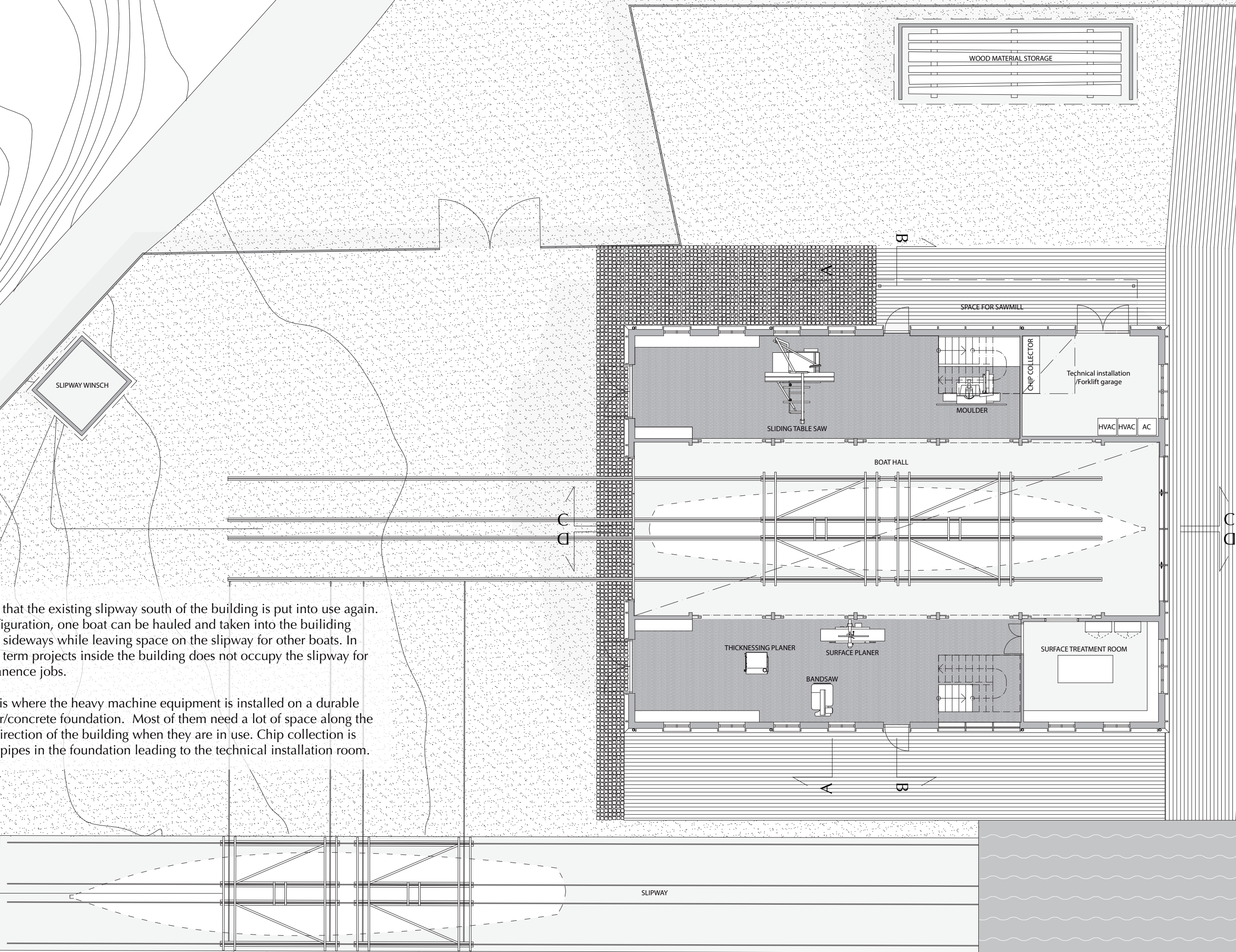
Fig. 75. First floor scale 1:150
