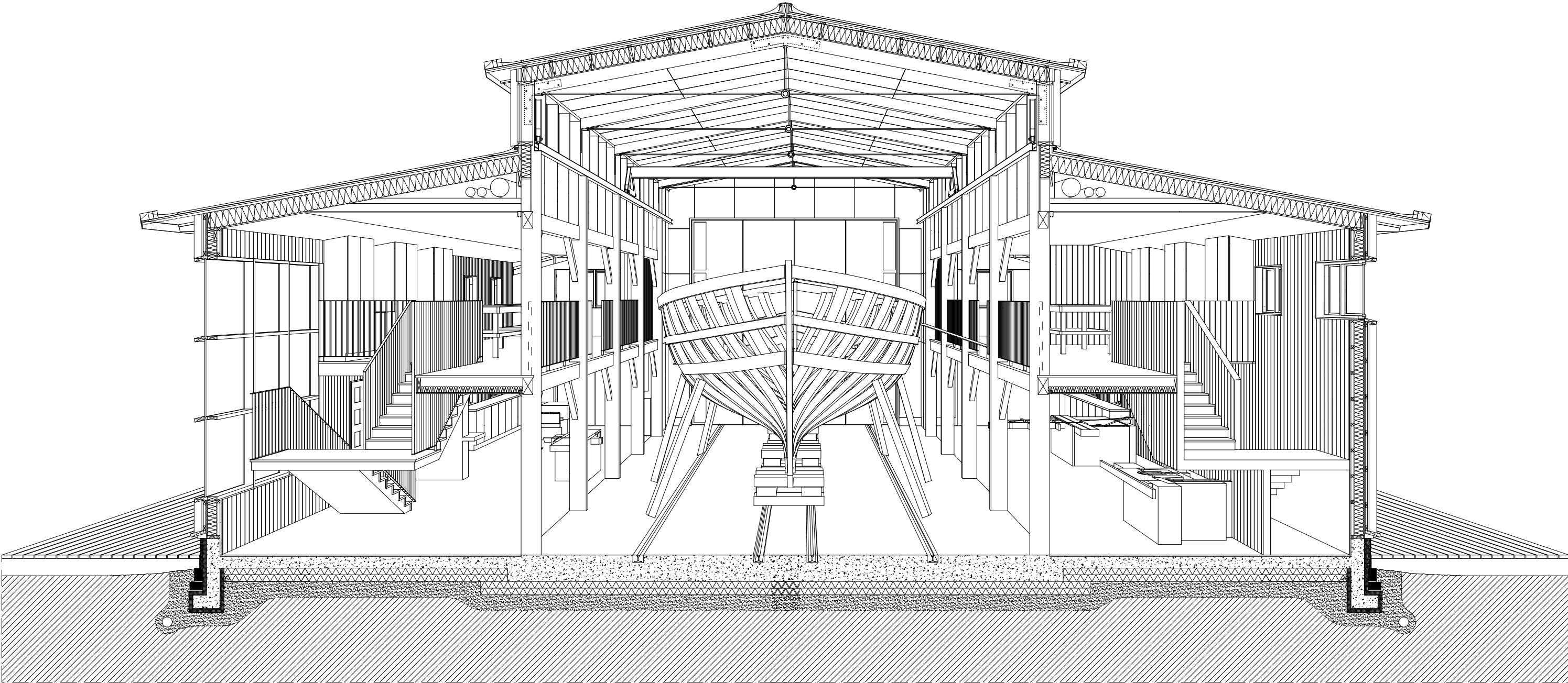
Fig. 77. Section perspective
