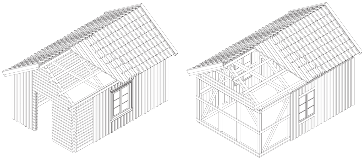
Fig. 9. Basic principle of stacked timber construction and timber frame construction
