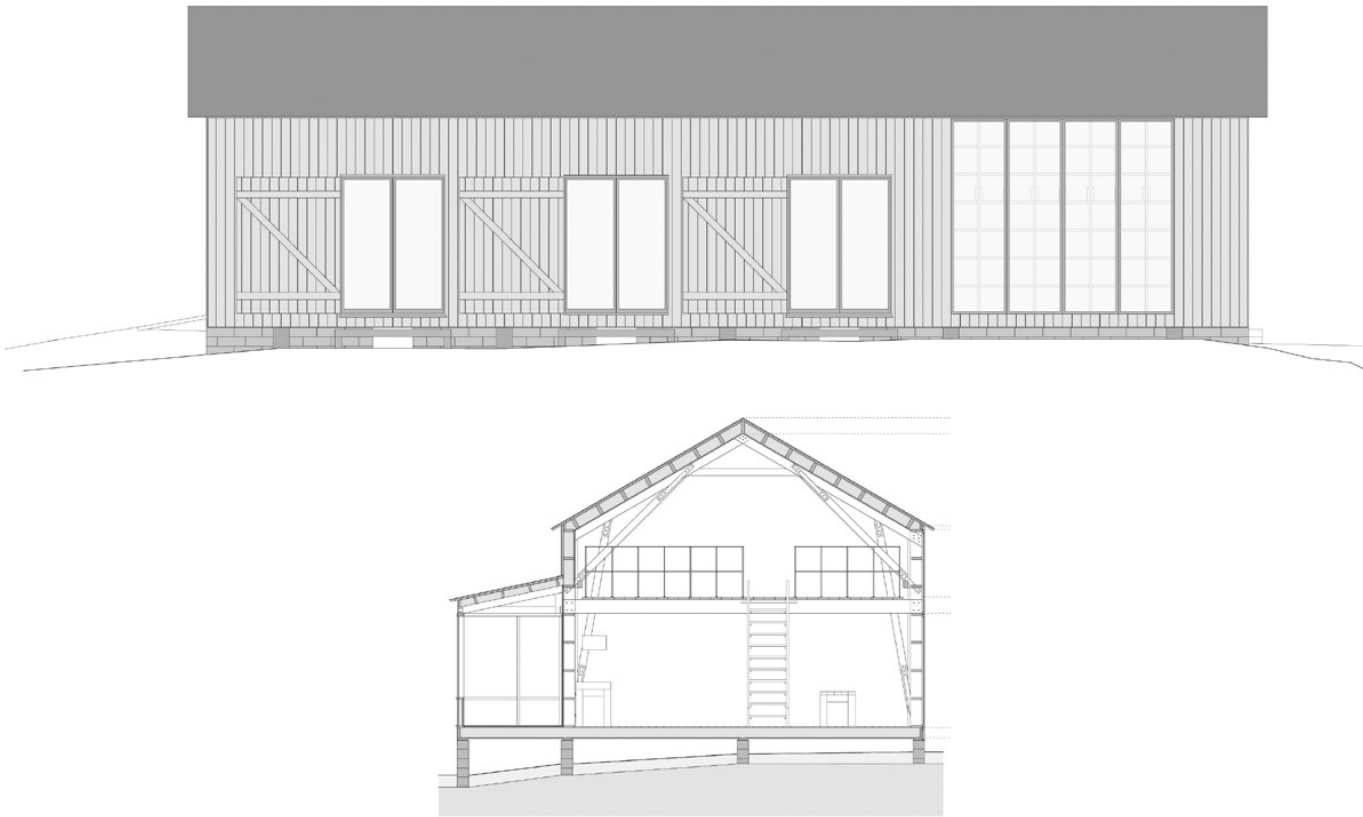
Fig. 35-36. Drawing of Atelje Södersvik
