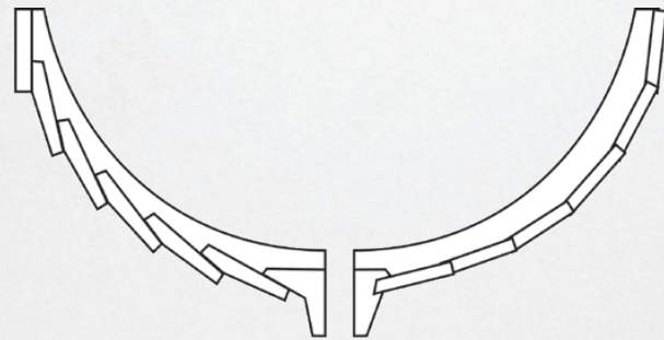
Fig. 31. Section of clinker built hull (left) and carvel built hull(right)
