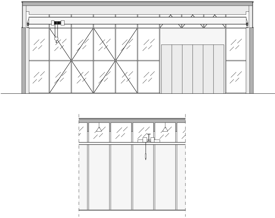
Fig. 39-40. Drawing of LOT Holzbau
