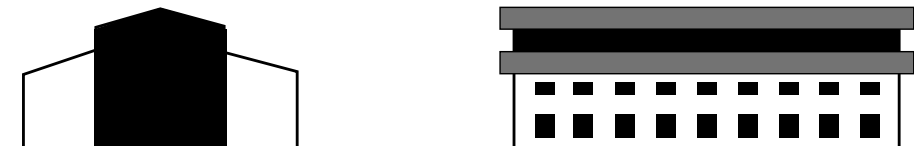
Fig. 63. The tall boat hall is all covered in glass, workshop areas are closed.
