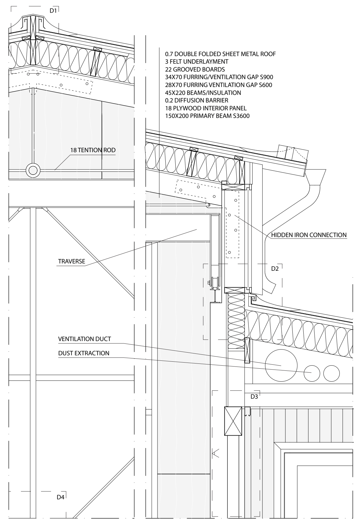
Fig. 78. Detailed section & facade elevation scale 1:25
