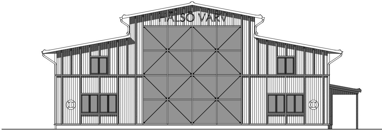
Fig. 69. Facade towards east
