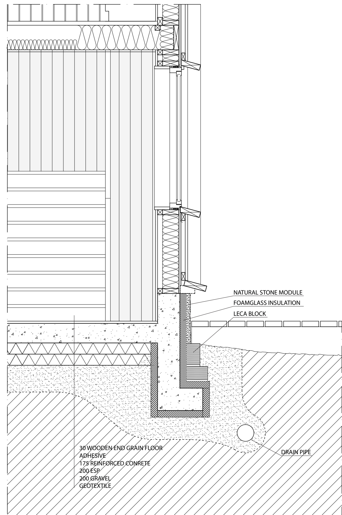
Fig. 80. Detailed section & facade elevation scale 1:25
