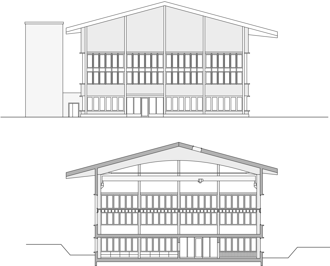
Fig. 37-38. Drawing of Wood production facility
