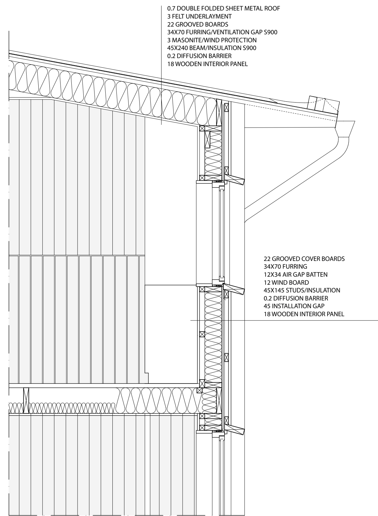
Fig. 79. Detailed section & facade elevation scale 1:25
