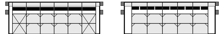
Fig. 62. Testing the amount of pillars in the exposed timber frame structure. Large diagonal braces are needed for the traverse. In the iteration to the right, these can be integrated into the wall. This number of pillars also works better with the plans.
