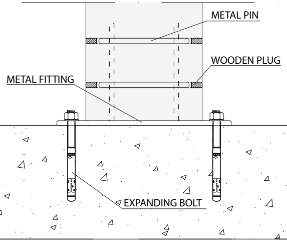
D5 CONNECTION TIMBER FRAME-GROUND
