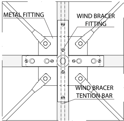
D4 WINDOW CONNECTION
