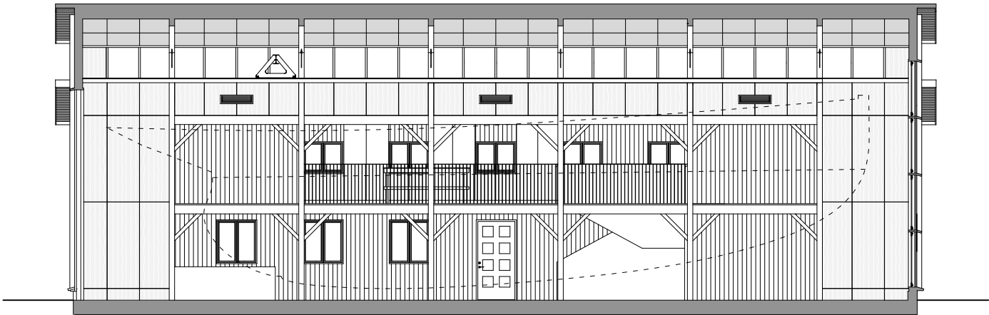
Fig. 72. Section C-C
