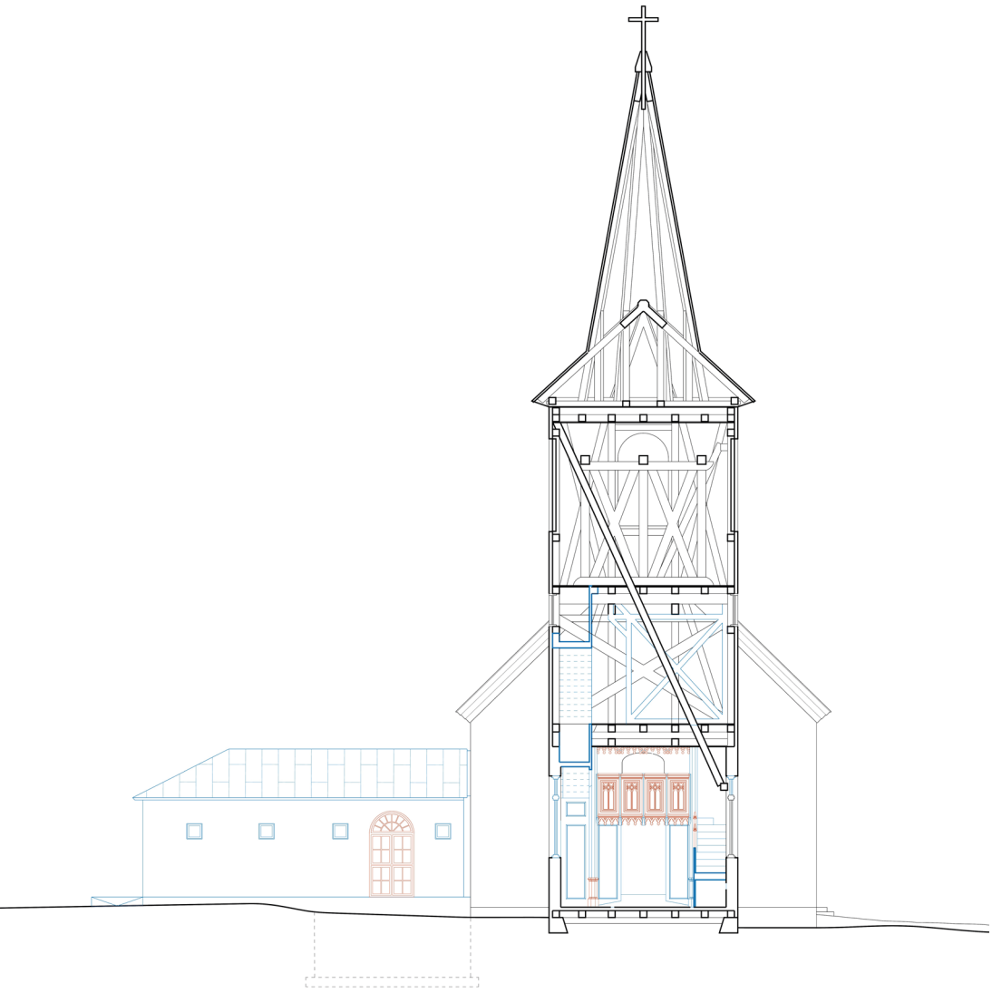
Fig. 108 Section & Elevation C-C Scale 1:200
