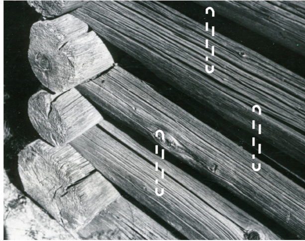
Figure 16. Traditional timber wall with internal wooden dowels (Västmanlands museum, 2018).
