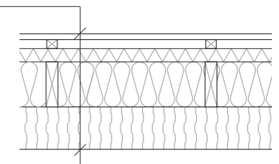
Horizontal section of outer wall
