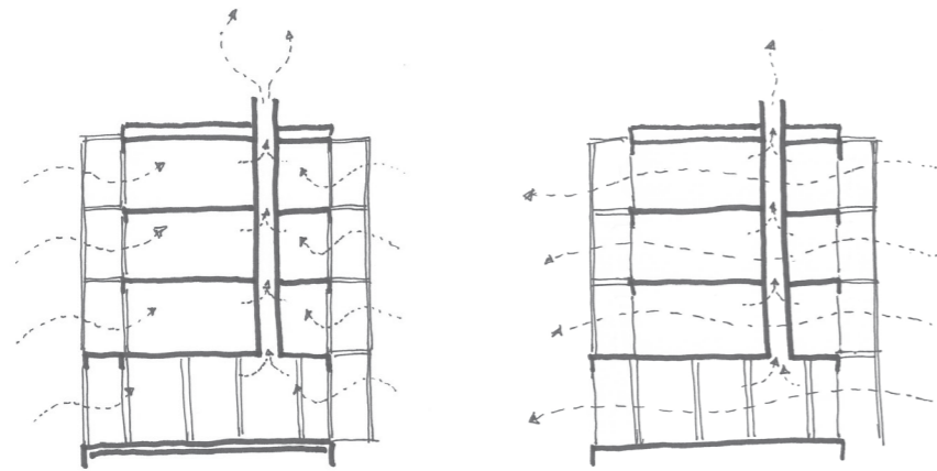
Winter scenario with prewarming of intake air through buffer zones. Exhaust chimney using stack effect.
