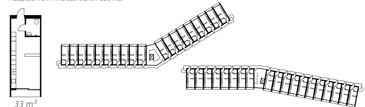
FIGURE 2.7 Snabba hus Råcksta modular apartments
