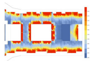
Analysis 4. Wing with two atriums and a partially recessed facade.
