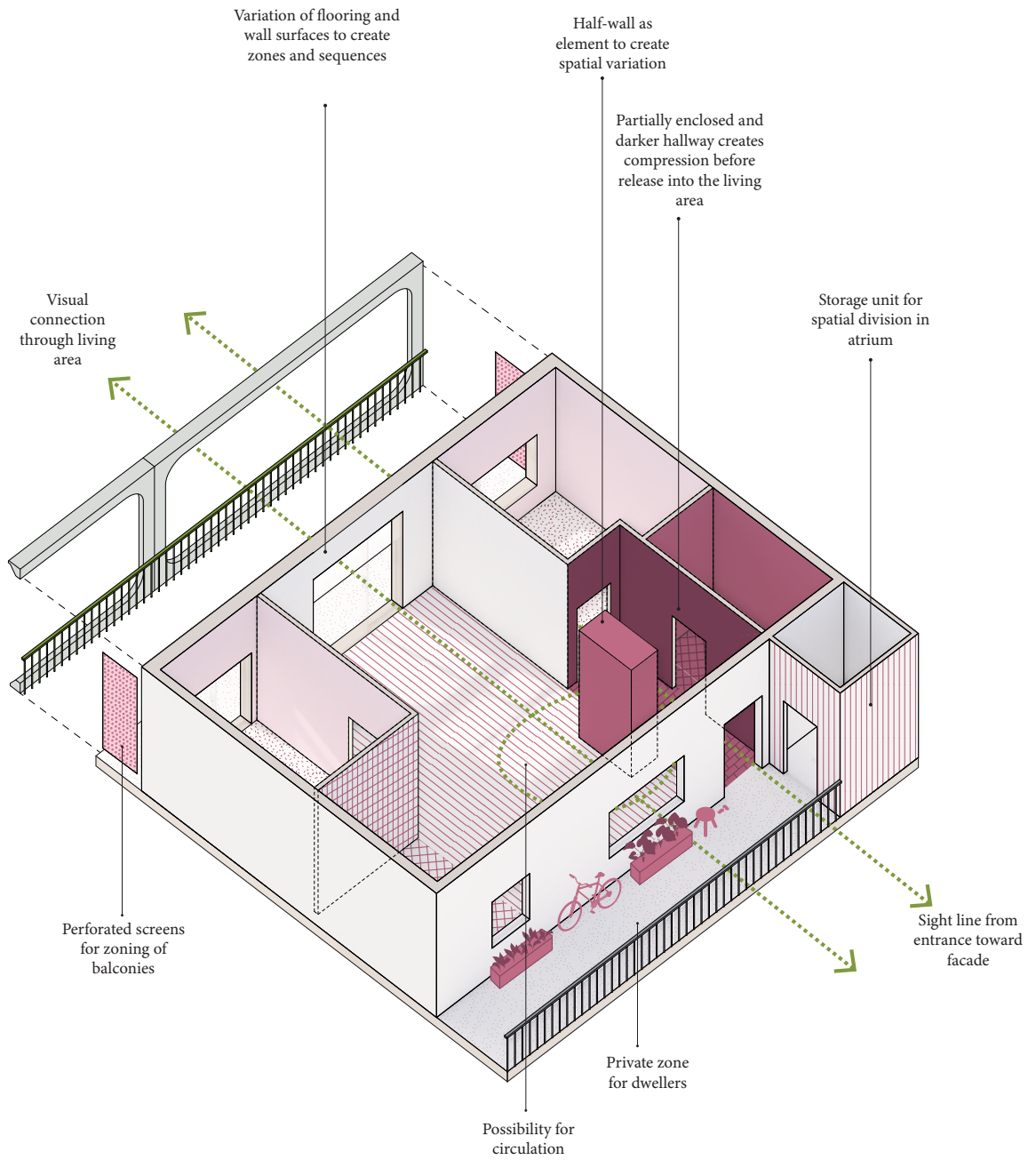
Axonometry explaining the atmospheric interventions on apartment level.
