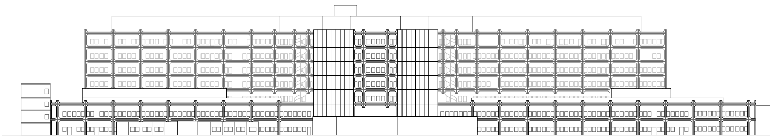
South elevation
