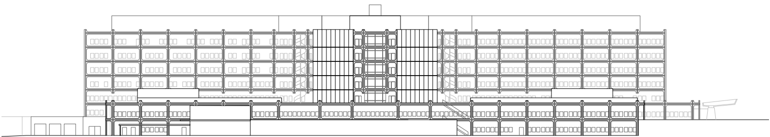
East elevation
