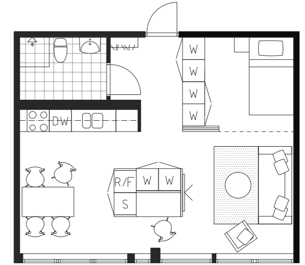
Figure 49. Transformed floor plan. 1:100
