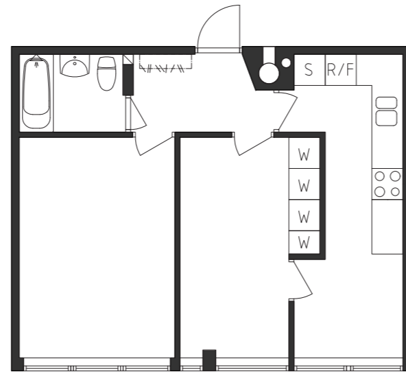
Figure 45. Original floor plan. 1:100
