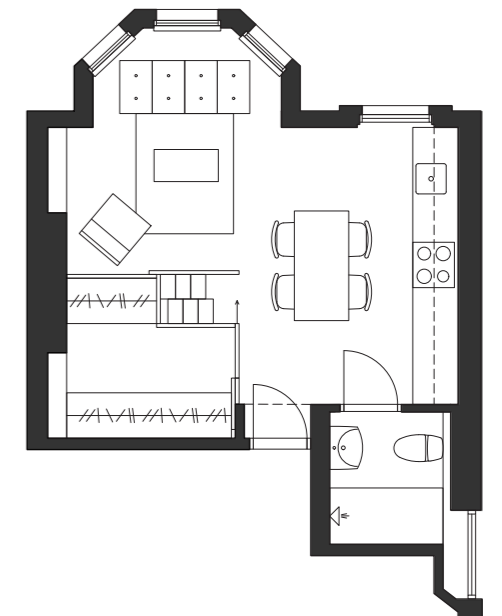
Figure 28. Floor plan 1:100
