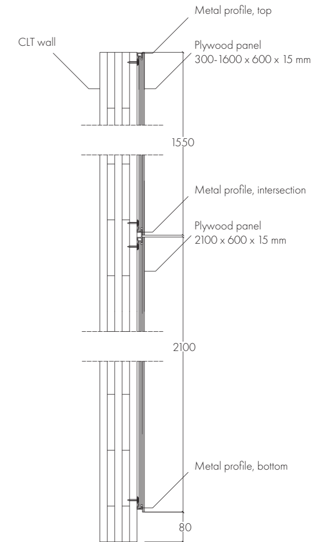
Figure 80. Detail drawing of panel fastening system.
