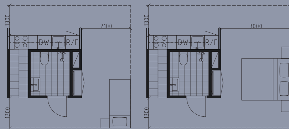
Figure 135, 136. Illustration showing the minimum measurement for the space around the Living Box, for a single- or double-bed.
