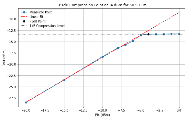
Figure B.2: Compression Points found at 50.5 GHz
