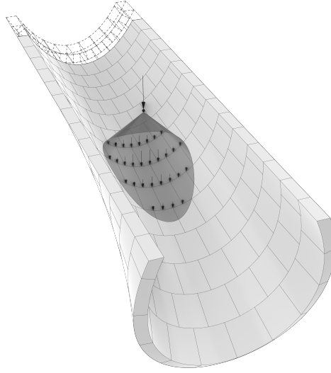
Figure 4.6: Assumed load distribution in the fill material
