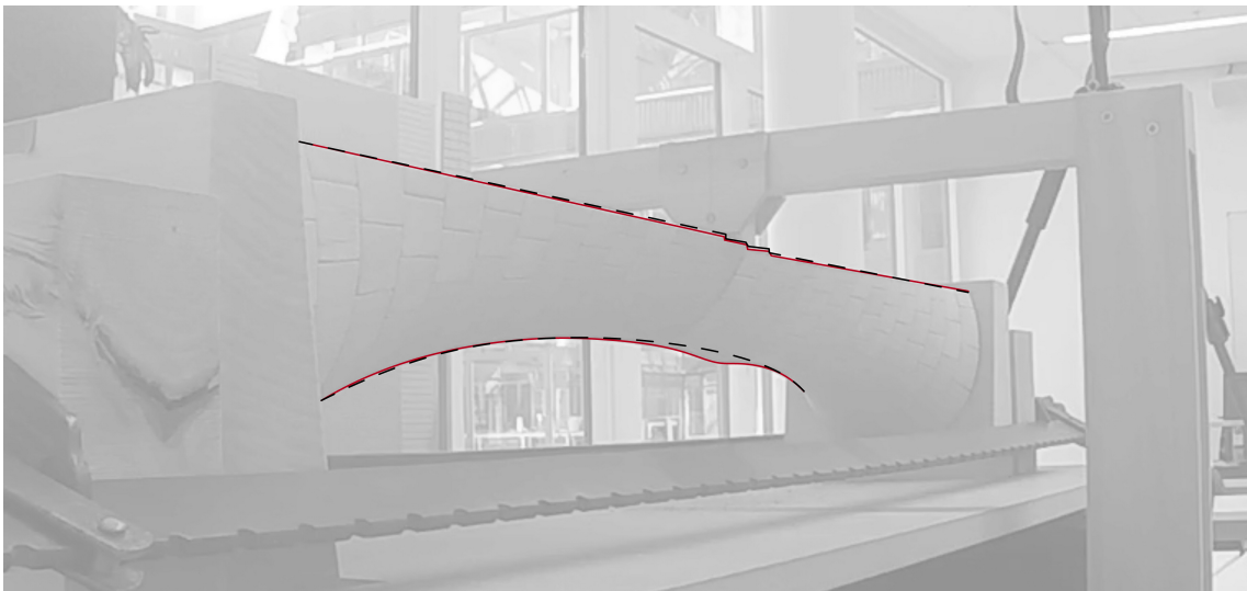
Figure 5.8: Load test of catenary with the load placed at 3/8 point, deformation at approximately 20 kilograms. Angled perspective.
