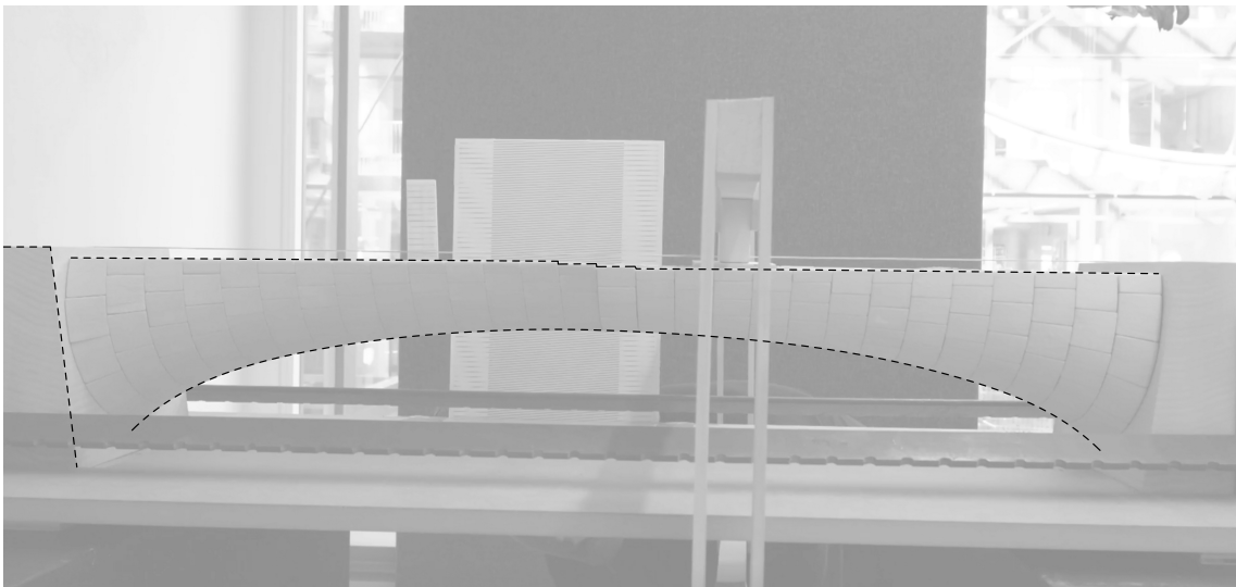
Figure 5.4: Load test of catenary with the load placed at 3/8 point, loaded with 1 kilogram.
