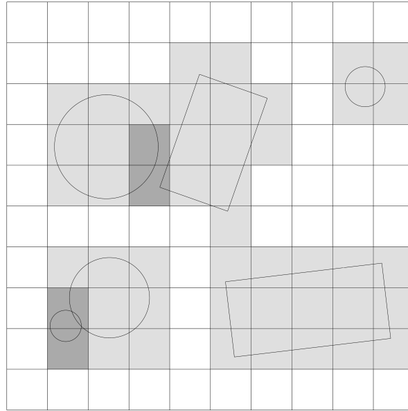
Figure 2.10: Munjizas detection algorithm: Areas marked in darker grey are occupied by two or more bodies
