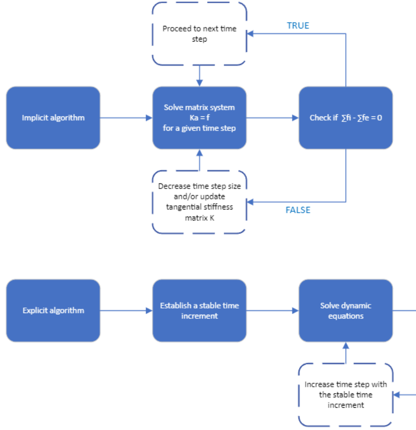
Figure 2.9: Flow chart describing the procedure for an implicit and explicit routine
