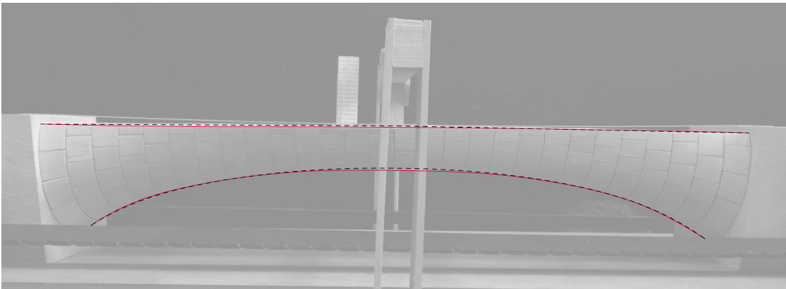
Figure 5.10: Load test of catenary with the load placed at the midpoint, deformation at approximately 10 kilograms. Red line: outlines of the bridge, black dashed: initial shape.
