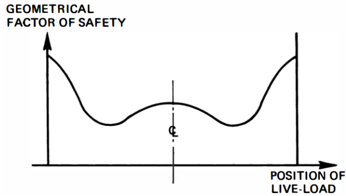
Figure 2.7: Geometrical safety factor for an arch. [25]
