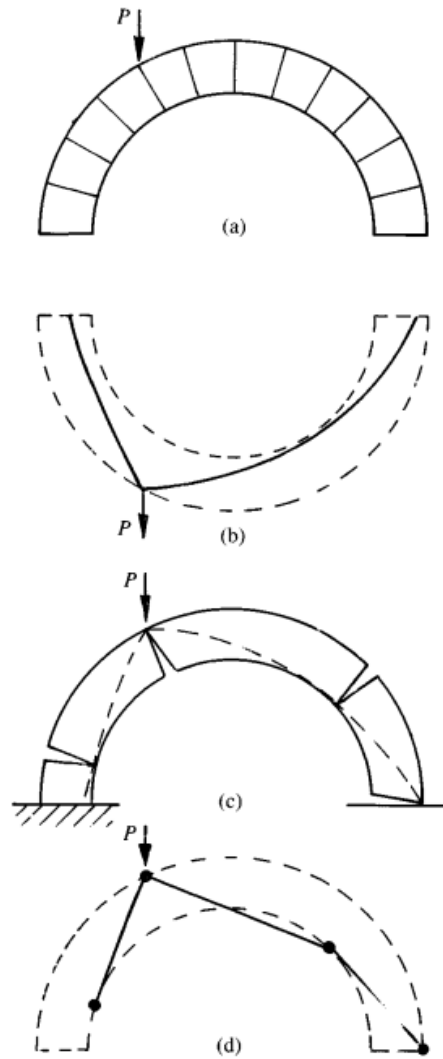
Figure 2.6: Collapse mechanism of an arch influenced by a concentrated force [26].
