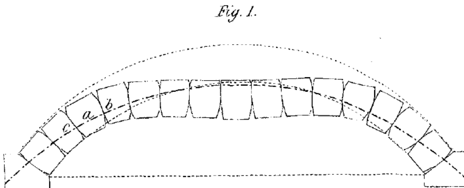
Figure 2.5: Drawing of Barlow's arch scale model [28]
