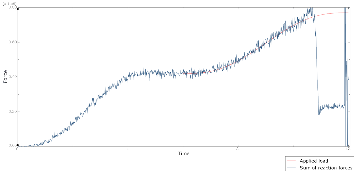
Figure 3.13: LC1: Vertical reaction force and applied load
