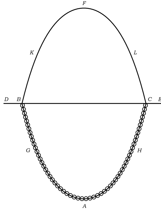
Figure 2.1: The hanging chain principle explaining the concept of the thrust line. Redrawn from Poleni [37]
