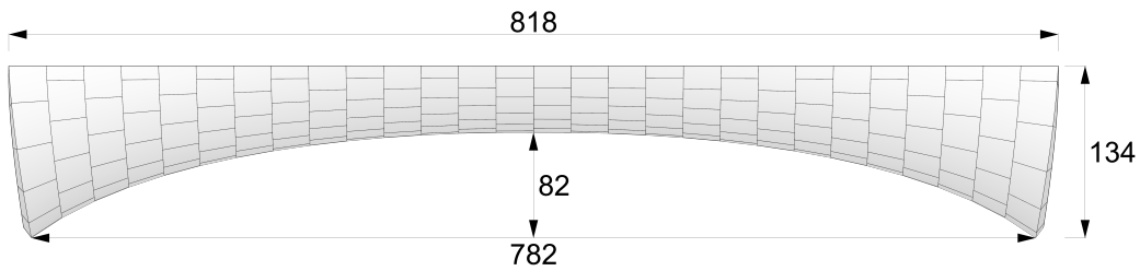
Figure 3.4: Elevation of the circle bridge [mm]
