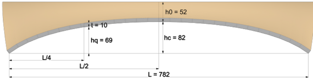
Figure 3.5: Dimensions of simplified circle cross-section bridge for hand calculations [mm]. Width of the bridge 139 mm.
