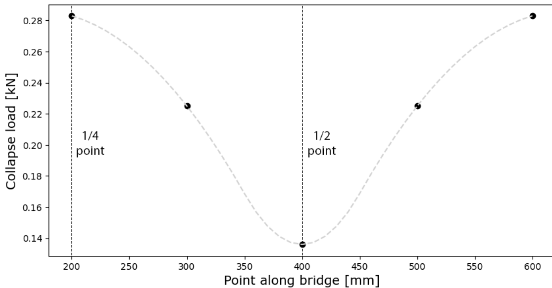
Figure 5.12: Collapse load for the analysed loading positions
