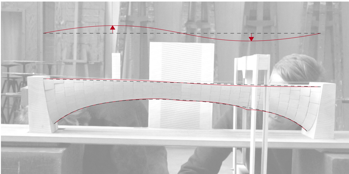
Figure 5.2: Load test of catenary with the load placed at the quarter point, deformation at approximately 27 kilograms. Red line: outlines of the bridge, black dashed: initial shape.
