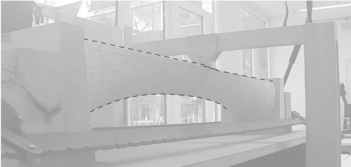
Figure 5.7: Load test of catenary with the load placed at 3/8 point, loaded with 1 kilogram. Angled perspective.
