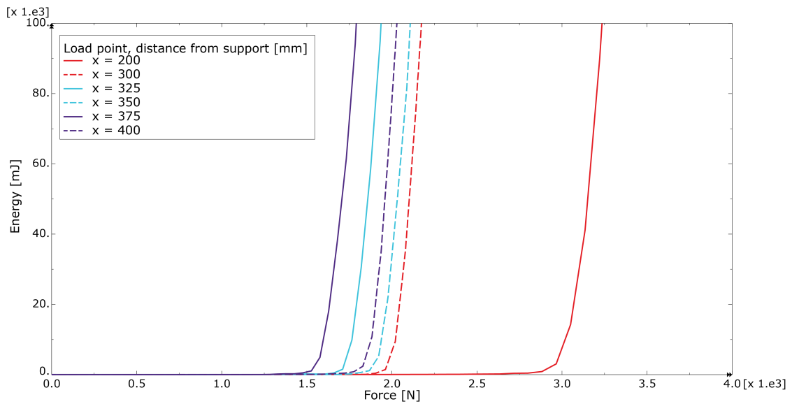
Figure 5.13: Catenary: Force-Kinetic Energy graph for different loading positions defined from the support
