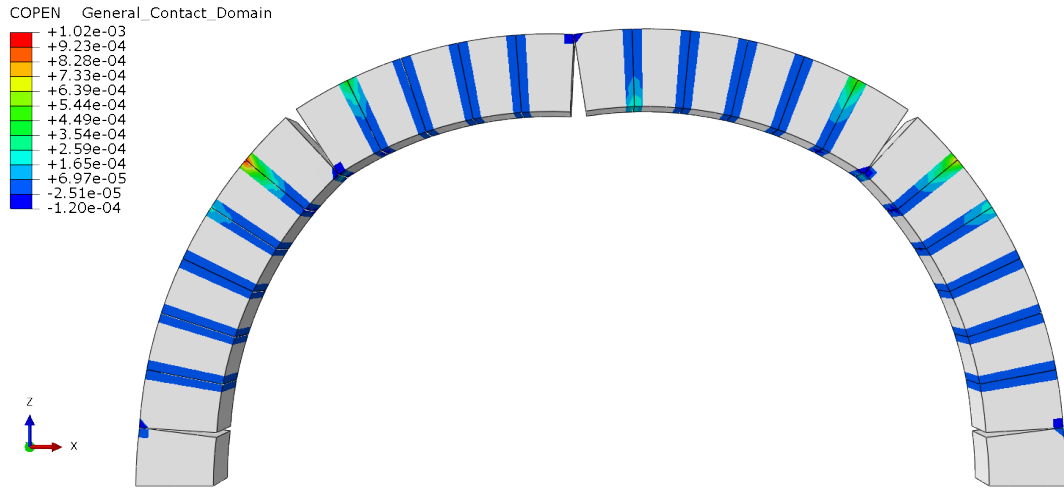
Figure 3.12: LC1: Contact openings at collapse stage: t = 10.4s
