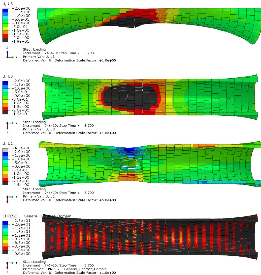
Figure A.7: Circle: Deformation figures for a load placed at y = 325 mm (a) Elevation: Vertical displacement. (b) Top view: Vertical displacement. (c) Top view: Horizontal displacement. (d) Top view: Contact pressure between voussoirs.
