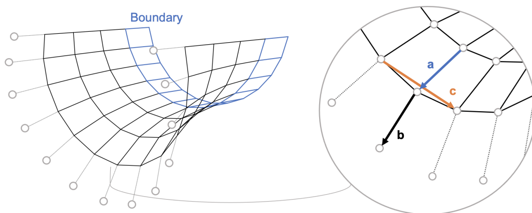
Figure 2.4: Vectors used for form finding of hydrostatic bridge. Redrawn from [7].
