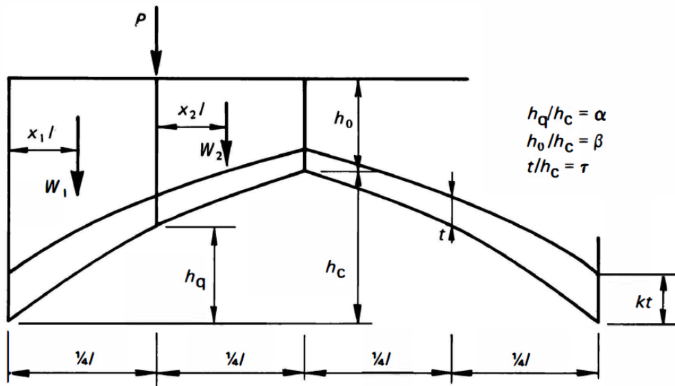
Figure 2.8: Physical quantities needed for prediction of load capacity of concentrated load P . [25]
