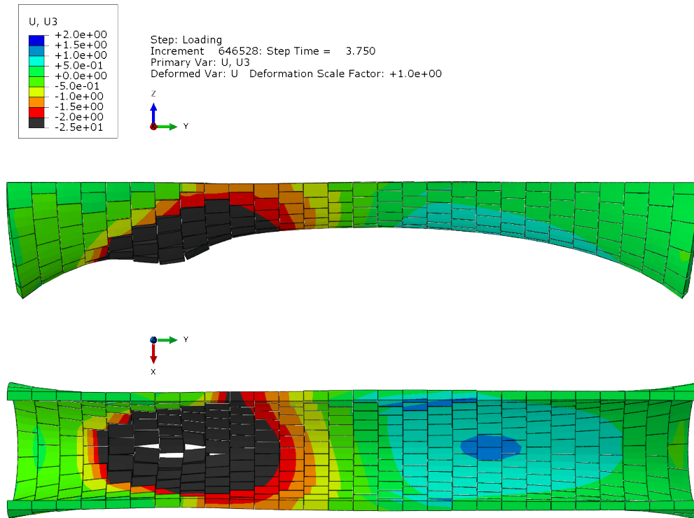
Figure 5.16: Catenary: Elevation and top view of vertical displacement [mm] for a load positioned in the quarter point of the span ( y = 200 mm). Force: 2.97 kN
