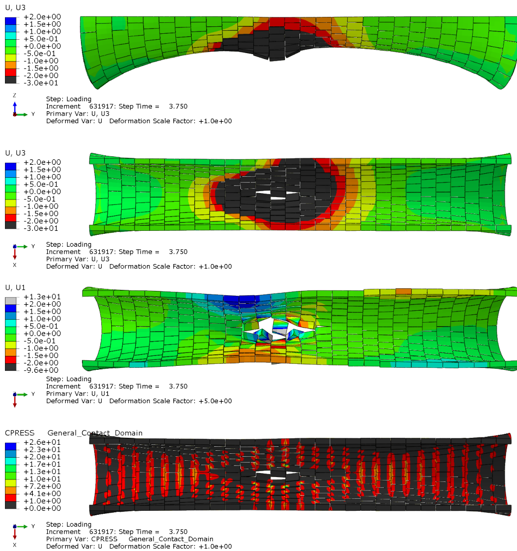
Figure A.2: Catenary: Deformation figures for a load placed at y = 350 mm (a) Elevation: Vertical displacement. (b) Top view: Vertical displacement. (c) Top view: Horizontal displacement. (d) Top view: Contact pressure between voussoirs.
