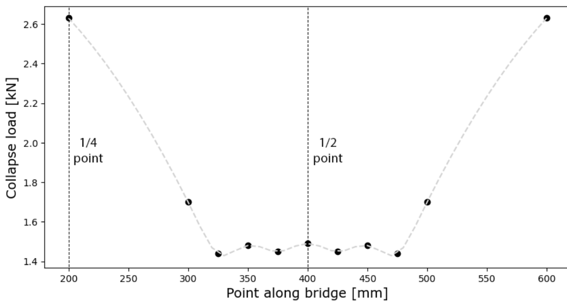
Figure 5.22: Circle: Collapse load for all the analysed loading positions
