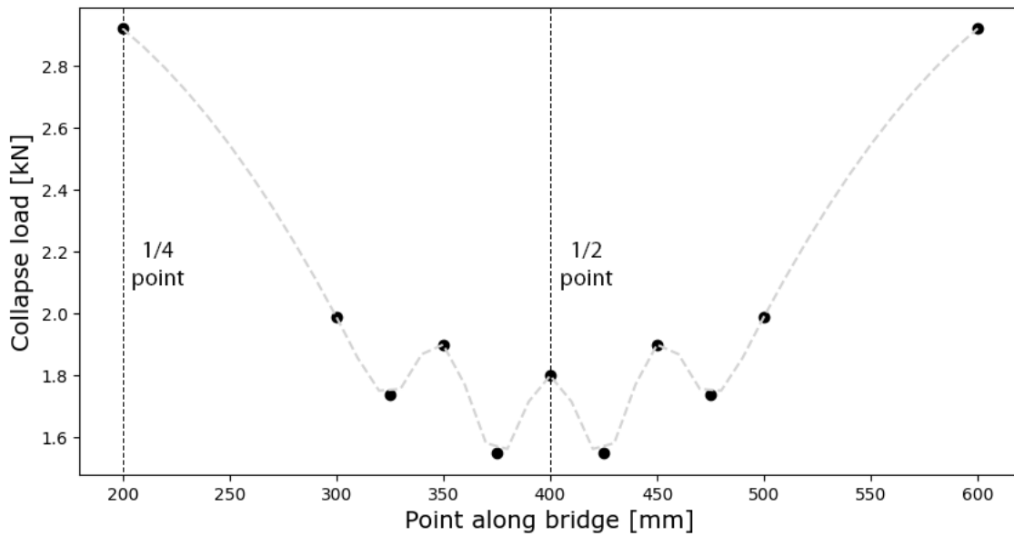
Figure 5.14: Catenary: Collapse load for all the analysed loading positions
