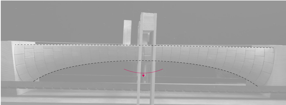
Figure 5.11: Load test of catenary with the load placed at midpoint, collapse at 13.9 kilograms.
