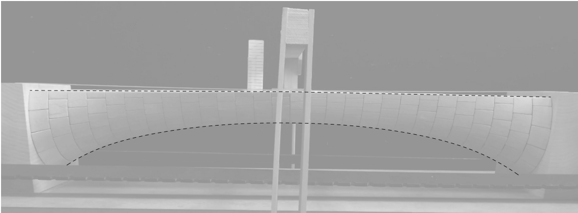
Figure 5.9: Load test of catenary with the load placed at midpoint, loaded with 1 kilogram.
