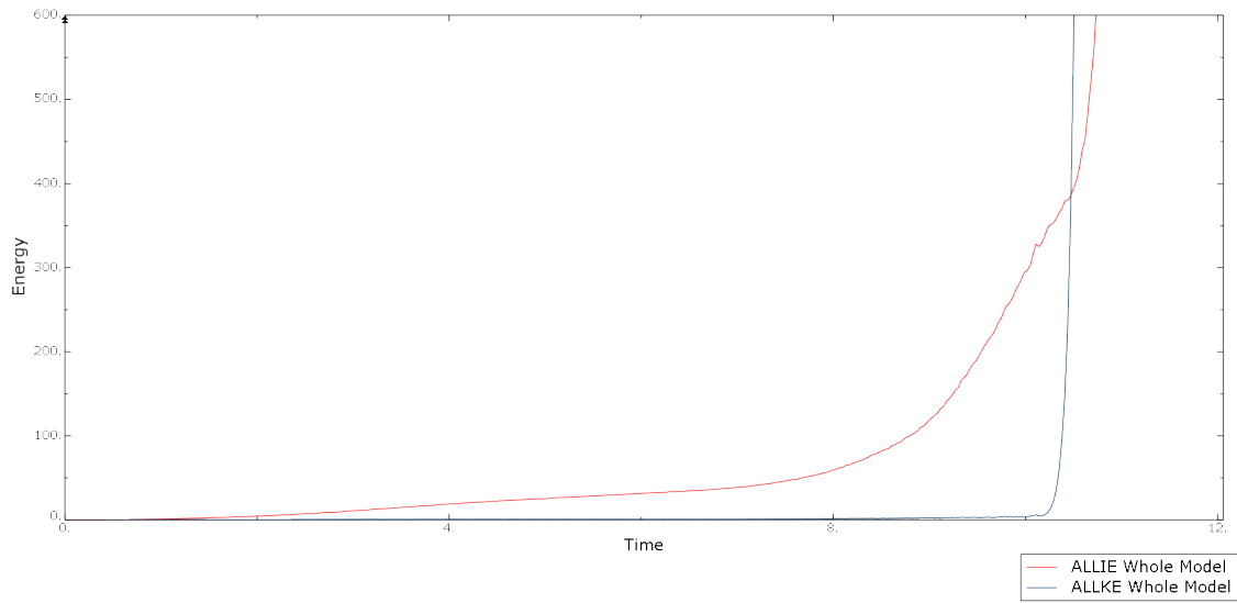
Figure 3.14: LC1: Internal (ALLIE) and kinetic (ALLKE) energy
