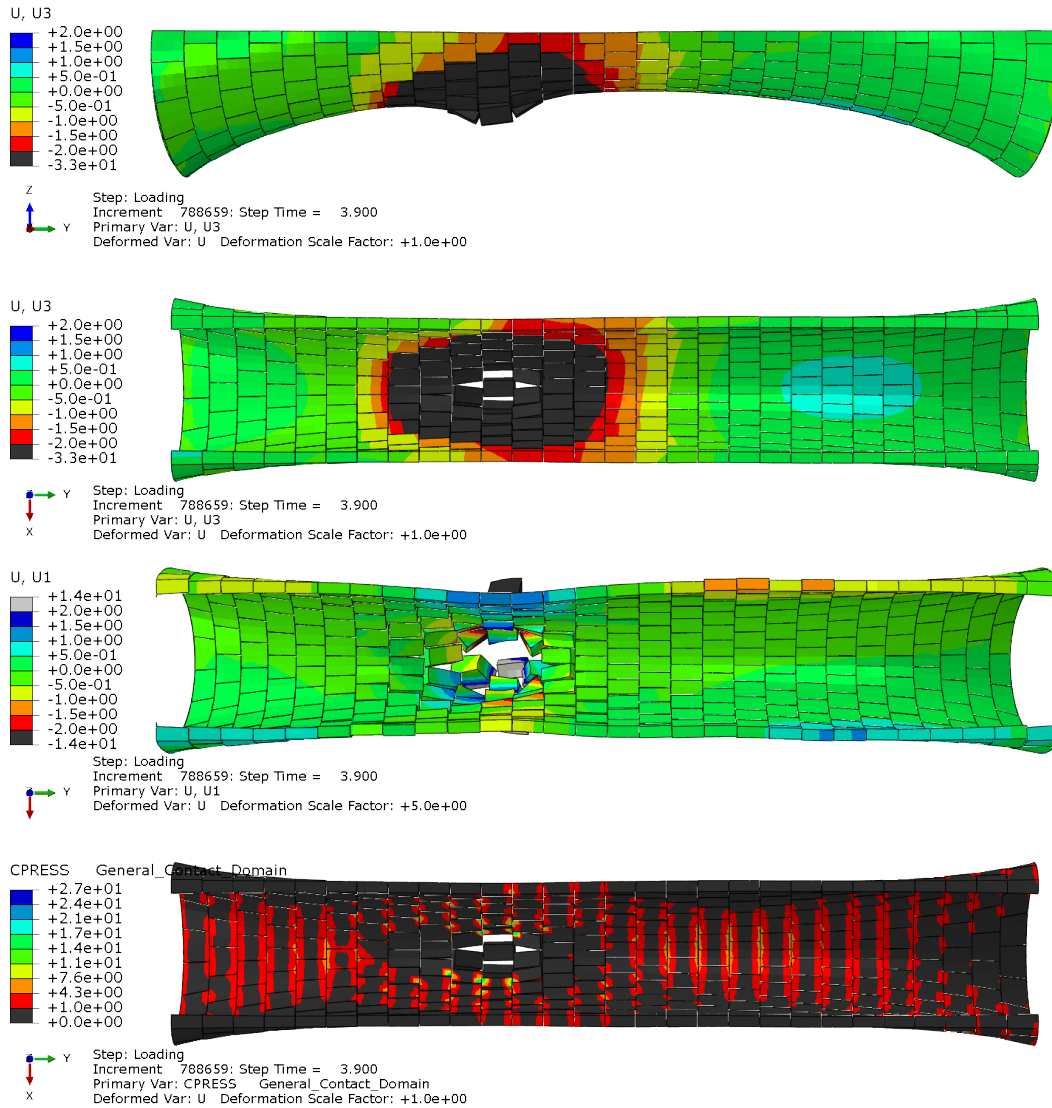
Figure A.8: Circle: Deformation figures for a load placed at y = 300 mm (a) Elevation: Vertical displacement. (b) Top view: Vertical displacement. (c) Top view: Horizontal displacement. (d) Top view: Contact pressure between voussoirs.
