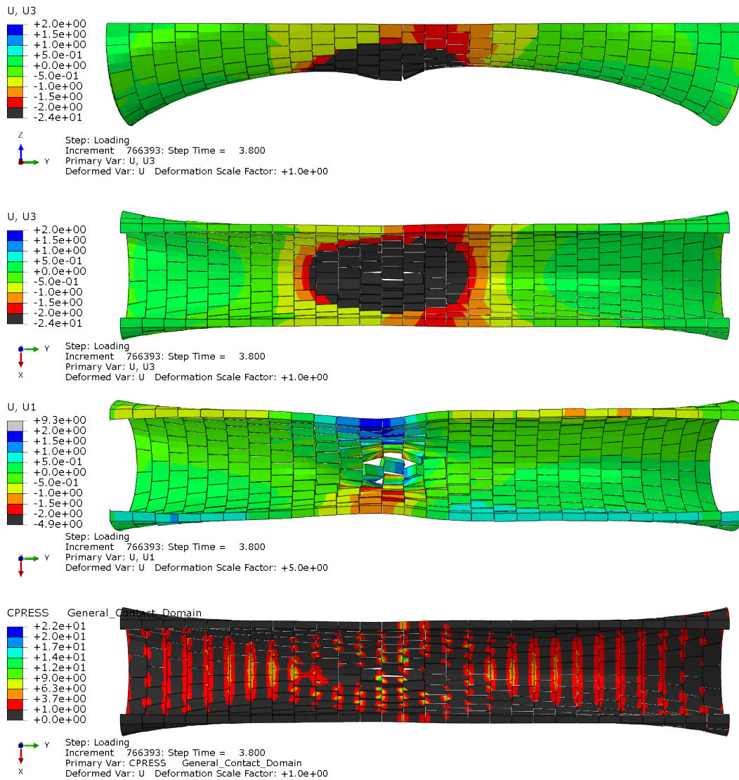
Figure A.6: Circle: Deformation figures for a load placed at y = 350 mm (a) Elevation: Vertical displacement. (b) Top view: Vertical displacement. (c) Top view: Horizontal displacement. (d) Top view: Contact pressure between voussoirs.
