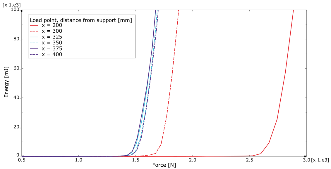
Figure 5.21: Circle: Force-Kinetic Energy graph for different loading positions defined from the support
