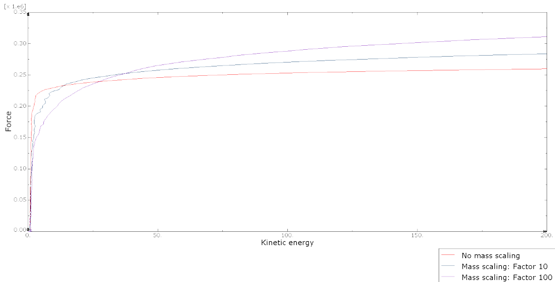
Figure 3.19: Effect of mass scaling on the kinetic energy
