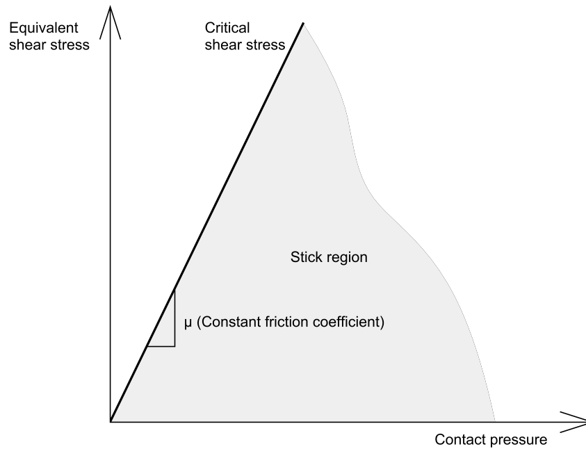
Figure 2.13: The Coulomb friction model redrawn from Abaqus User's Manual[1]
