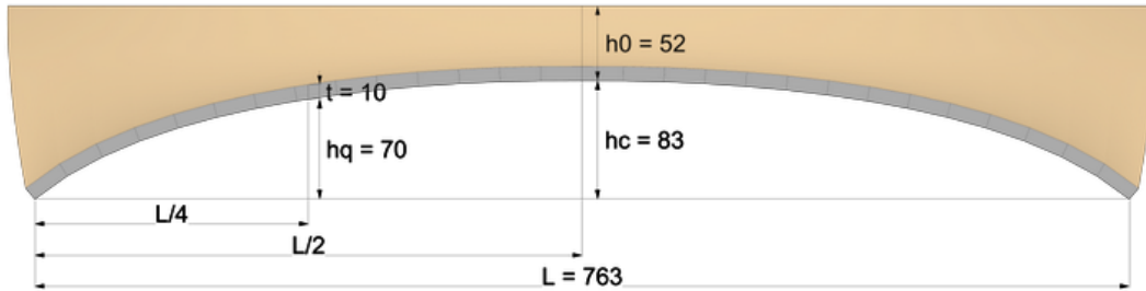
Figure 3.6: Dimensions of simplified catenary cross-section bridge for hand calculations [mm]. Width of bridge 138 mm.
