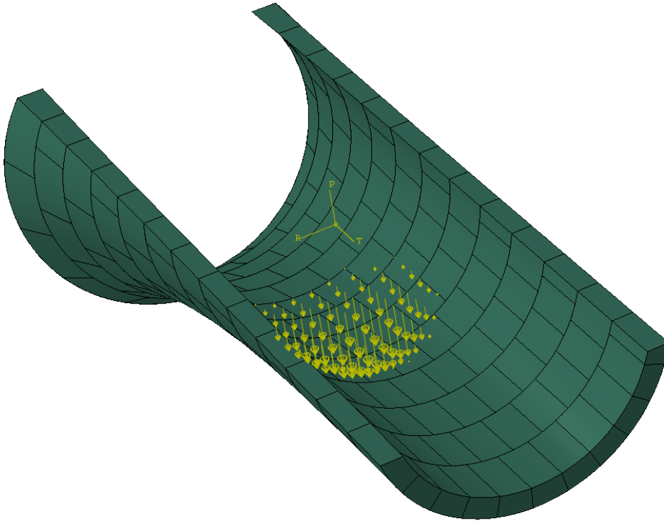
Figure 4.8: Load dispersion model in Abaqus for a concentrated force in the quarter point
