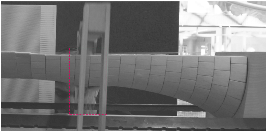
Figure 6.1: Initiation of collapse. Physical load test with load placed in 3/8 point.
