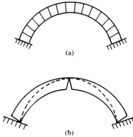
Figure 2.2: a) Statically indeterminate arch. b) Statically determinate arch under self weight due to movement of the abutments [26]
