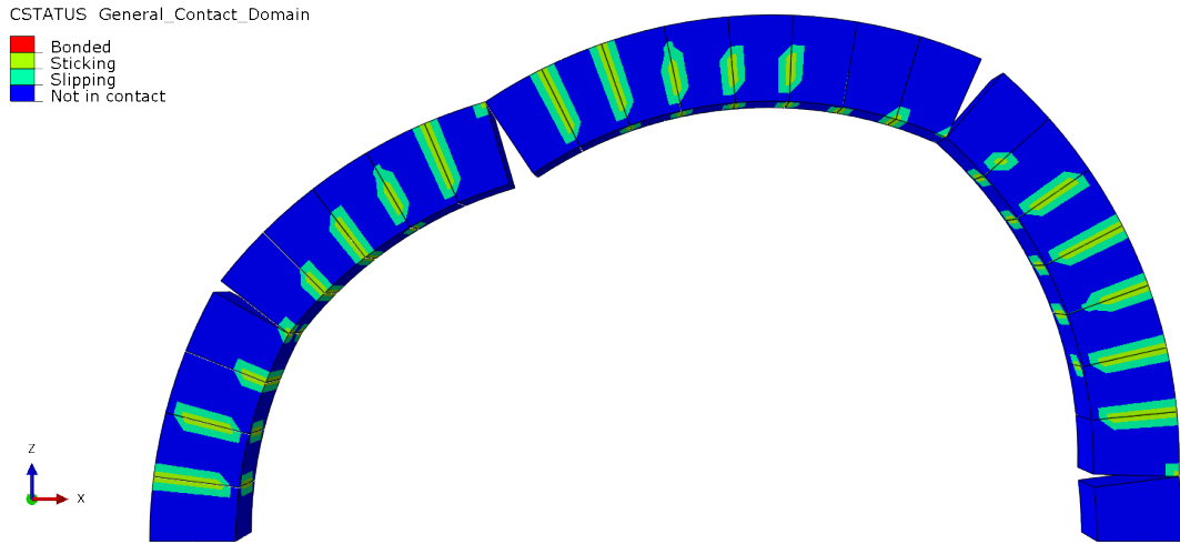
Figure 3.16: LC2: Collapse mode at t = 10.5s
