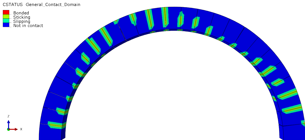
Figure 3.15: LC2: initialization of collapse: t = 9.9\text{s}
