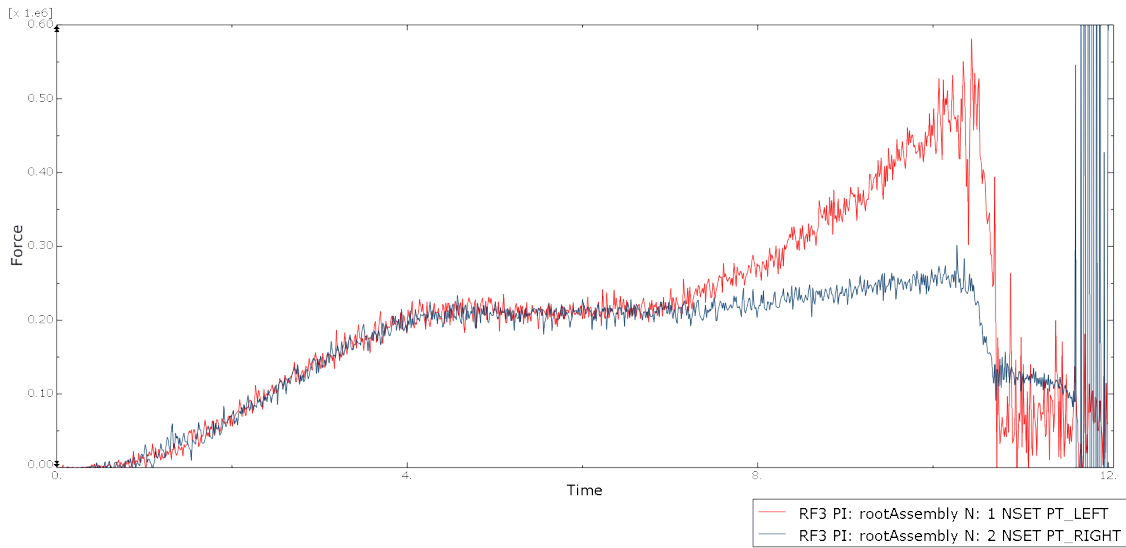
Figure 3.17: LC2: Vertical reaction forces in the left and right abutment
