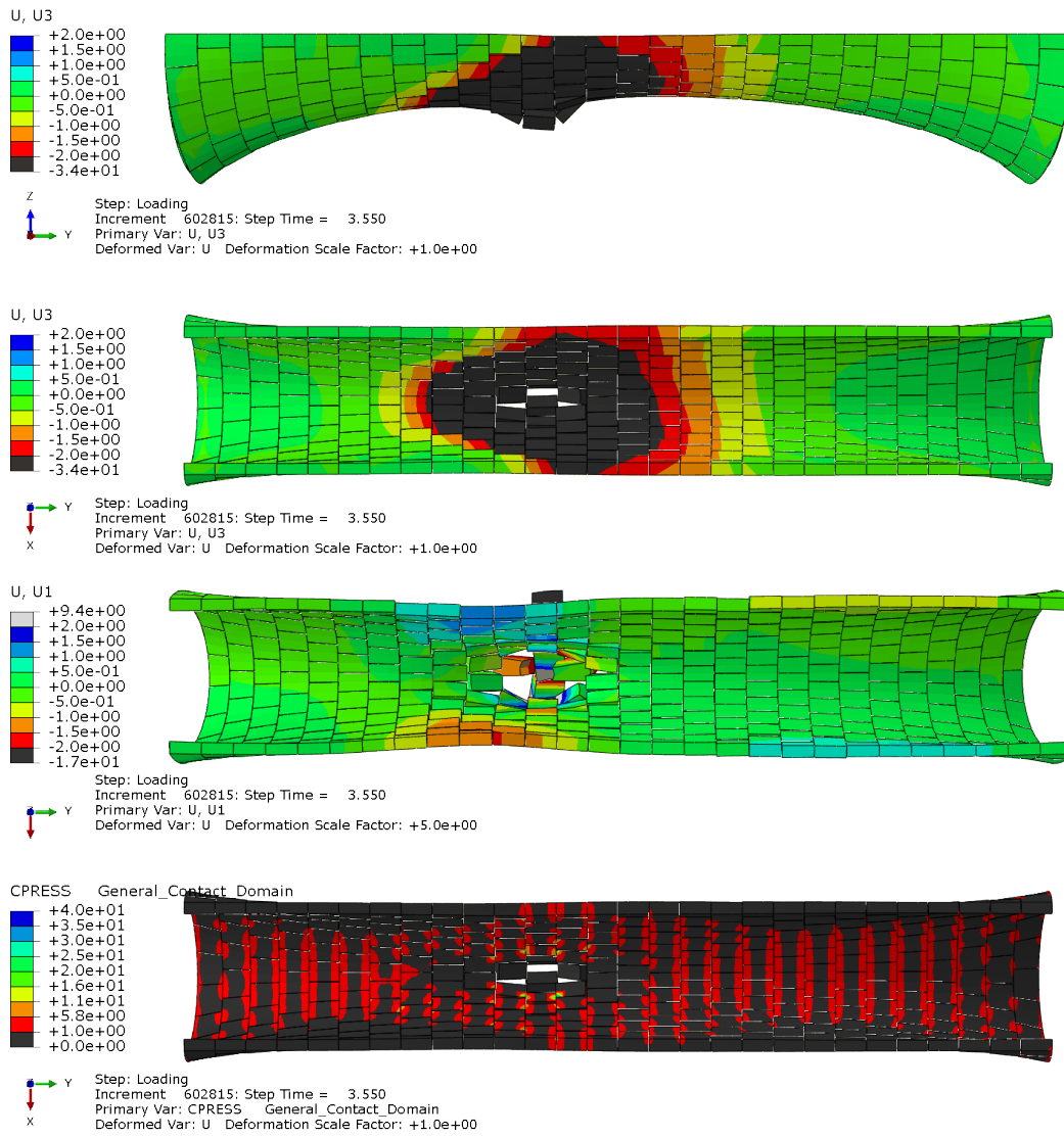
Figure A.3: Catenary: Deformation figures for a load placed at y = 325 mm (a) Elevation: Vertical displacement. (b) Top view: Vertical displacement. (c) Top view: Horizontal displacement. (d) Top view: Contact pressure between voussoirs.
