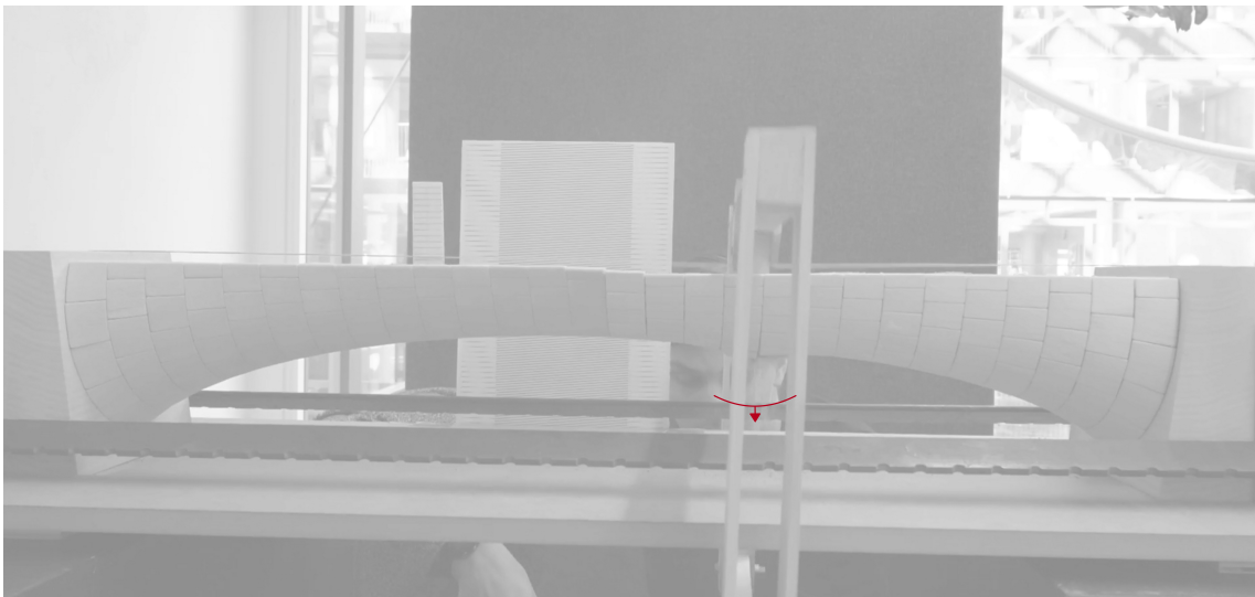
Figure 5.6: Load test of catenary with the load placed at 3/8 point, collapse at 22.9 kilograms.
