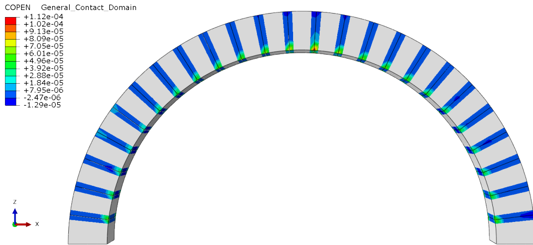
Figure 3.11: LC1: Contact openings after gravity load: t = 6\text{ s}
