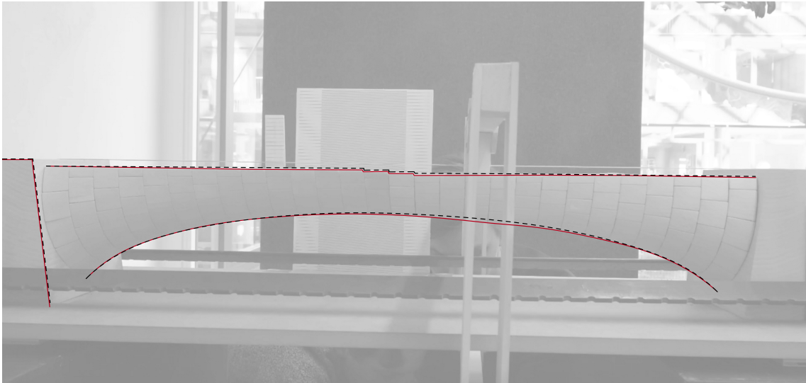
Figure 5.5: Load test of catenary with the load placed at the 3/8 point, deformation at approximately 20 kilograms. Red line: outlines of the bridge, black dashed: initial shape.
