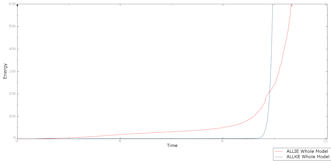
Figure 3.18: LC2: Internal (ALLIE) and kinetic (ALLKE) energy
