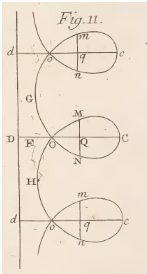
Figure 2.3: Euler's elastica [15], which has the same shape as an hydrostatic arch.
