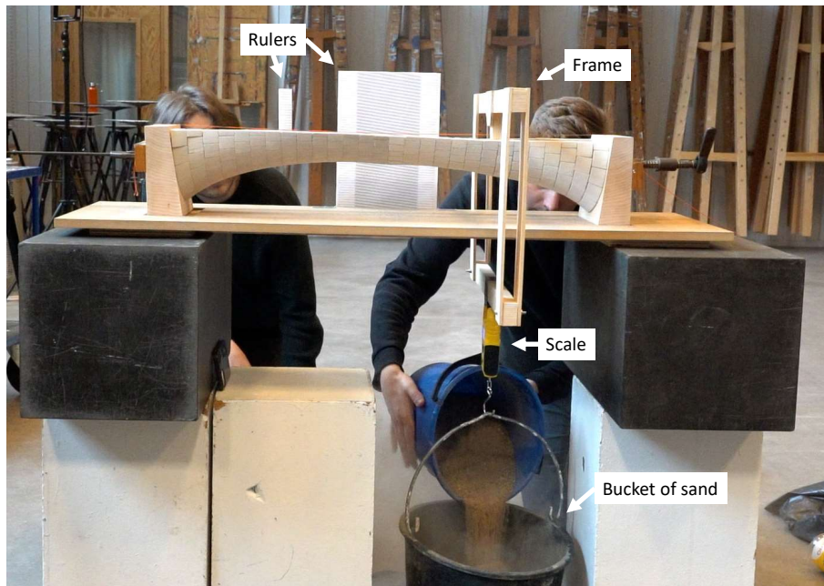
Figure 3.8: Setup for first physical load test.
