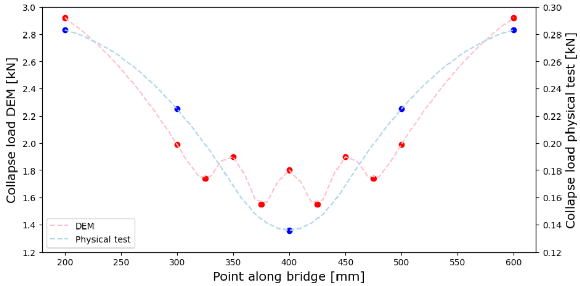
Figure 6.3: Comparison between Physical testing and Discrete Element Method of measured critical load
