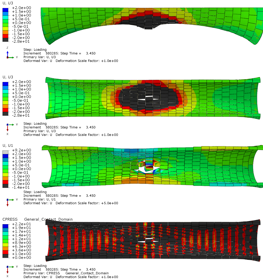
Figure A.1: Catenary: Deformation figures for a load placed at y = 375 mm. (a) Elevation: Vertical displacement. (b) Top view: Vertical displacement. (c) Top view: Horizontal displacement. (d) Top view: Contact pressure between voussoirs.
