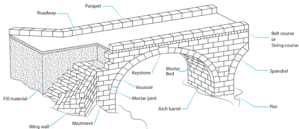
Figure 1.2: Typical stone arch bridge and terminology. Redrawn from Commonwealth of Pennsylvania [10].
