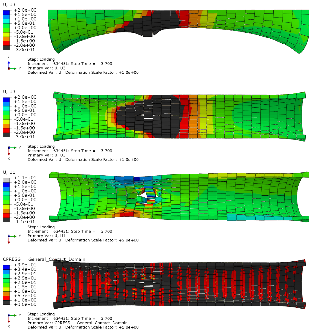
Figure A.4: Catenary: Deformation figures for a load placed at y = 300 mm (a) Elevation: Vertical displacement. (b) Top view: Vertical displacement. (c) Top view: Horizontal displacement. (d) Top view: Contact pressure between voussoirs.
