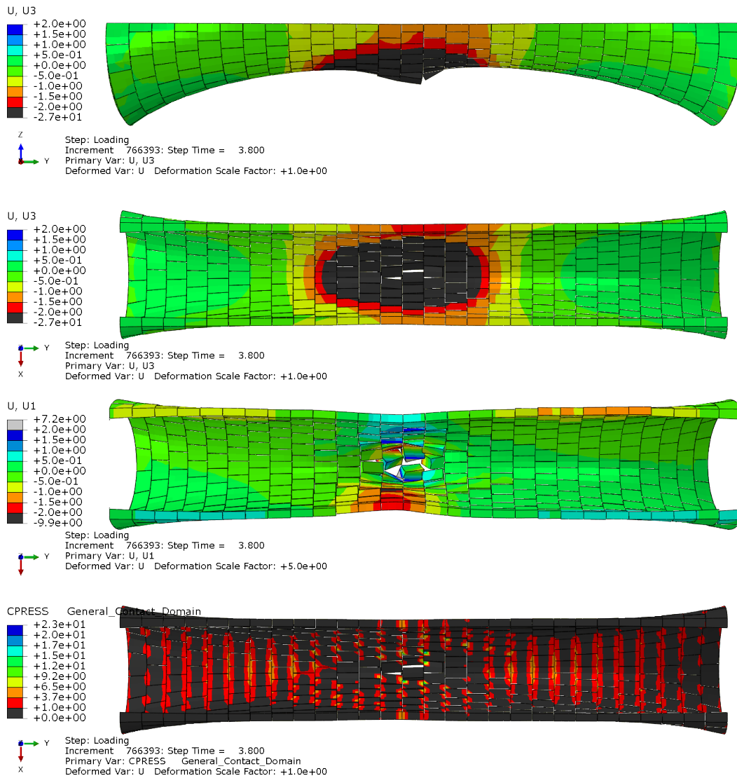
Figure A.5: Circle: Deformation figures for a load placed at y = 375 mm (a) Elevation: Vertical displacement. (b) Top view: Vertical displacement. (c) Top view: Horizontal displacement. (d) Top view: Contact pressure between voussoirs.
