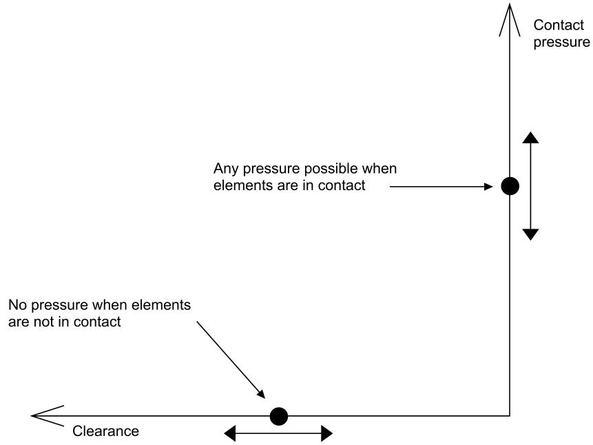
Figure 2.12: Default pressure-overclosure relationship redrawn from Abaqus User's Manual[1]
