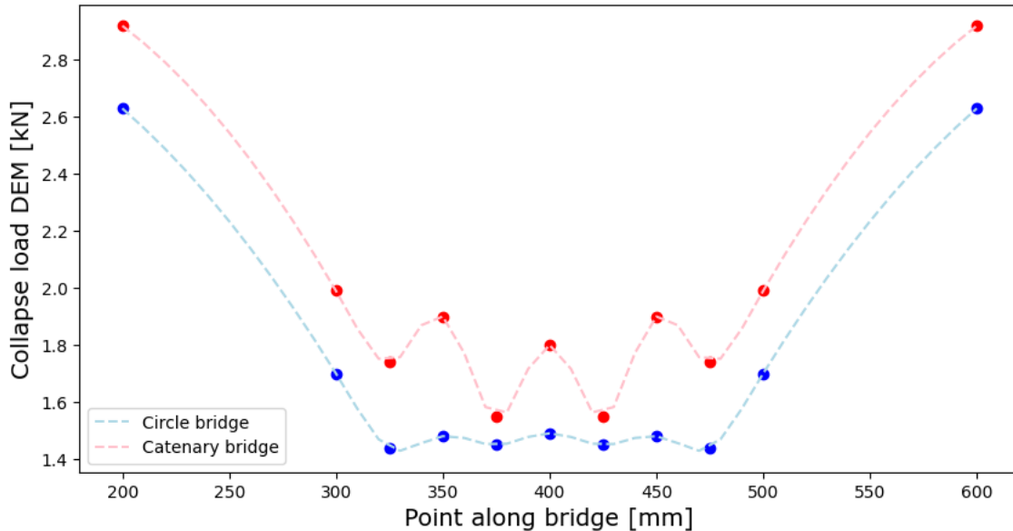
Figure 6.2: Collapse load from DE-analysis for the catenary and circle bridge
