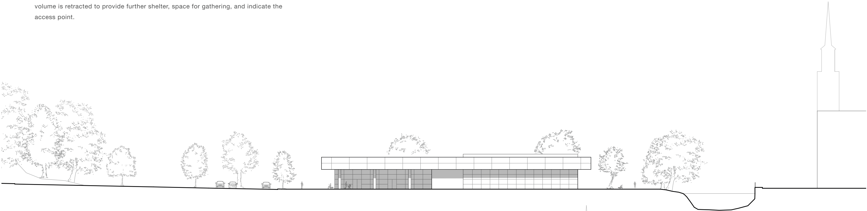
Elevation south 1:500
