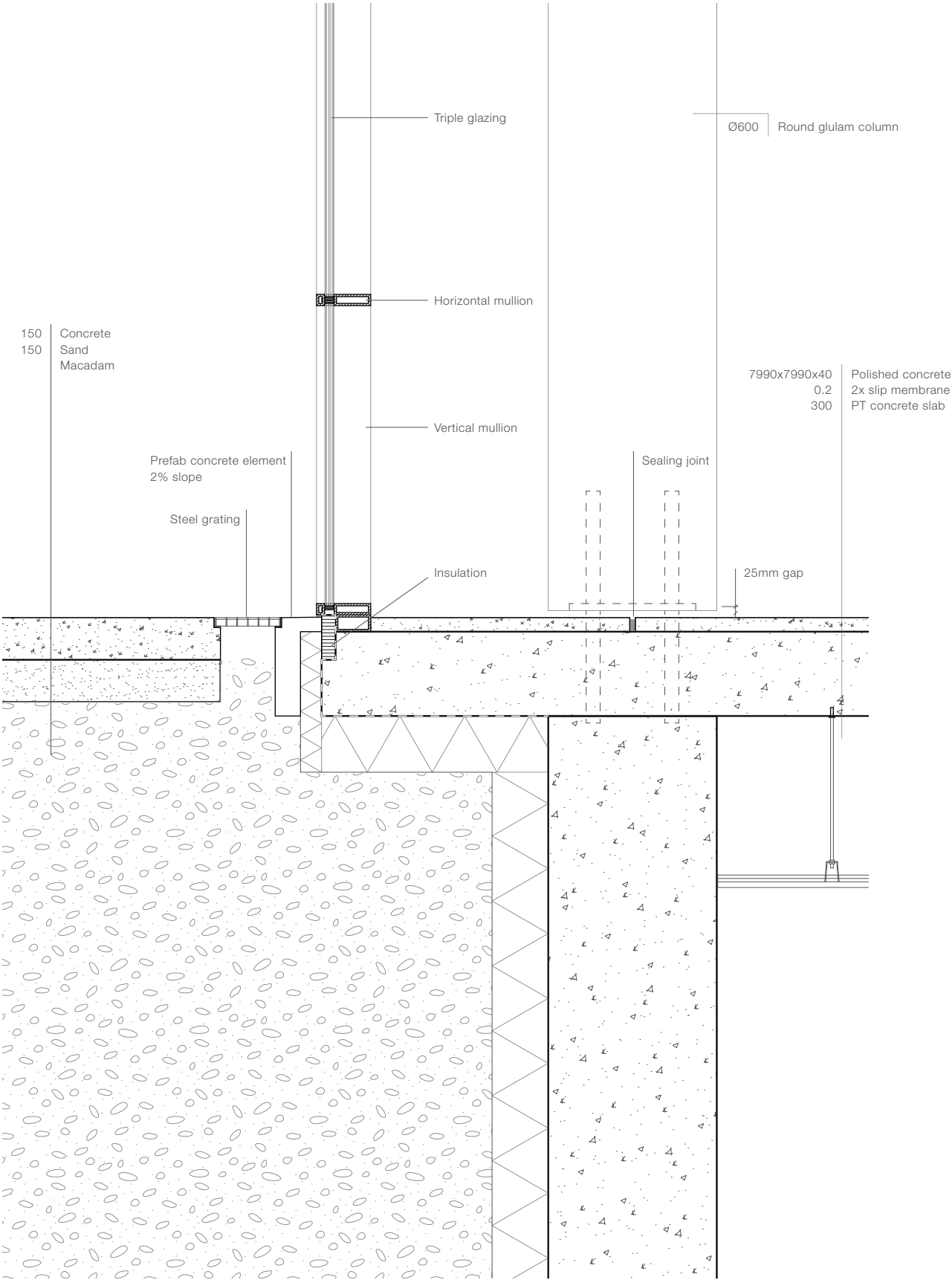
Detail section C 1:20
