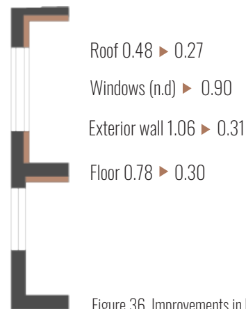
Figure 36. Improvements in U-value
