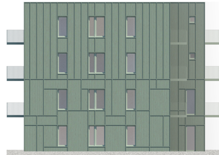
West Facade, Scale 1:200
