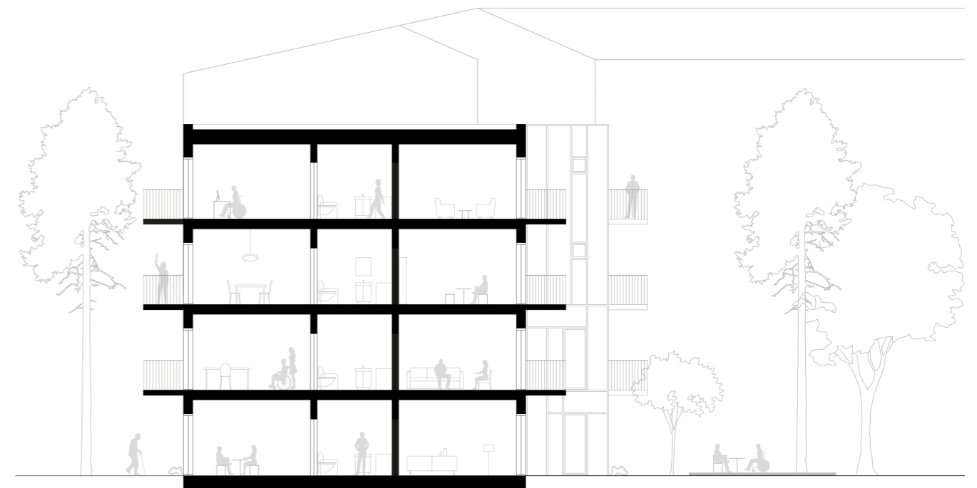
Section, Scale 1:200
