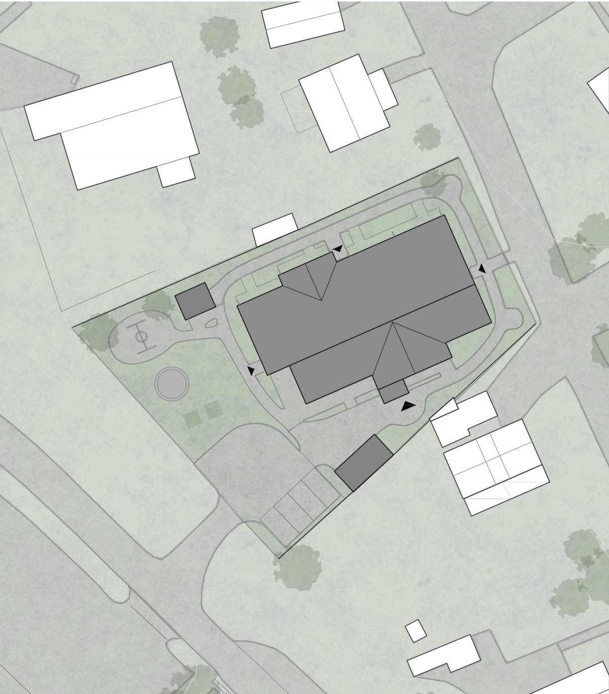
Figure 56. Site plan scale 1:500
