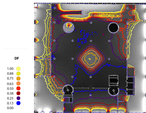
Figure 45: Daylight analysis - Ground floor plan
