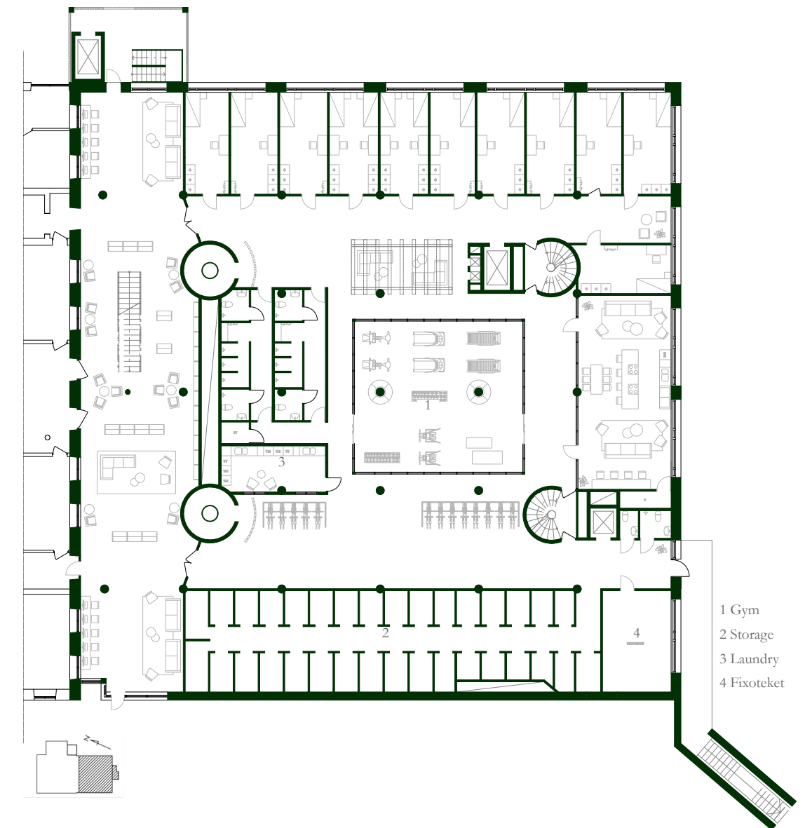
Underground floor, scale 1:300
