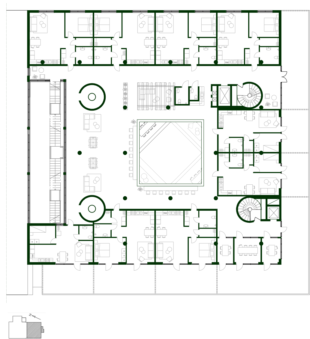
Second floor, scale 1:300
