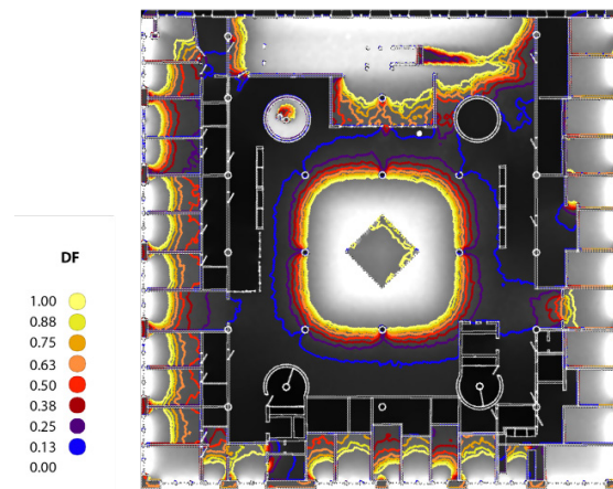
Figure 44: Daylight analysis - First floor plan
