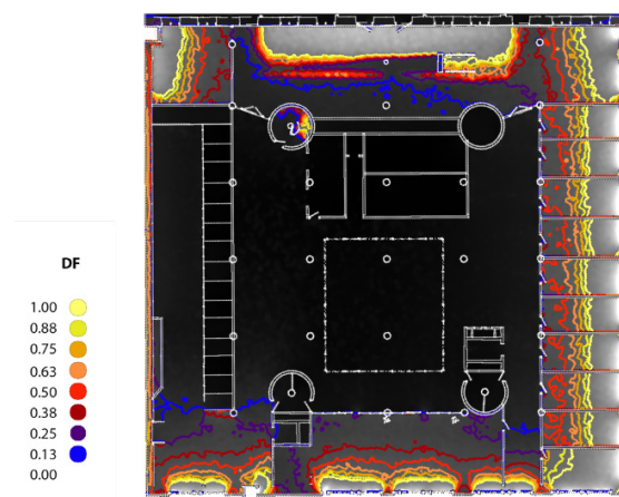
Figure 46: Daylight analysis - underground floor plan
