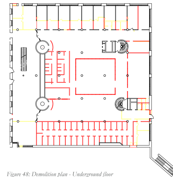
Figure 48: Demolition plan - Underground floor
