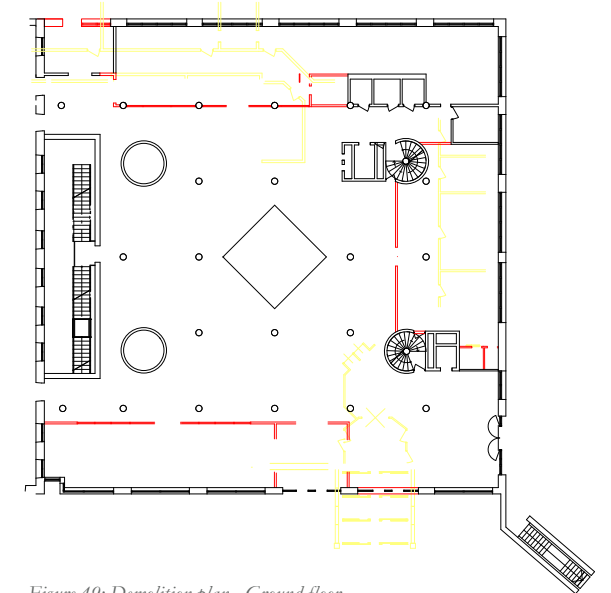
Figure 49: Demolition plan - Ground floor
