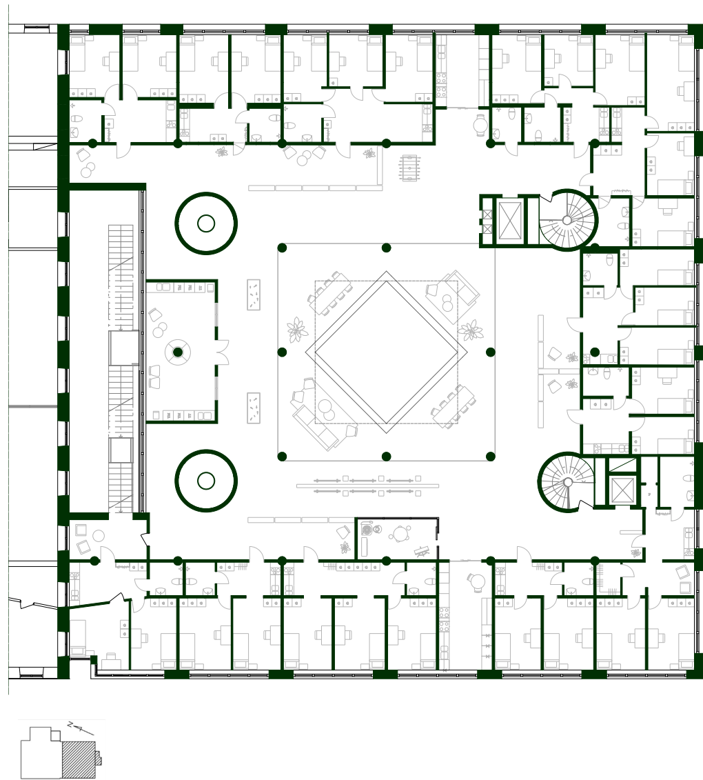
First floor, scale 1:300
