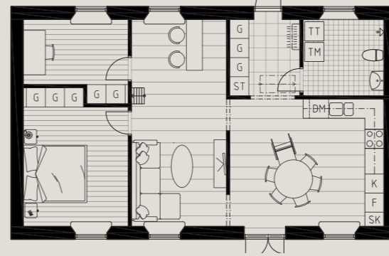
Figure 100-101. Furnishability in the dwellings.
