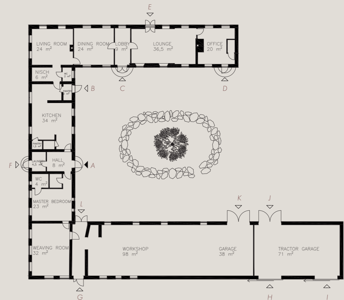
Figure 56. Floorplan with all entrances marked.
