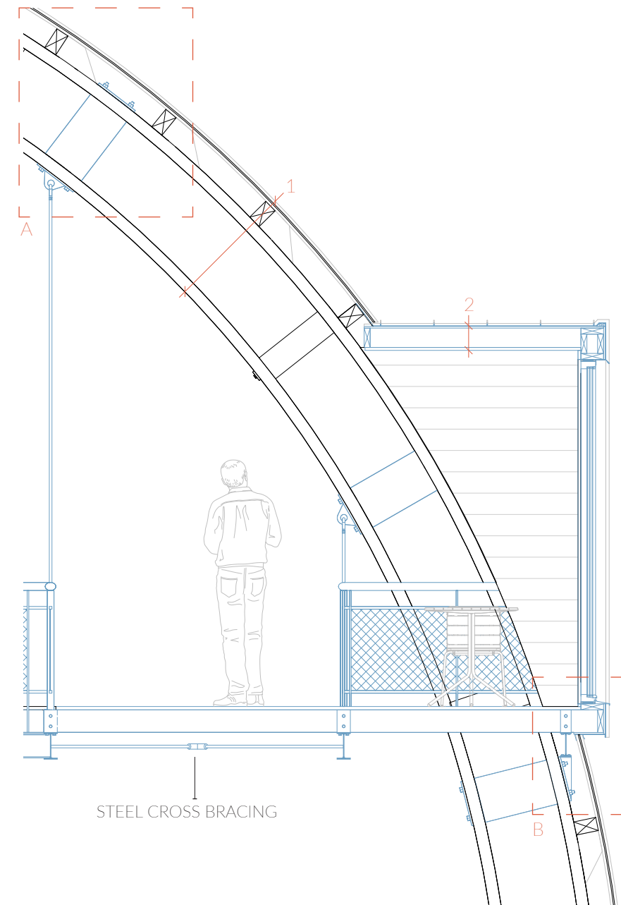
Fig. 108 Dormer detail 1:40
