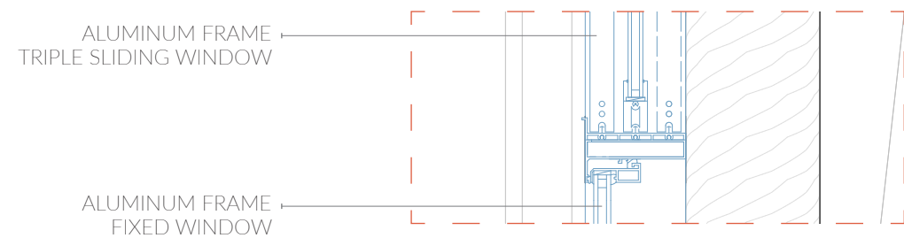
Fig. 110 Gable callout B 1:10
