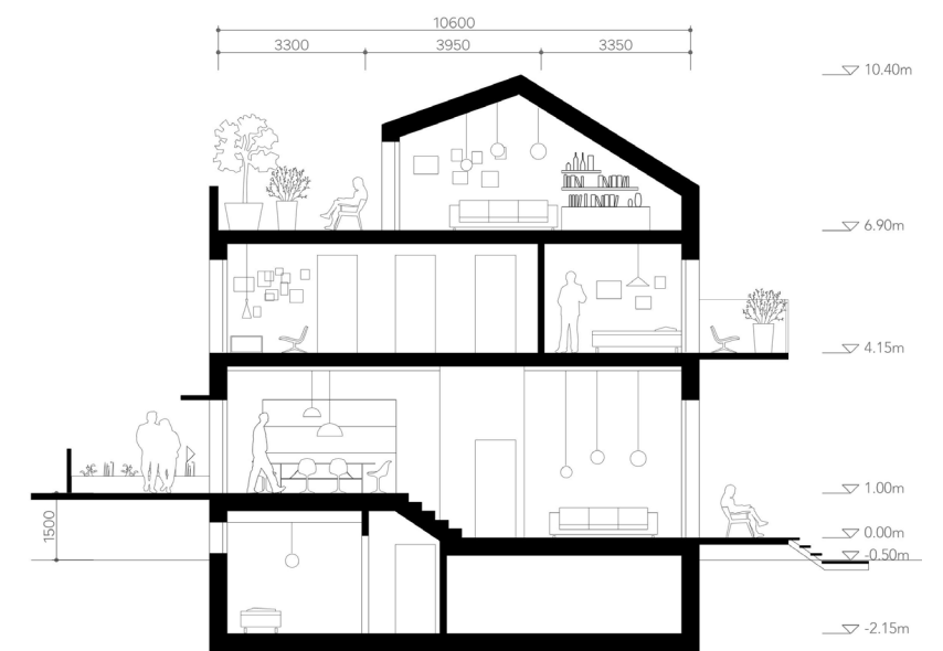
SECTION 1:200
