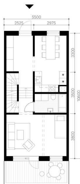
GF PLAN 1:200
