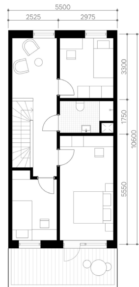
1F PLAN 1:200
