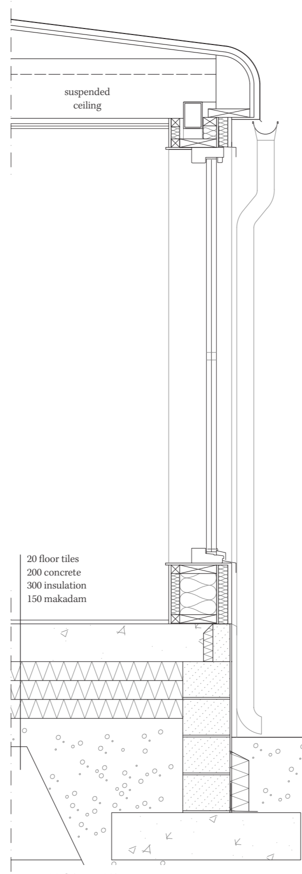
02. VERTICAL DETAIL
