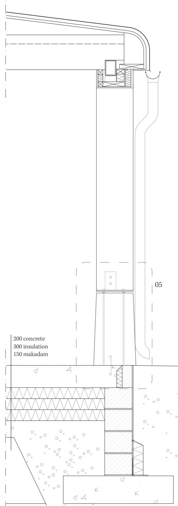
04. VERTICAL DETAIL
