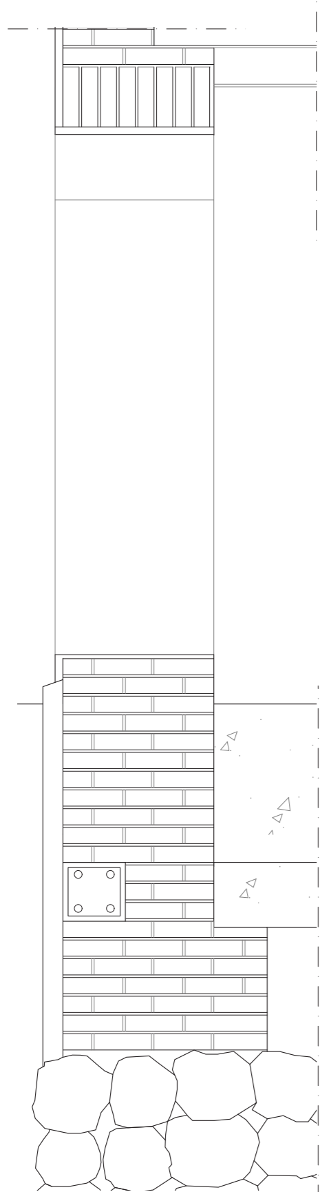
03. VERTICAL DETAIL
