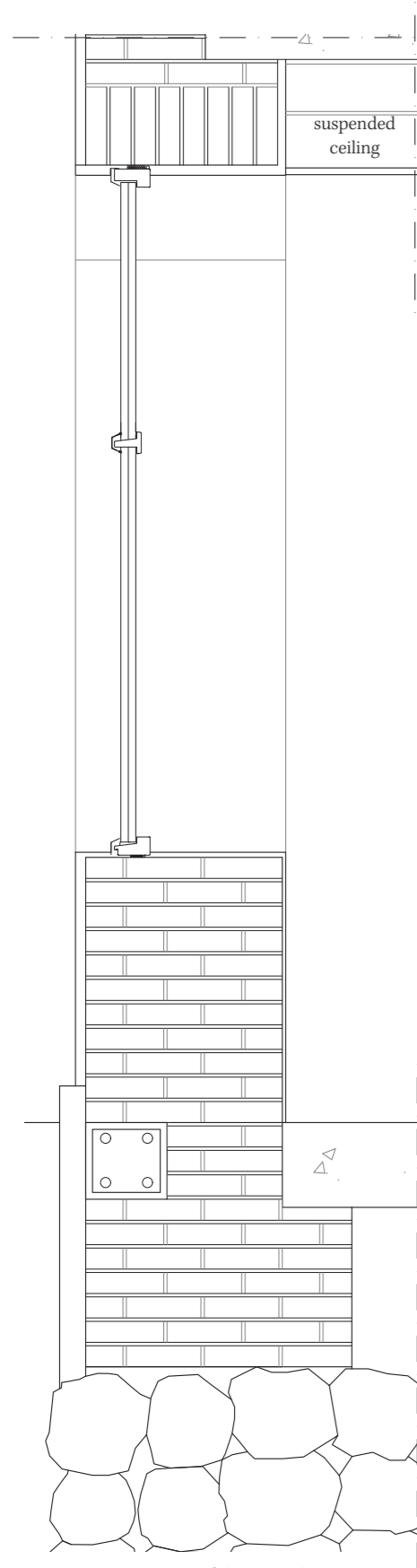
01. VERTICAL DETAIL
