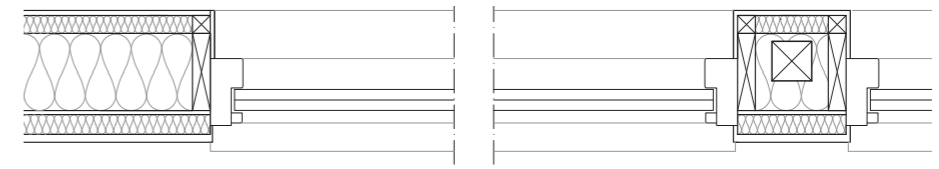
02. HORIZONTAL DETAIL
