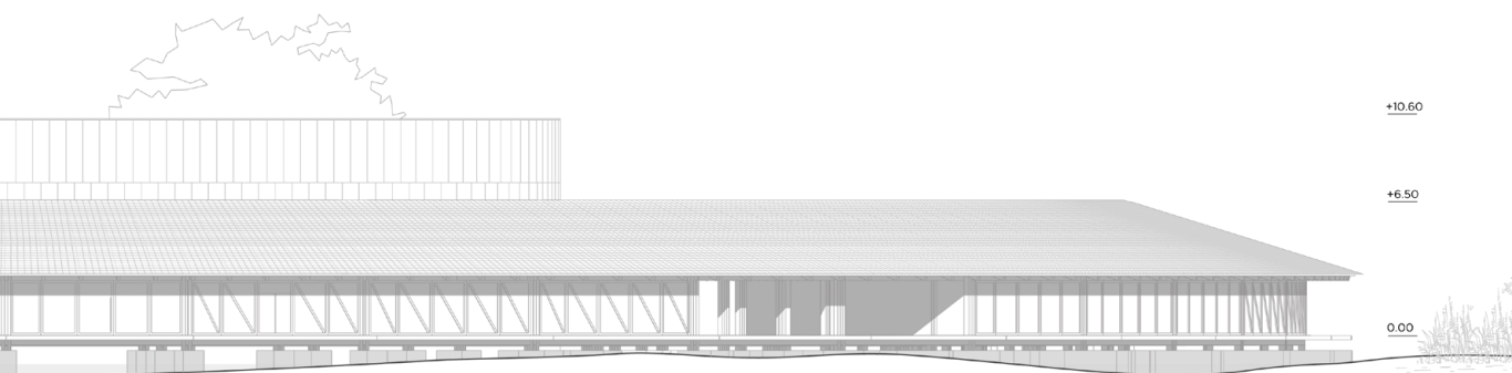
WEST ELEVATION
