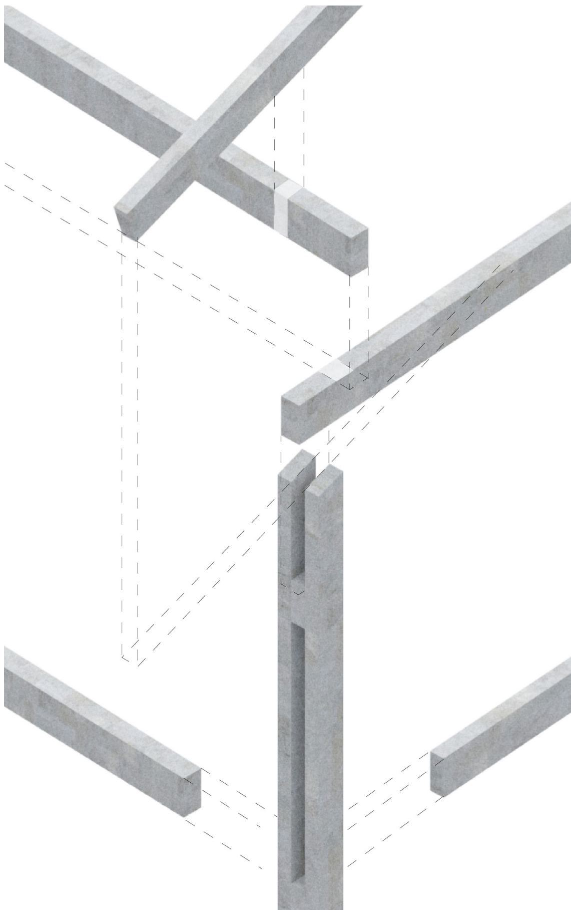
Fig. 40. Wood construction - assembly diagram
